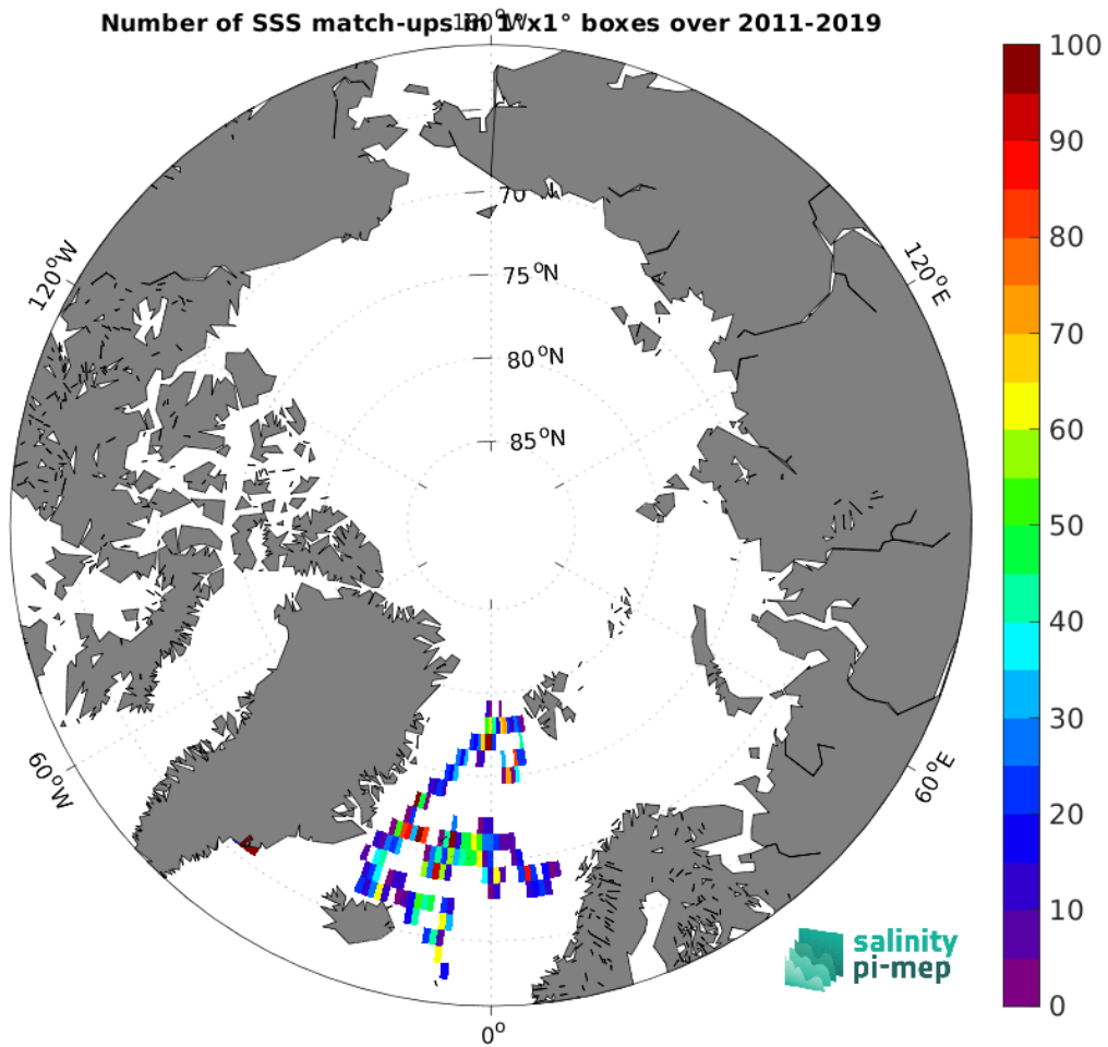
Figure 4: Number of SSS match-ups between Surface drifters SSS and the SMAP SSS L4 OI v3 - Daily (ESR) SSS product for the Arctic Ocean Pi-MEP region over 1^\circ \times 1^\circ boxes and for the full satellite product period.
