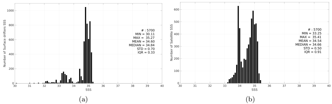
Figure 3: Histograms of SSS from Surface drifters (a) and SMAP SSS L4 OI v3 - Daily (ESR) (b) considering all match-up pairs per bins of 0.1 over the Arctic Ocean Pi-MEP region and for the full satellite product period.
