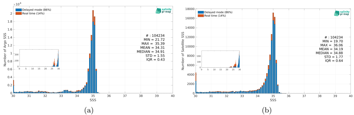
Figure 3: Histograms of SSS from Argo (a) and SMAP SSS L4 OI v3 - Daily (ESR) (b) considering all match-up pairs per bins of 0.1 over the Arctic Ocean Pi-MEP region and for the full satellite product period.
