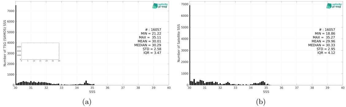
Figure 2: Histograms of SSS from TSG (SAMOS) (a) and SMAP SSS L4 OI v2 - 7 Days (ESR) (b) considering all match-up pairs per bins of 0.1 over the Arctic Ocean Pi-MEP region and for the full satellite product period.
