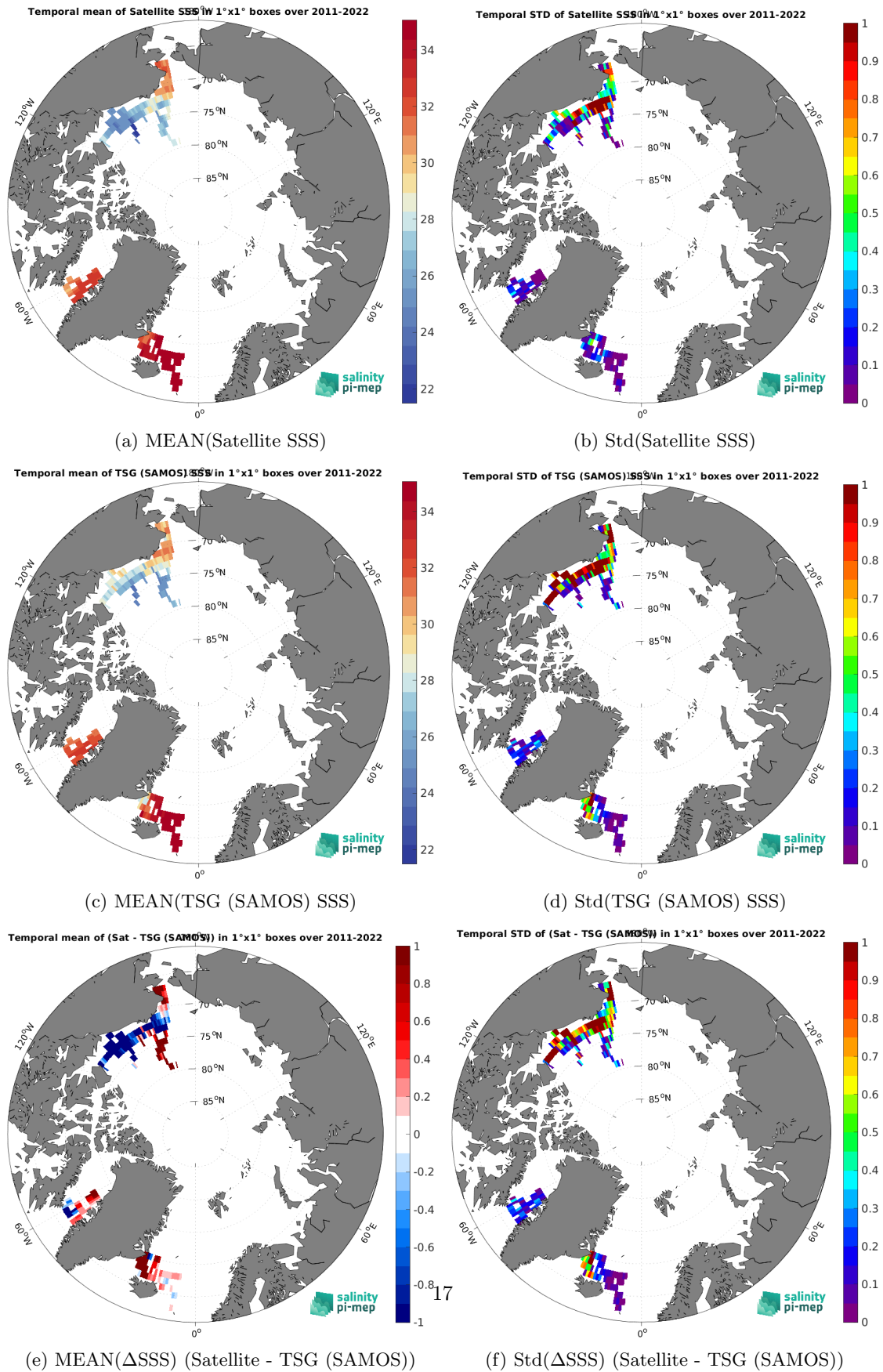
Figure 6: Temporal mean (left) and Std (right) of SSS from SMAP SSS L4 OI v2 - 7 Days (ESR) (top), TSG (SAMOS) (middle), and of \Delta SSS (Satellite - TSG (SAMOS)). Only match-up pairs are used to generate these maps.
