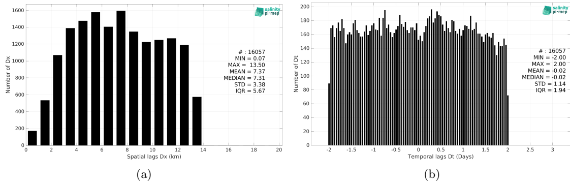
Figure 5: Histograms of the spatial (a) and temporal (b) lags between the location/time of the TSG (SAMOS) measurement and the date of the corresponding SMAP SSS L4 OI v2 - 7 Days (ESR) SSS pixel.
