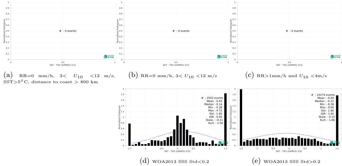
Figure 13: Normalized histogram of \Delta SSS (SMAP SSS L4 OI v2 - 7 Days (ESR) - TSG (SAMOS)) for 5 different subdatasets corresponding to: RR=0 mm/h, 3 < U_{10} < 12 m/s, SST>5°C, distance to coast > 800 km (a), RR=0 mm/h, 3 < U_{10} < 12 m/s (b), RR>1mm/h and U_{10} < 4 m/s (c), WOA2013 SSS Std<0.2 (d), WOA2013 SSS Std>0.2 (e).
