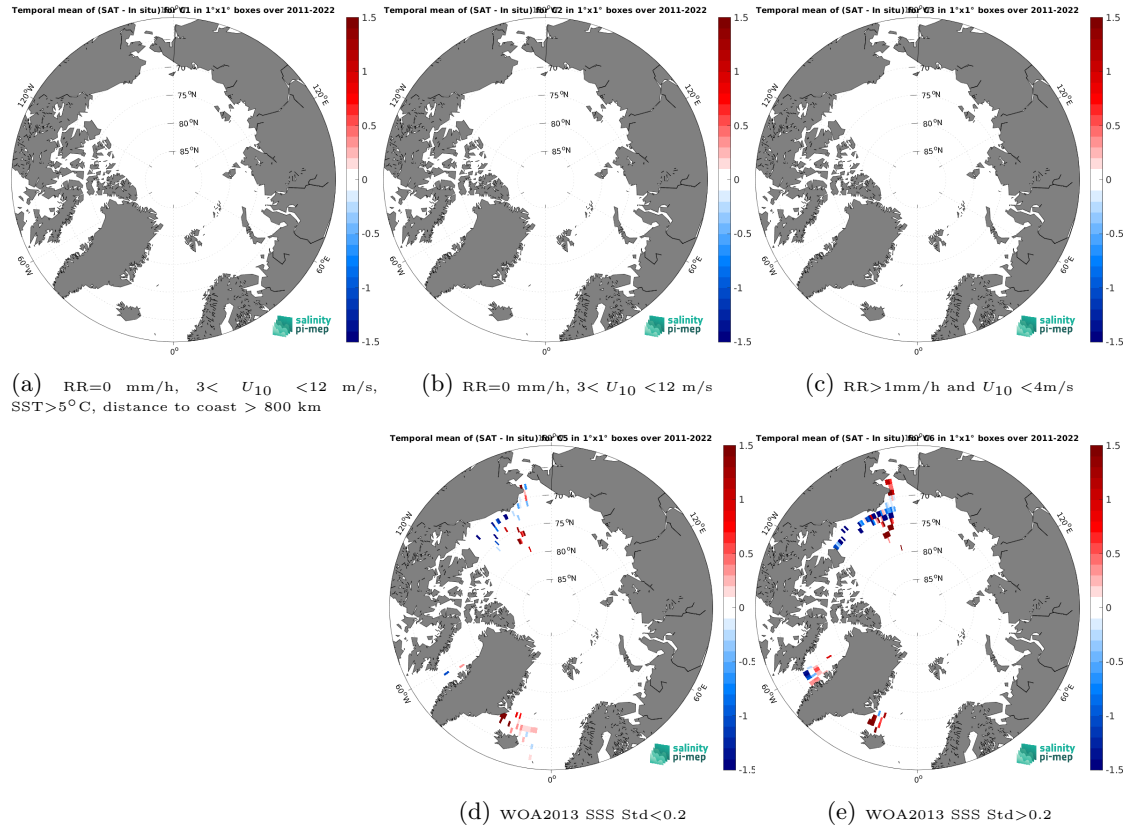
Figure 12: Temporal mean gridded over spatial boxes of size 1^{\circ}\times 1^{\circ} of \Delta\text{SSS} (SMAP SSS L4 OI v2 - 7 Days (ESR) - TSG (SAMOS)) for 5 different subdatasets corresponding to:RR=0 mm/h, 3 < U_{10} < 12 m/s, SST > 5^{\circ}\text{C} , distance to coast > 800 km (a), RR=0 mm/h, 3 < U_{10} < 12 m/s (b), RR > 1 mm/h and U_{10} < 4 m/s (c), WOA2013 SSS Std < 0.2 (d), WOA2013 SSS Std > 0.2 (e).
