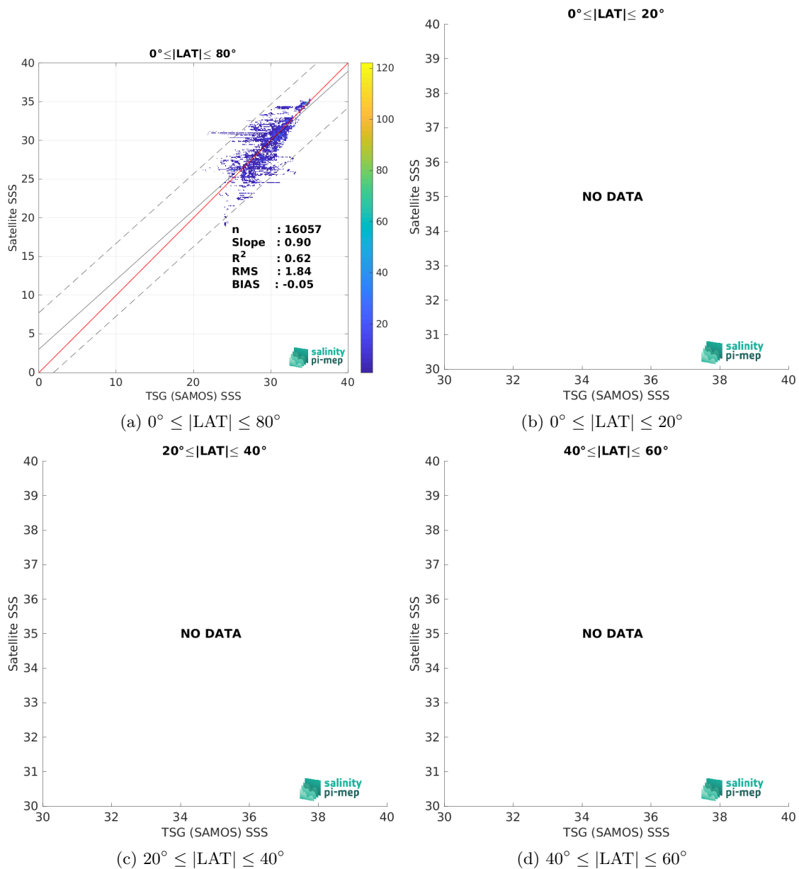
Figure 9: Contour maps of the concentration of SMAP SSS L4 OI v2 - 7 Days (ESR) SSS (y-axis) versus TSG (SAMOS) SSS (x-axis) at match-up pairs for different latitude bands. For each plot, the red line shows x=y . The black thin and dashed lines indicate a linear fit through the data cloud and the \pm 95\% confidence levels, respectively. The number match-up pairs n , the slope and R^2 coefficient of the linear fit, the root mean square (RMS) and the mean bias between satellite and in situ data are indicated for each latitude band in each plots.
