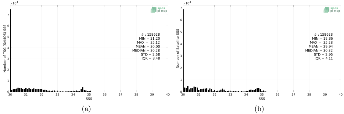
Figure 2: Histograms of SSS from TSG (SAMOS) (a) and SMAP SSS L4 OI v2 - 7 Days (ESR) (b) considering all match-up pairs per bins of 0.1 over the Arctic Ocean Pi-MEP region and for the full satellite product period.
