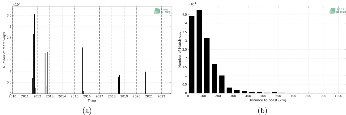
Figure 1: Number of match-ups between TSG (SAMOS) and SMAP SSS L4 OI v2 - 7 Days (ESR) SSS as a function of time (a) and as function of the distance to coast (b) over the Arctic Ocean Pi-MEP region and for the full satellite product period.
