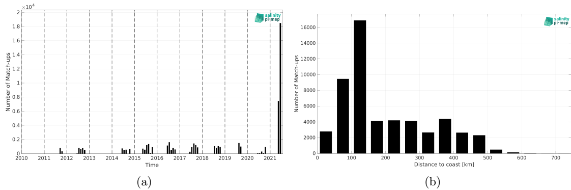
Figure 1: Number of match-ups between TSG (Polarstern) and SMAP SSS L4 OI v2 - 7 Days (ESR) SSS as a function of time (a) and as function of the distance to coast (b) over the Arctic Ocean Pi-MEP region and for the full satellite product period.
