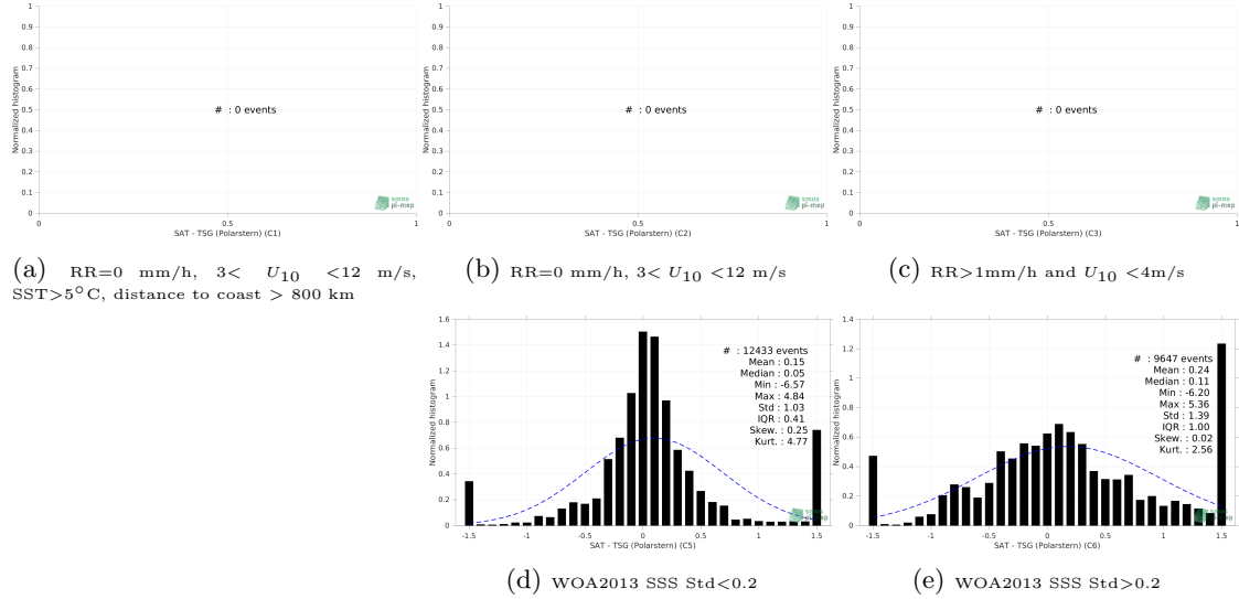
Figure 13: Normalized histogram of \Delta SSS (SMAP SSS L4 OI v2 - 7 Days (ESR) - TSG (Polarstern)) for 5 different subdatasets corresponding to: RR=0 mm/h, 3 < U_{10} < 12 m/s, SST>5°C, distance to coast > 800 km (a), RR=0 mm/h, 3 < U_{10} < 12 m/s (b), RR>1mm/h and U_{10} < 4 m/s (c), WOA2013 SSS Std<0.2 (d), WOA2013 SSS Std>0.2 (e).
