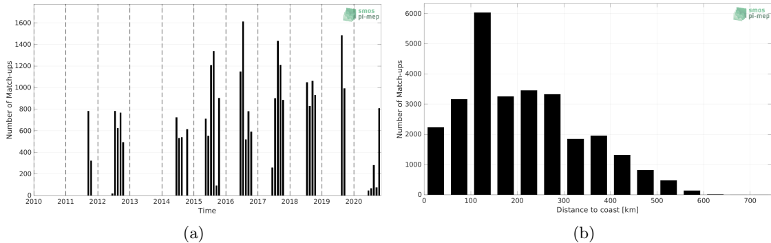
Figure 1: Number of match-ups between TSG (Polarstern) and SMAP SSS L4 OI v2 - 7 Days (ESR) SSS as a function of time (a) and as function of the distance to coast (b) over the Arctic Ocean Pi-MEP region and for the full satellite product period.
