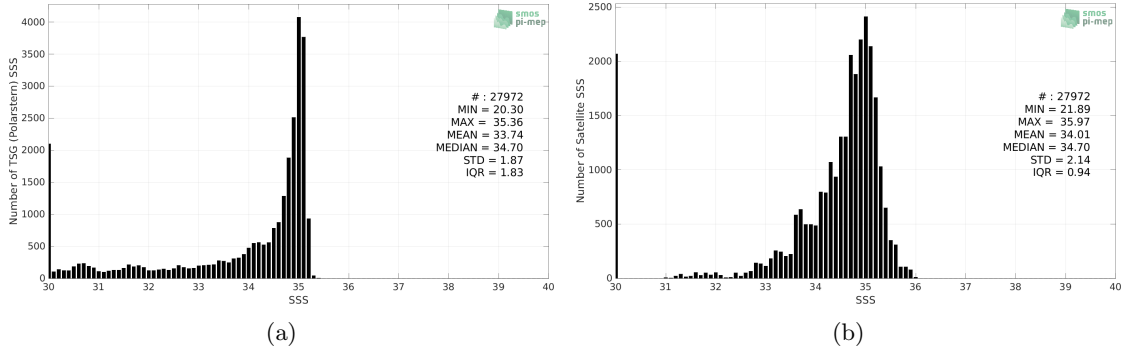
Figure 2: Histograms of SSS from TSG (Polarstern) (a) and SMAP SSS L4 OI v2 - 7 Days (ESR) (b) considering all match-up pairs per bins of 0.1 over the Arctic Ocean Pi-MEP region and for the full satellite product period.
