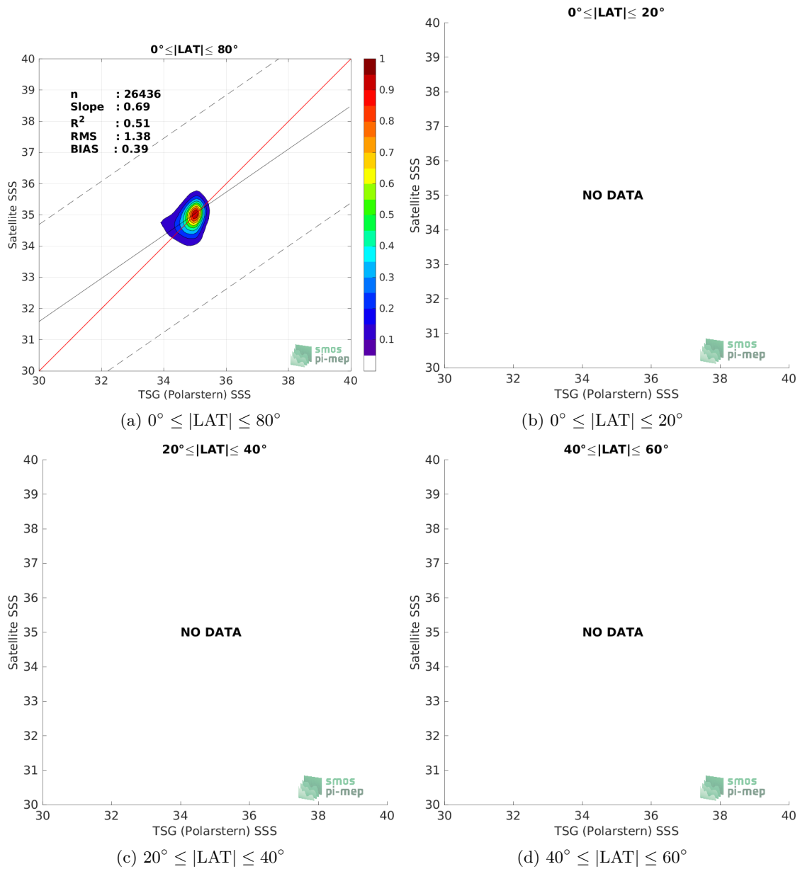
Figure 9: Contour maps of the concentration of SMAP SSS L4 OI v2 - 7 Days (ESR) SSS (y-axis) versus TSG (Polarstern) SSS (x-axis) at match-up pairs for different latitude bands. For each plot, the red line shows x=y . The black thin and dashed lines indicate a linear fit through the data cloud and the \pm 95\% confidence levels, respectively. The number match-up pairs n , the slope and R^2 coefficient of the linear fit, the root mean square (RMS) and the mean bias between satellite and in situ data are indicated for each latitude band in each plots.
