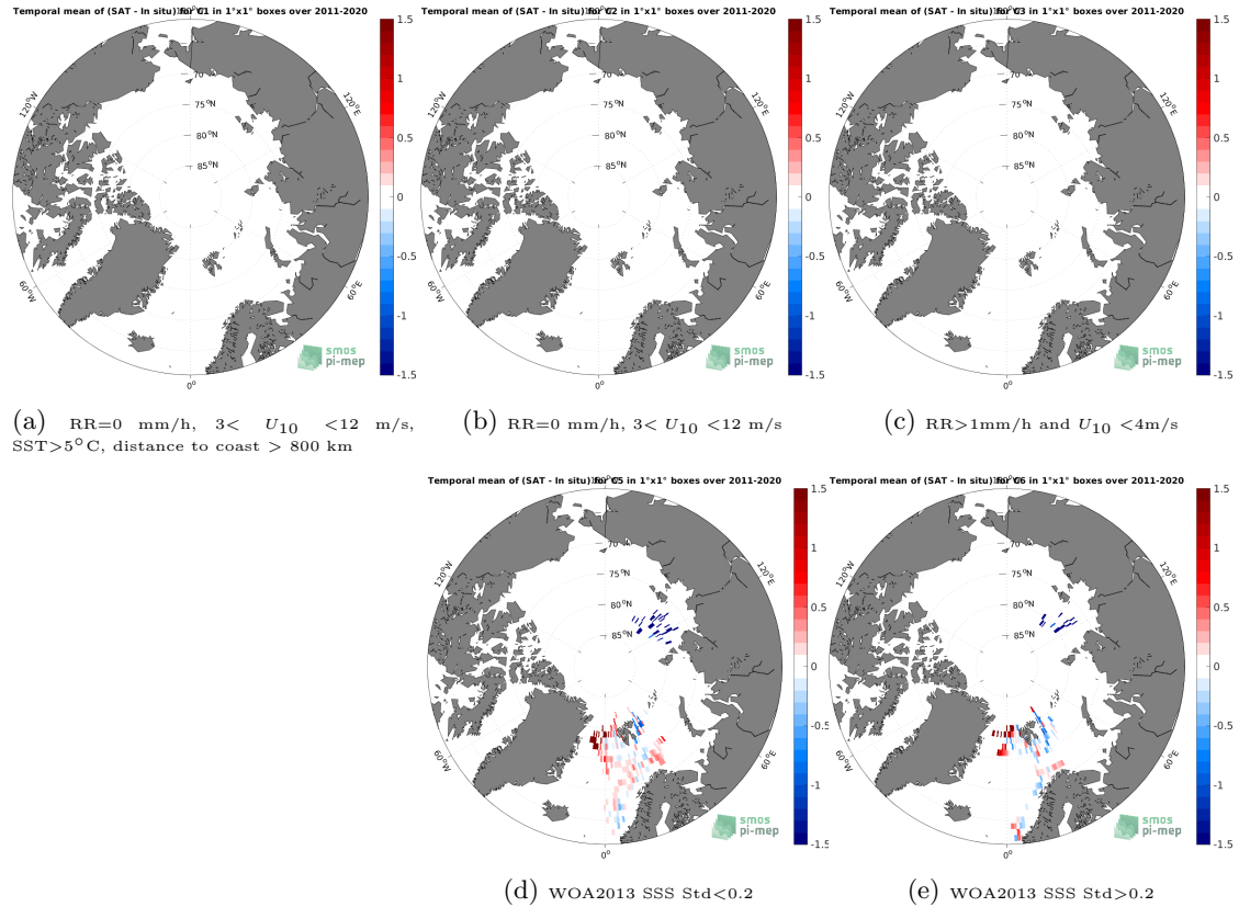
Figure 12: Temporal mean gridded over spatial boxes of size 1^{\circ}\times 1^{\circ} of \Delta\text{SSS} (SMAP SSS L4 OI v2 - 7 Days (ESR) - TSG (Polarstern)) for 5 different subdatasets corresponding to:RR=0 mm/h, 3 < U_{10} < 12 m/s, SST > 5^{\circ}\text{C} , distance to coast > 800 km (a), RR=0 mm/h, 3 < U_{10} < 12 m/s (b), RR > 1 mm/h and U_{10} < 4 m/s (c), WOA2013 SSS Std < 0.2 (d), WOA2013 SSS Std > 0.2 (e).
