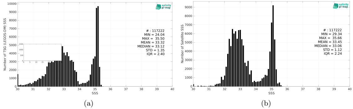
Figure 2: Histograms of SSS from TSG (LEGOS-DM) (a) and SMAP SSS L4 OI v2 - 7 Days (ESR) (b) considering all match-up pairs per bins of 0.1 over the Arctic Ocean Pi-MEP region and for the full satellite product period.
