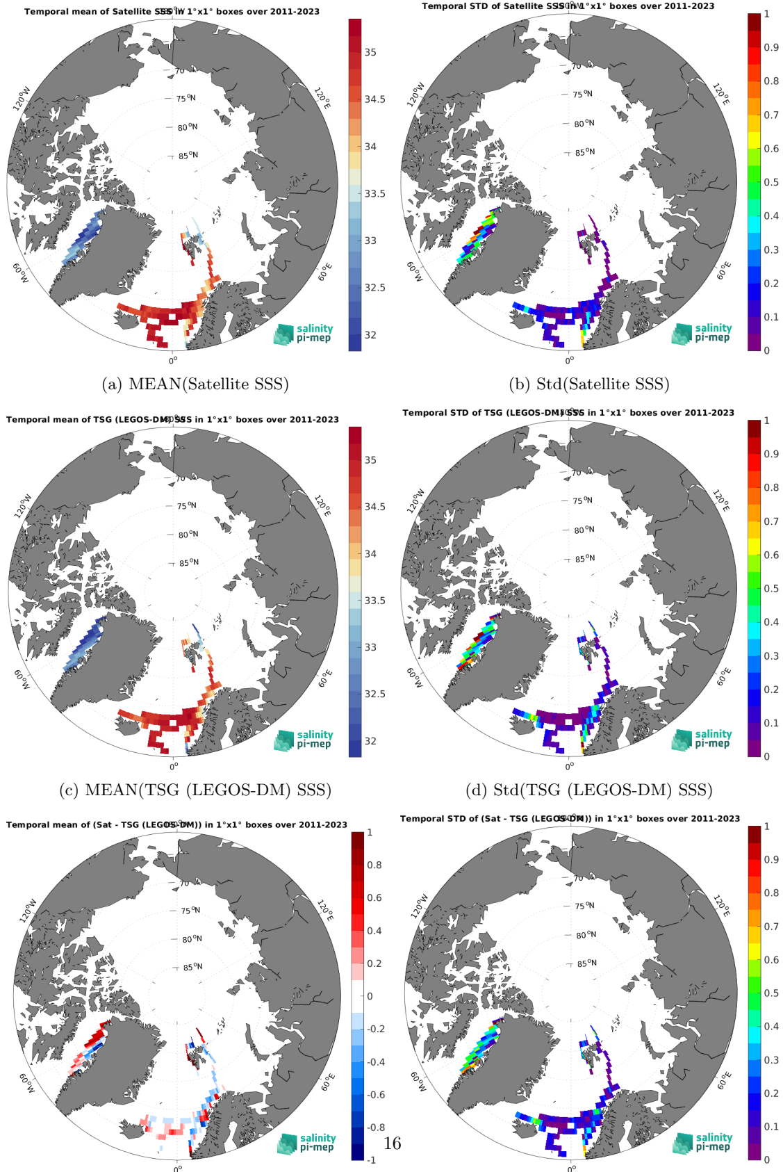
(e) MEAN( \Delta SSS) (Satellite - TSG (LEGOS-DM)) (f) Std( \Delta SSS) (Satellite - TSG (LEGOS-DM)) Figure 6: Temporal mean (left) and Std (right) of SSS from SMAP SSS L4 OI v2 - 7 Days (ESR) (top), TSG (LEGOS-DM) (middle), and of \Delta SSS (Satellite - TSG (LEGOS-DM)). Only match-up pairs are used to generate these maps.
