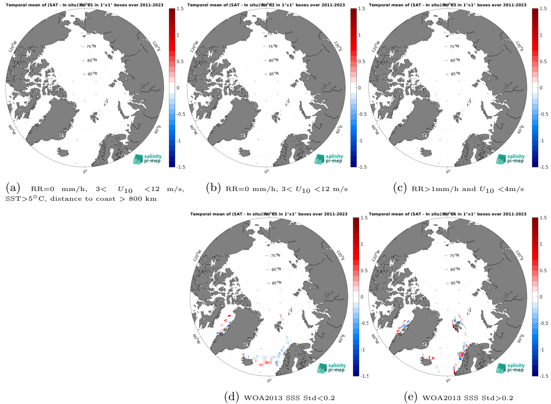
Figure 12: Temporal mean gridded over spatial boxes of size 1^{\circ}\times 1^{\circ} of \Delta\text{SSS} (SMAP SSS L4 OI v2 - 7 Days (ESR) - TSG (LEGOS-DM)) for 5 different subdatasets corresponding to:RR=0 mm/h, 3 < U_{10} < 12 m/s, SST > 5^{\circ}\text{C} , distance to coast > 800 km (a), RR=0 mm/h, 3 < U_{10} < 12 m/s (b), RR > 1 mm/h and U_{10} < 4 m/s (c), WOA2013 SSS Std < 0.2 (d), WOA2013 SSS Std > 0.2 (e).
