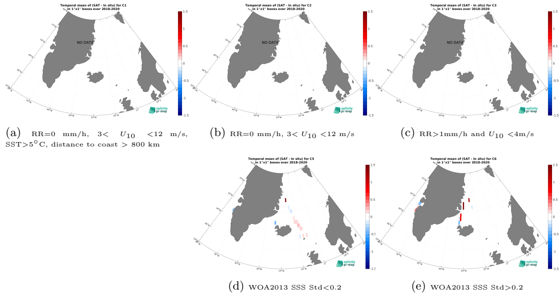
Figure 12: Temporal mean gridded over spatial boxes of size 1^{\circ}\times 1^{\circ} of \Delta\text{SSS} (SMAP SSS L4 OI v2 - 7 Days (ESR) - TSG (Lauge-Koch)) for 5 different subdatasets corresponding to:RR=0 mm/h, 3 < U_{10} < 12 m/s, SST >5^{\circ}\text{C} , distance to coast > 800 km (a), RR=0 mm/h, 3 < U_{10} < 12 m/s (b), RR >1 mm/h and U_{10} < 4 m/s (c), WOA2013 SSS Std <0.2 (d), WOA2013 SSS Std >0.2 (e).
