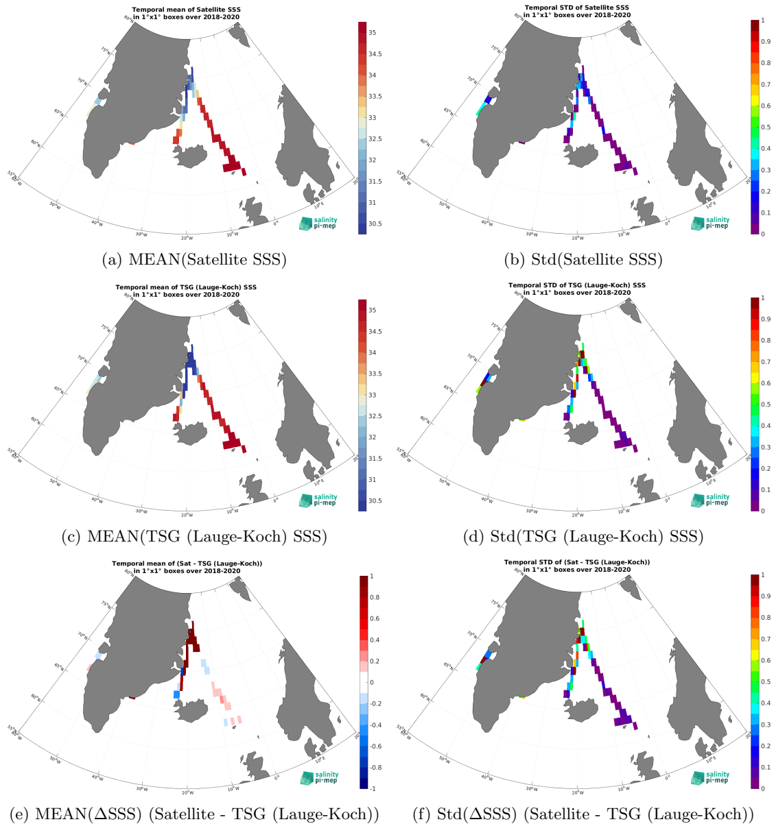
Figure 6: Temporal mean (left) and Std (right) of SSS from SMAP SSS L4 OI v2 - 7 Days (ESR) (top), TSG (Lauge-Koch) (middle), and of \Delta SSS (Satellite - TSG (Lauge-Koch)). Only match-up pairs are used to generate these maps.
