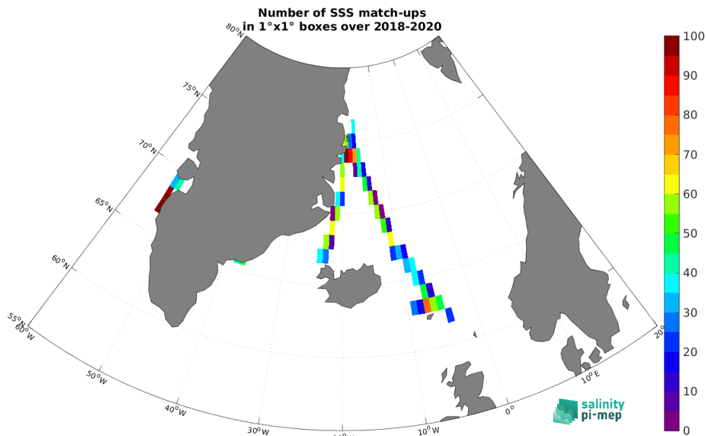
Figure 4: Number of SSS match-ups between TSG (Lauge-Koch) SSS and the SMAP SSS L4 OI v2 - 7 Days (ESR) SSS product for the Arctic Ocean Pi-MEP region over 1^\circ \times 1^\circ boxes and for the full satellite product period.
