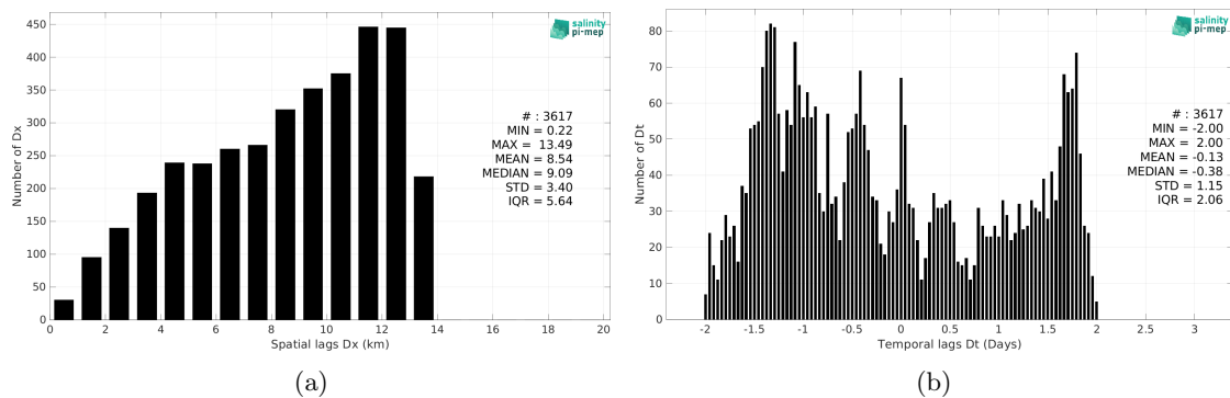
Figure 5: Histograms of the spatial (a) and temporal (b) lags between the location/time of the TSG (Lauge-Koch) measurement and the date of the corresponding SMAP SSS L4 OI v2 - 7 Days (ESR) SSS pixel.
