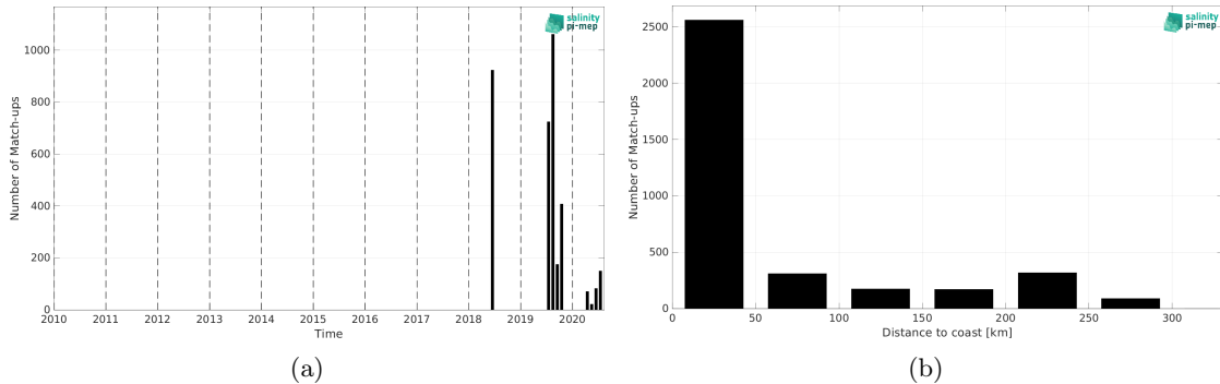
Figure 1: Number of match-ups between TSG (Lauge-Koch) and SMAP SSS L4 OI v2 - 7 Days (ESR) SSS as a function of time (a) and as function of the distance to coast (b) over the Arctic Ocean Pi-MEP region and for the full satellite product period.
