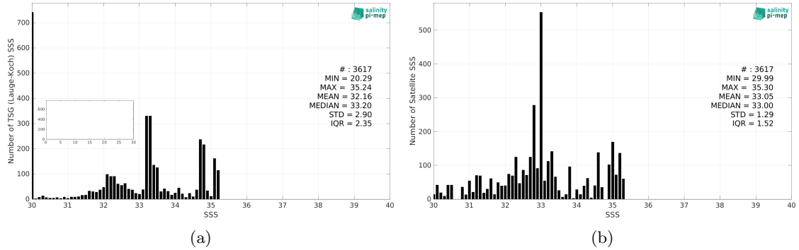
Figure 2: Histograms of SSS from TSG (Lauge-Koch) (a) and SMAP SSS L4 OI v2 - 7 Days (ESR) (b) considering all match-up pairs per bins of 0.1 over the Arctic Ocean Pi-MEP region and for the full satellite product period.
