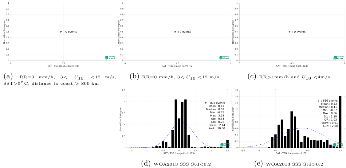
Figure 13: Normalized histogram of \Delta SSS (SMAP SSS L4 OI v2 - 7 Days (ESR) - TSG (Lauge-Koch)) for 5 different subdatasets corresponding to: RR=0 mm/h, 3 < U_{10} < 12 m/s, SST>5°C, distance to coast > 800 km (a), RR=0 mm/h, 3 < U_{10} < 12 m/s (b), RR>1mm/h and U_{10} < 4 m/s (c), WOA2013 SSS Std<0.2 (d), WOA2013 SSS Std>0.2 (e).
