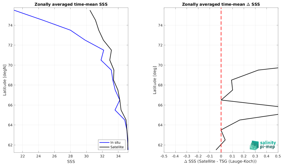
Figure 8: Left panel: Zonal mean SSS from SMAP SSS L4 OI v2 - 7 Days (ESR) satellite product (black) and from TSG (Lauge-Koch) (blue). Right panel: Zonal mean of \Delta SSS (Satellite - TSG (Lauge-Koch)) for all the collected Pi-MEP match-up pairs estimated over the full satellite product period.
