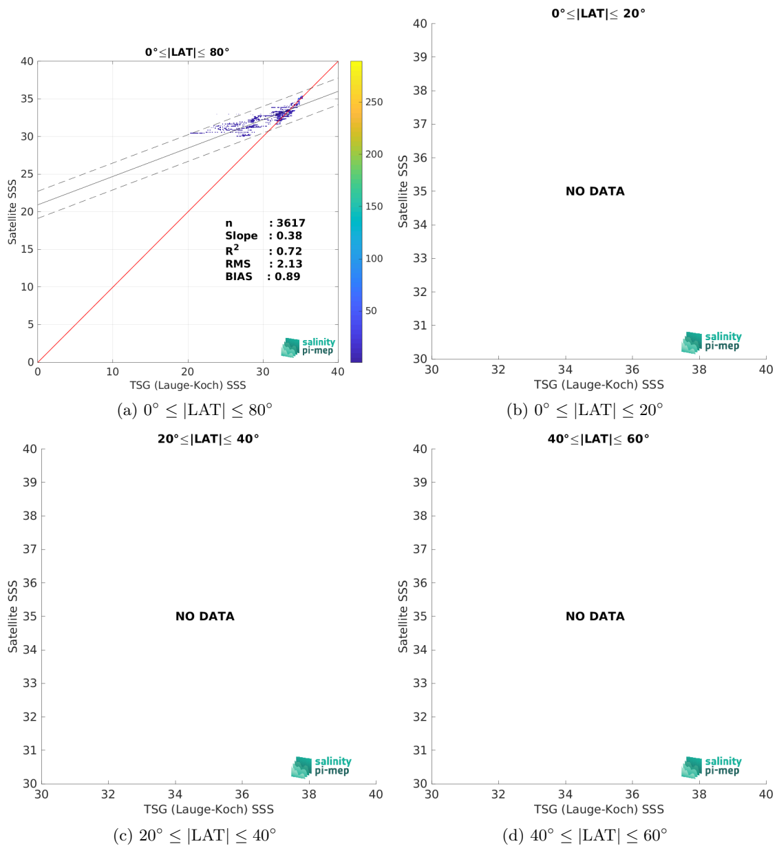
Figure 9: Contour maps of the concentration of SMAP SSS L4 OI v2 - 7 Days (ESR) SSS (y-axis) versus TSG (Lauge-Koch) SSS (x-axis) at match-up pairs for different latitude bands. For each plot, the red line shows x=y . The black thin and dashed lines indicate a linear fit through the data cloud and the \pm 95\% confidence levels, respectively. The number match-up pairs n , the slope and R^2 coefficient of the linear fit, the root mean square (RMS) and the mean bias between satellite and in situ data are indicated for each latitude band in each plots.
