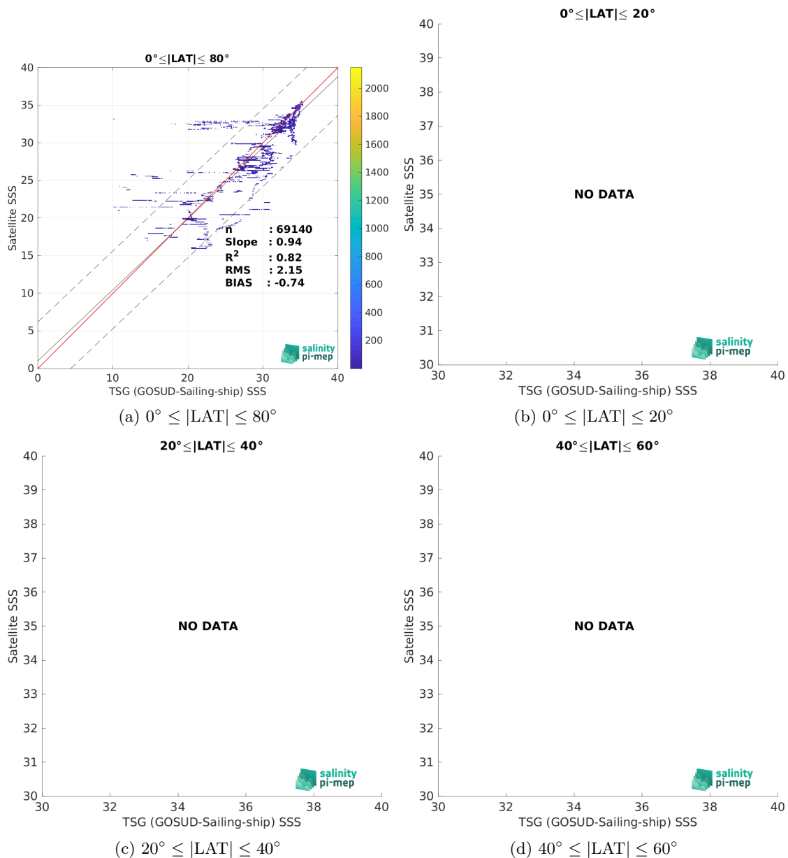
Figure 9: Contour maps of the concentration of SMAP SSS L4 OI v2 - 7 Days (ESR) SSS (y-axis) versus TSG (GOSUD-Sailing-ship) SSS (x-axis) at match-up pairs for different latitude bands. For each plot, the red line shows x=y . The black thin and dashed lines indicate a linear fit through the data cloud and the \pm 95\% confidence levels, respectively. The number match-up pairs n , the slope and R^2 coefficient of the linear fit, the root mean square (RMS) and the mean bias between satellite and in situ data are indicated for each latitude band in each plots.
