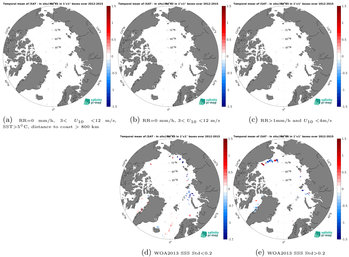
Figure 12: Temporal mean gridded over spatial boxes of size 1^\circ \times 1^\circ of \Delta SSS (SMAP SSS L4 OI v2 - 7 Days (ESR) - TSG (GOSUD-Sailing-ship)) for 5 different subdatasets corresponding to: RR=0 mm/h, 3 < U_{10} < 12 m/s, SST>5°C, distance to coast > 800 km (a), RR=0 mm/h, 3 < U_{10} < 12 m/s (b), RR>1mm/h and U_{10} < 4 m/s (c), WOA2013 SSS Std<0.2 (d), WOA2013 SSS Std>0.2 (e).
