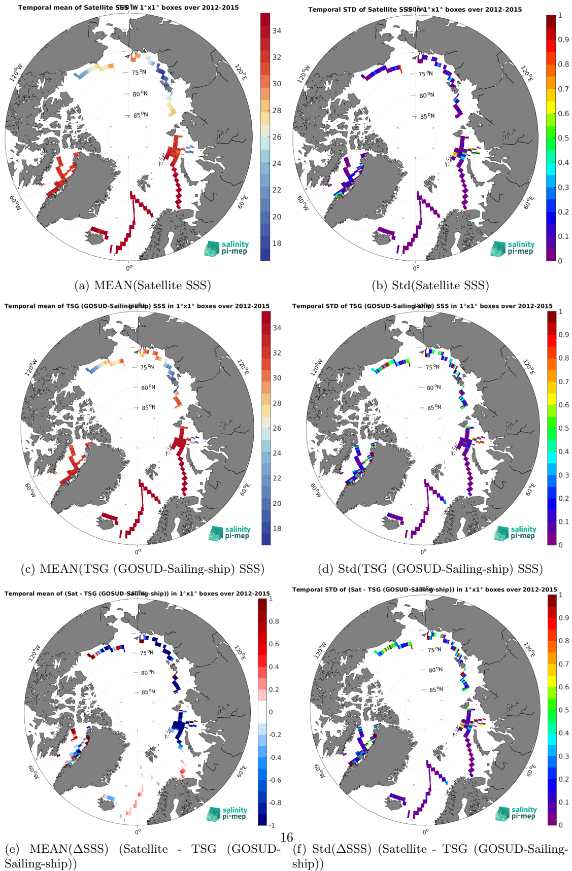
Figure 6: Temporal mean (left) and Std (right) of SSS from SMAP SSS L4 OI v2 - 7 Days (ESR) (top), TSG (GOSUD-Sailing-ship) (middle), and of \Delta SSS (Satellite - TSG (GOSUD-Sailing-ship)). Only match-up pairs are used to generate these maps.
