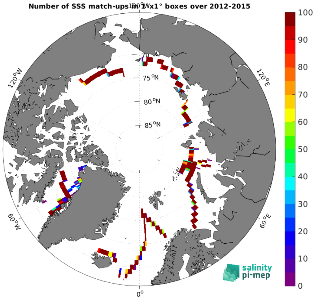
Figure 4: Number of SSS match-ups between TSG (GOSUD-Sailing-ship) SSS and the SMAP SSS L4 OI v2 - 7 Days (ESR) SSS product for the Arctic Ocean Pi-MEP region over 1^\circ \times 1^\circ boxes and for the full satellite product period.
