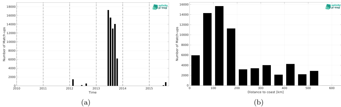
Figure 1: Number of match-ups between TSG (GOSUD-Sailing-ship) and SMAP SSS L4 OI v2 - 7 Days (ESR) SSS as a function of time (a) and as function of the distance to coast (b) over the Arctic Ocean Pi-MEP region and for the full satellite product period.
