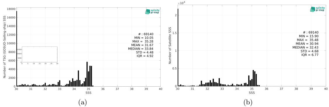
Figure 2: Histograms of SSS from TSG (GOSUD-Sailing-ship) (a) and SMAP SSS L4 OI v2 - 7 Days (ESR) (b) considering all match-up pairs per bins of 0.1 over the Arctic Ocean Pi-MEP region and for the full satellite product period.
