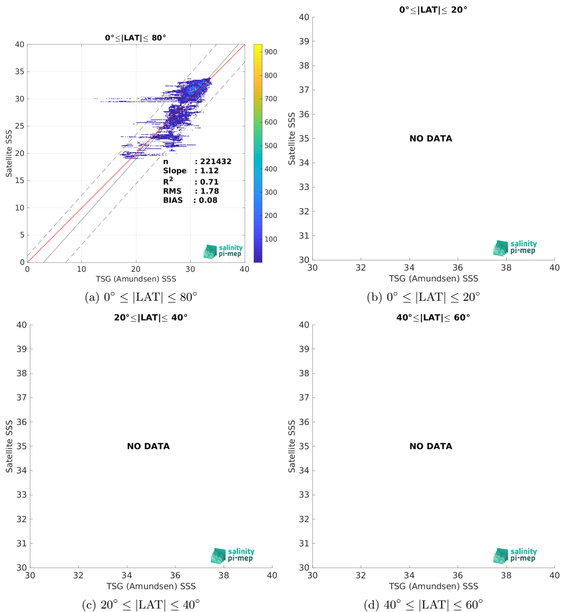
Figure 9: Contour maps of the concentration of SMAP SSS L4 OI v2 - 7 Days (ESR) SSS (y-axis) versus TSG (Amundsen) SSS (x-axis) at match-up pairs for different latitude bands. For each plot, the red line shows x=y . The black thin and dashed lines indicate a linear fit through the data cloud and the \pm 95\% confidence levels, respectively. The number match-up pairs n , the slope and R^2 coefficient of the linear fit, the root mean square (RMS) and the mean bias between satellite and in situ data are indicated for each latitude band in each plots.
