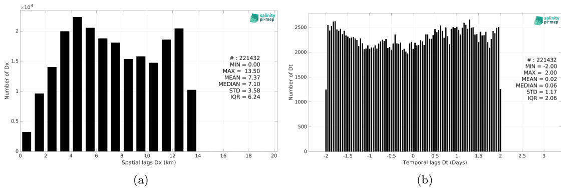
Figure 5: Histograms of the spatial (a) and temporal (b) lags between the location/time of the TSG (Amundsen) measurement and the date of the corresponding SMAP SSS L4 OI v2 - 7 Days (ESR) SSS pixel.
