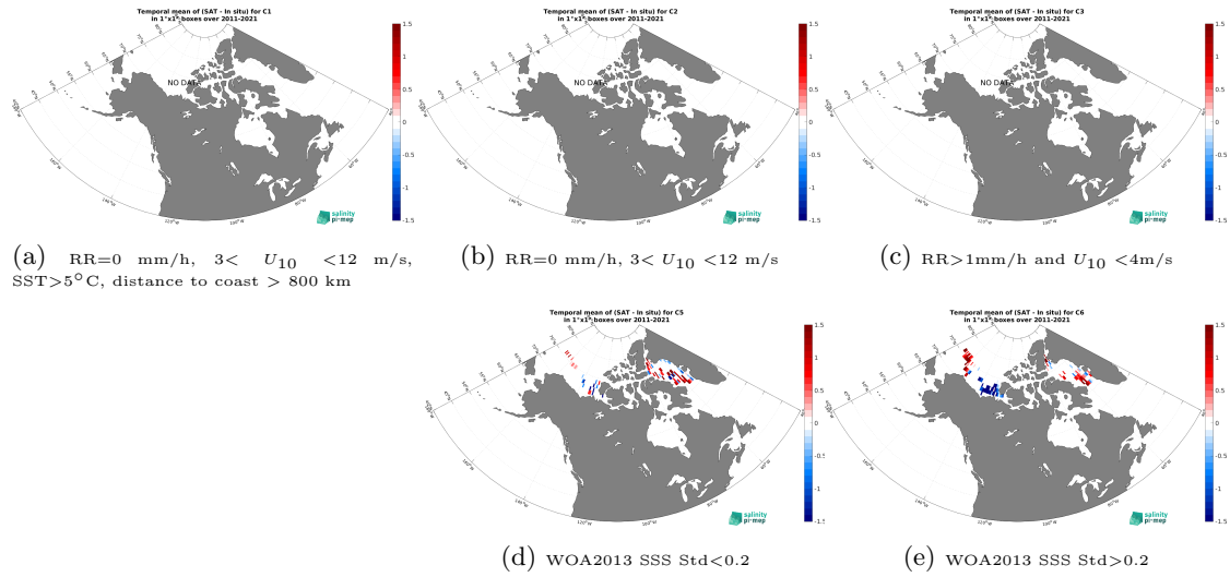
Figure 12: Temporal mean gridded over spatial boxes of size 1^{\circ}\times 1^{\circ} of \Delta\text{SSS} (SMAP SSS L4 OI v2 - 7 Days (ESR) - TSG (Amundsen)) for 5 different subdatasets corresponding to:RR=0 mm/h, 3 < U_{10} < 12 m/s, SST > 5^{\circ}\text{C} , distance to coast > 800 km (a), RR=0 mm/h, 3 < U_{10} < 12 m/s (b), RR > 1 mm/h and U_{10} < 4 m/s (c), WOA2013 SSS Std < 0.2 (d), WOA2013 SSS Std > 0.2 (e).
