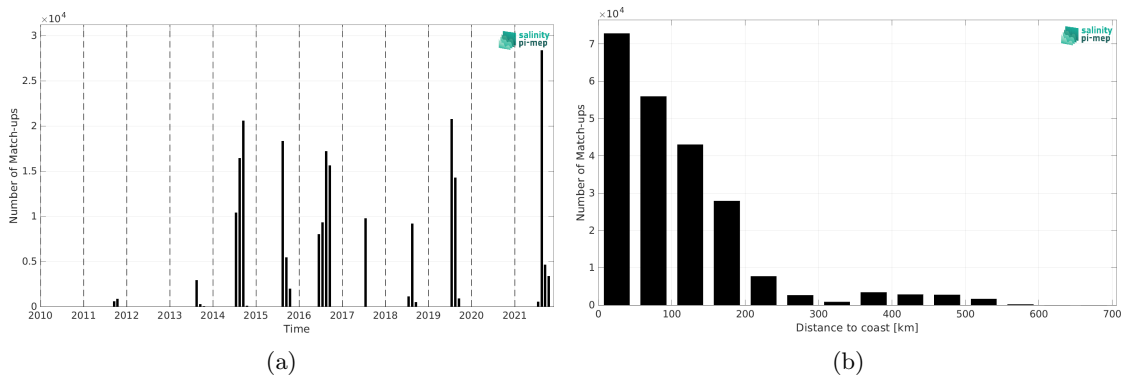
Figure 1: Number of match-ups between TSG (Amundsen) and SMAP SSS L4 OI v2 - 7 Days (ESR) SSS as a function of time (a) and as function of the distance to coast (b) over the Arctic Ocean Pi-MEP region and for the full satellite product period.
