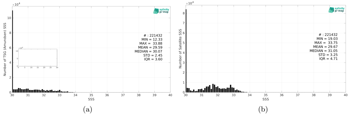
Figure 2: Histograms of SSS from TSG (Amundsen) (a) and SMAP SSS L4 OI v2 - 7 Days (ESR) (b) considering all match-up pairs per bins of 0.1 over the Arctic Ocean Pi-MEP region and for the full satellite product period.
