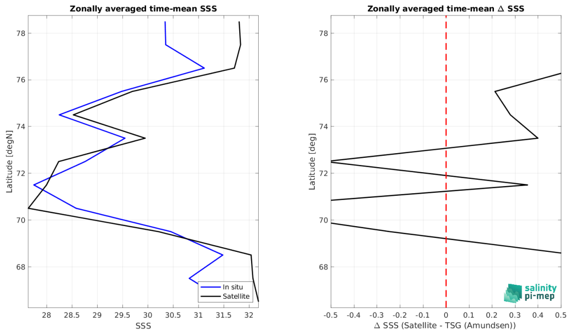
Figure 8: Left panel: Zonal mean SSS from SMAP SSS L4 OI v2 - 7 Days (ESR) satellite product (black) and from TSG (Amundsen) (blue). Right panel: Zonal mean of \Delta SSS (Satellite - TSG (Amundsen)) for all the collected Pi-MEP match-up pairs estimated over the full satellite product period.
