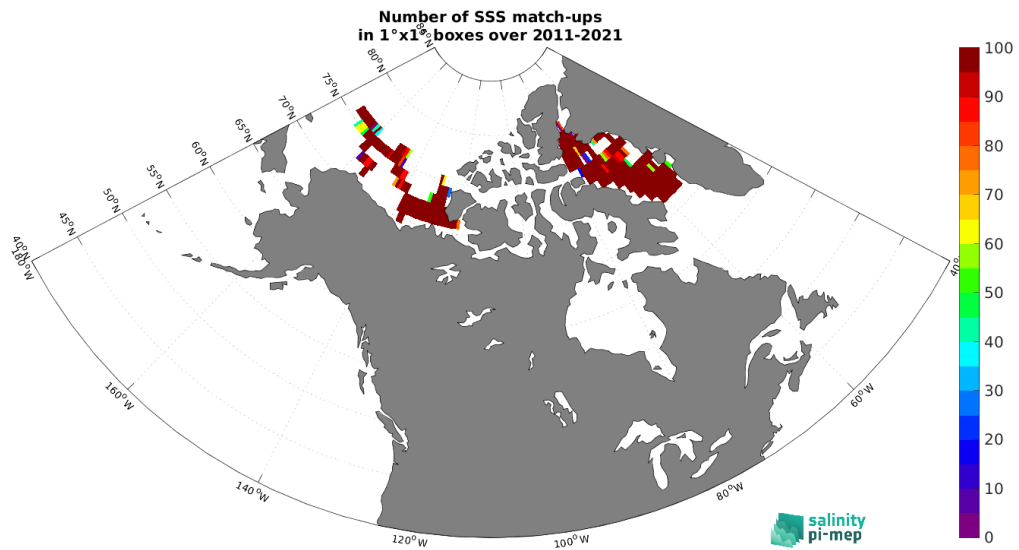
Figure 4: Number of SSS match-ups between TSG (Amundsen) SSS and the SMAP SSS L4 OI v2 - 7 Days (ESR) SSS product for the Arctic Ocean Pi-MEP region over 1^\circ \times 1^\circ boxes and for the full satellite product period.
