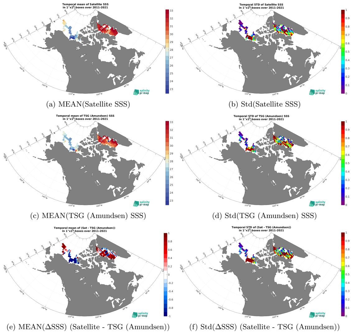
Figure 6: Temporal mean (left) and Std (right) of SSS from SMAP SSS L4 OI v2 - 7 Days (ESR) (top), TSG (Amundsen) (middle), and of \Delta SSS (Satellite - TSG (Amundsen)). Only match-up pairs are used to generate these maps.
