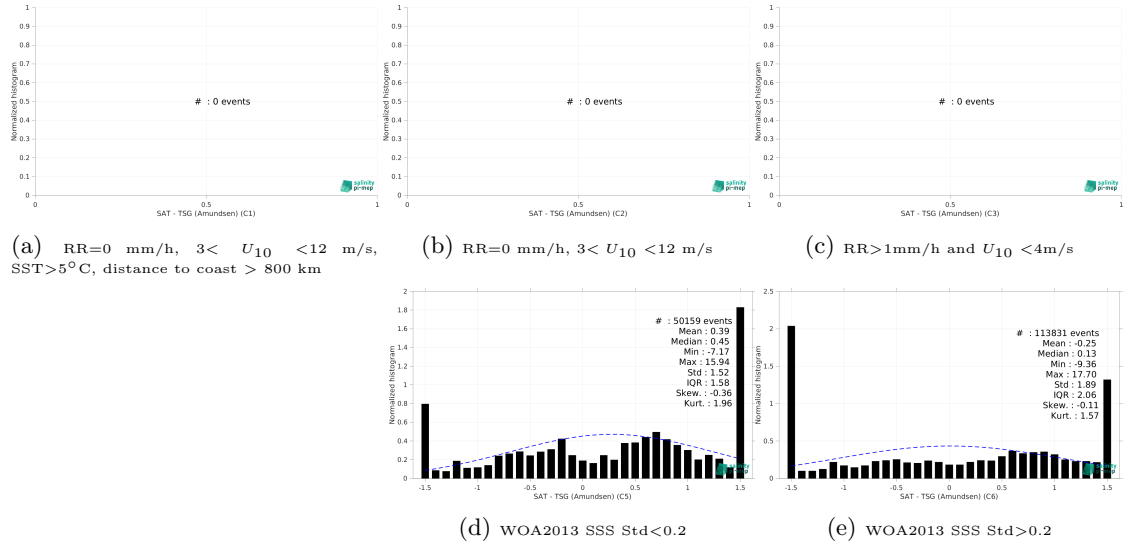
Figure 13: Normalized histogram of \Delta SSS (SMAP SSS L4 OI v2 - 7 Days (ESR) - TSG (Amundsen)) for 5 different subdatasets corresponding to: RR=0 mm/h, 3 < U_{10} < 12 m/s, SST>5°C, distance to coast > 800 km (a), RR=0 mm/h, 3 < U_{10} < 12 m/s (b), RR>1mm/h and U_{10} < 4 m/s (c), WOA2013 SSS Std<0.2 (d), WOA2013 SSS Std>0.2 (e).
