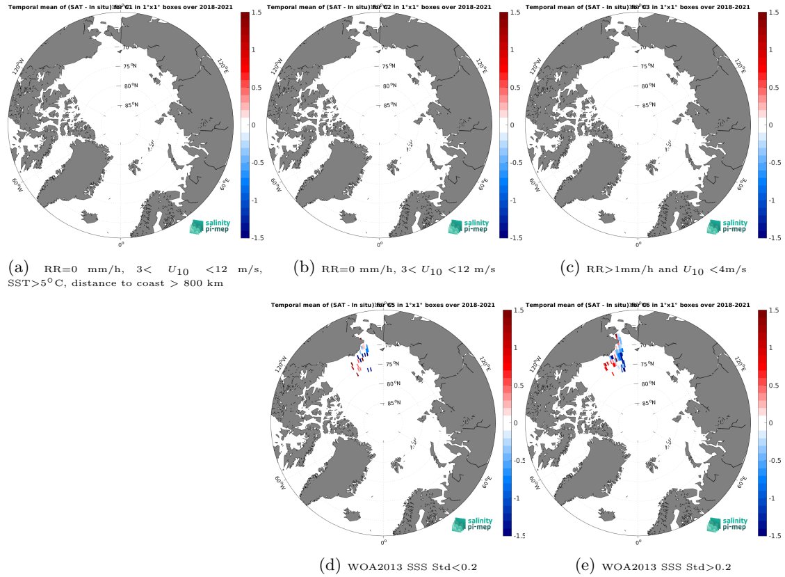
Figure 12: Temporal mean gridded over spatial boxes of size 1^{\circ}\times 1^{\circ} of \Delta\text{SSS} (SMAP SSS L4 OI v2 - 7 Days (ESR) - Sailability) for 5 different subdatasets corresponding to:RR=0 mm/h, 3 < U_{10} < 12 m/s, SST > 5^{\circ}\text{C} , distance to coast > 800 km (a), RR=0 mm/h, 3 < U_{10} < 12 m/s (b), RR > 1 mm/h and U_{10} < 4 m/s (c), WOA2013 SSS Std < 0.2 (d), WOA2013 SSS Std > 0.2 (e).
