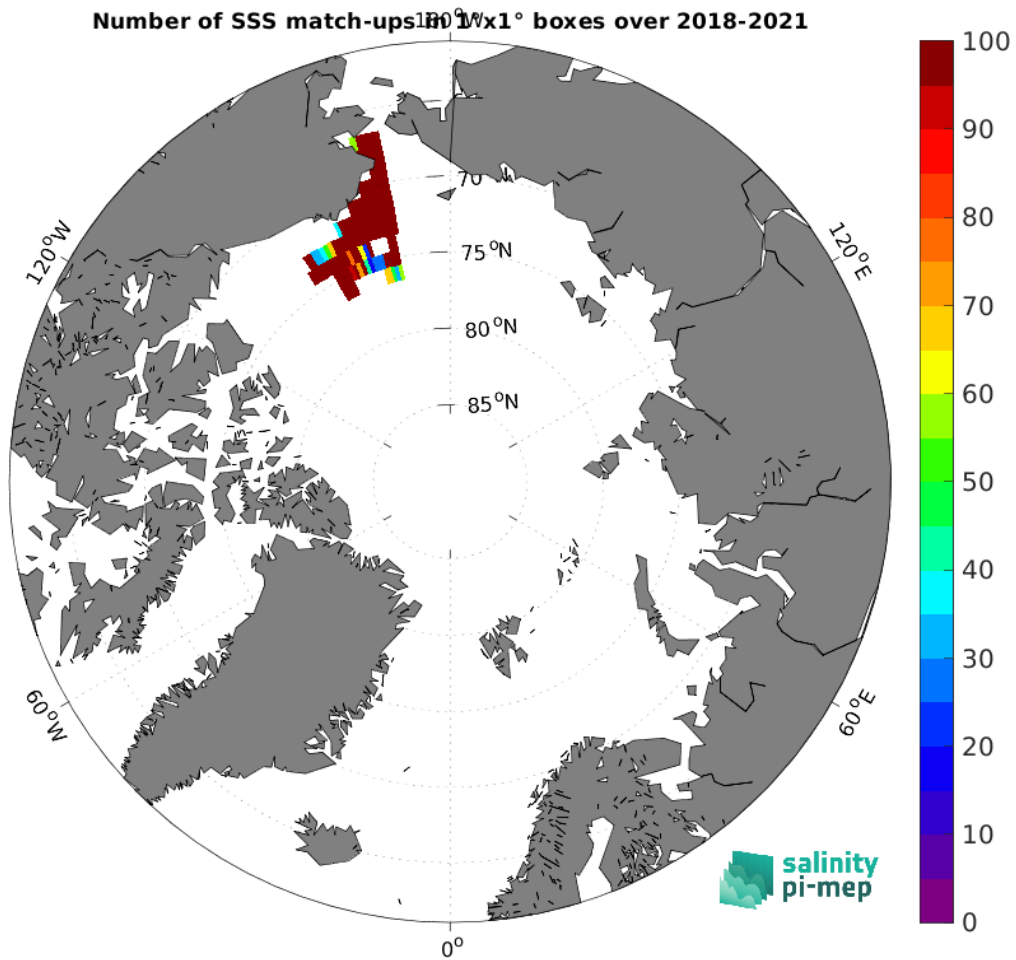
Figure 4: Number of SSS match-ups between Sairdrones SSS and the SMAP SSS L4 OI v2 - 7 Days (ESR) SSS product for the Arctic Ocean Pi-MEP region over 1^\circ \times 1^\circ boxes and for the full satellite product period.
