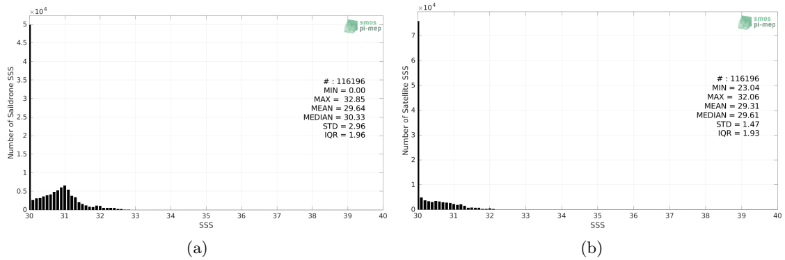
Figure 2: Histograms of SSS from Saildrone (a) and SMAP SSS L4 OI v2 - 7 Days (ESR) (b) considering all match-up pairs per bins of 0.1 over the Arctic Ocean Pi-MEP region and for the full satellite product period.
