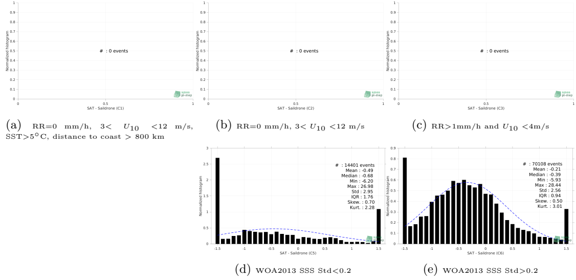
Figure 13: Normalized histogram of \Delta SSS (SMAP SSS L4 OI v2 - 7 Days (ESR) - Saldrone) for 5 different subdatasets corresponding to: RR=0 mm/h, 3 < U_{10} < 12 m/s, SST>5°C, distance to coast > 800 km (a), RR=0 mm/h, 3 < U_{10} < 12 m/s (b), RR>1mm/h and U_{10} < 4 m/s (c), WOA2013 SSS Std<0.2 (d), WOA2013 SSS Std>0.2 (e).
