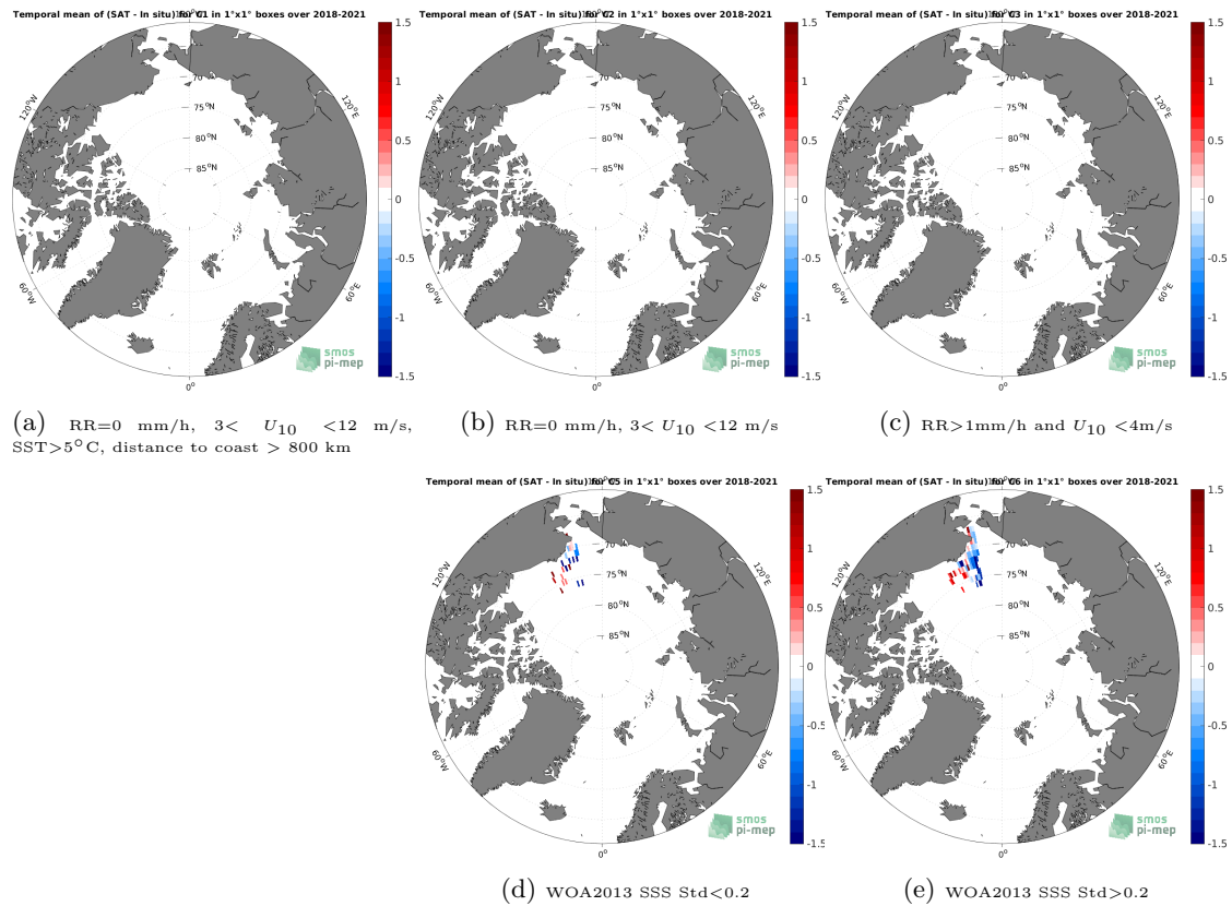
Figure 12: Temporal mean gridded over spatial boxes of size 1^{\circ}\times 1^{\circ} of \Delta\text{SSS} (SMAP SSS L4 OI v2 - 7 Days (ESR) - Sairdrone) for 5 different subdatasets corresponding to:RR=0 mm/h, 3 < U_{10} < 12 m/s, SST >5^{\circ}\text{C} , distance to coast > 800 km (a), RR=0 mm/h, 3 < U_{10} < 12 m/s (b), RR >1 mm/h and U_{10} < 4 m/s (c), WOA2013 SSS Std <0.2 (d), WOA2013 SSS Std >0.2 (e).
