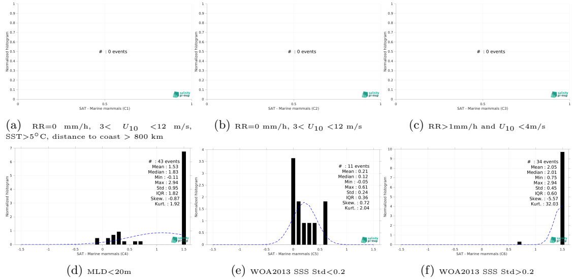
Figure 13: Normalized histogram of \Delta\text{SSS} (SMAP SSS L4 OI v2 - 7 Days (ESR) - Marine mammals) for 6 different subdatasets corresponding to: RR=0 mm/h, 3 < U_{10} < 12 m/s, SST > 5^\circ\text{C} , distance to coast > 800 km (a), RR=0 mm/h, 3 < U_{10} < 12 m/s (b), RR > 1\text{mm/h} and U_{10} < 4\text{m/s} (c), MLD < 20\text{m} (d), WOA2013 SSS Std < 0.2 (e), WOA2013 SSS Std > 0.2 (f).
