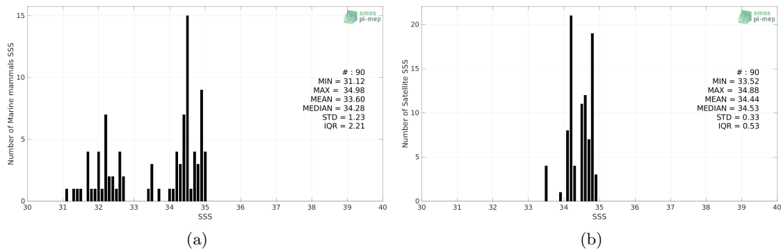
Figure 2: Histograms of SSS from Marine mammals (a) and SMAP SSS L4 OI v2 - 7 Days (ESR) (b) considering all match-up pairs per bins of 0.1 over the Arctic Ocean Pi-MEP region and for the full satellite product period.
