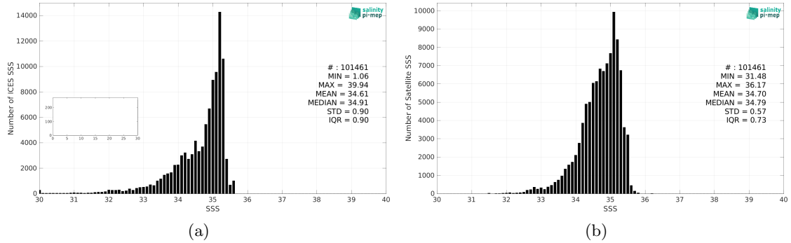
Figure 2: Histograms of SSS from ICES (a) and SMAP SSS L4 OI v2 - 7 Days (ESR) (b) considering all match-up pairs per bins of 0.1 over the Arctic Ocean Pi-MEP region and for the full satellite product period.
