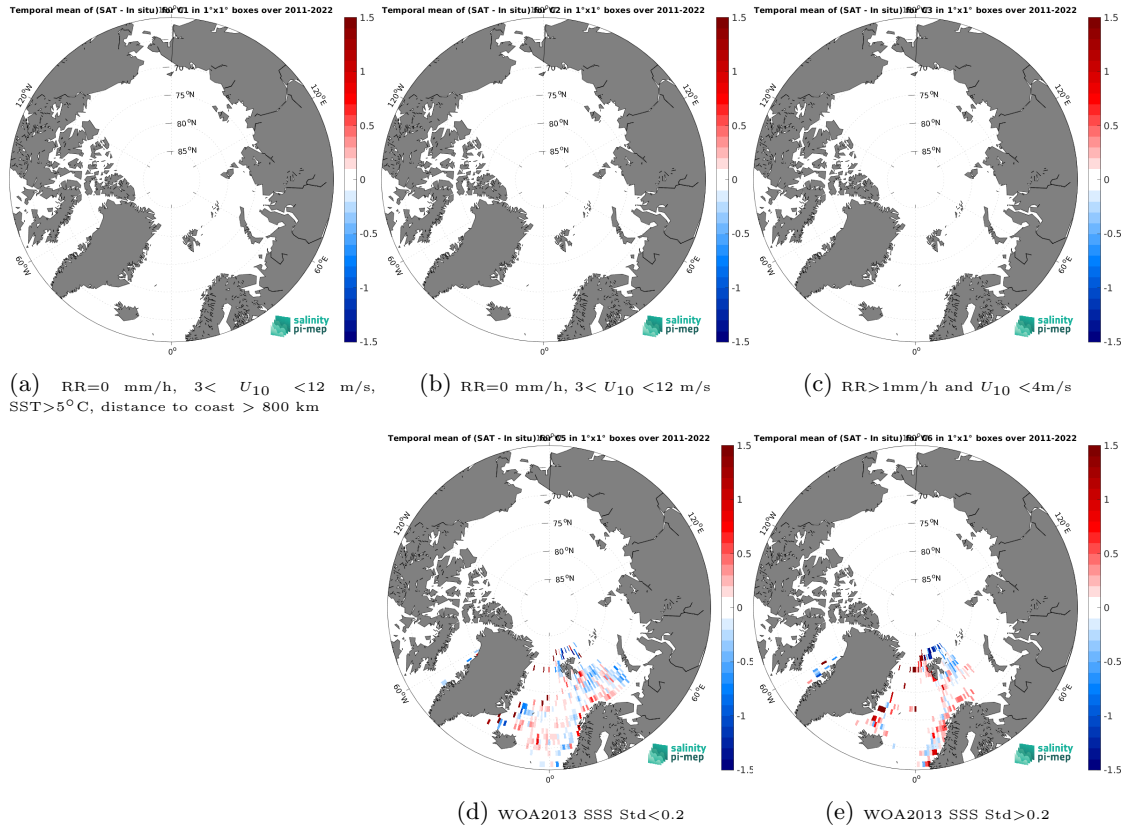
Figure 12: Temporal mean gridded over spatial boxes of size 1^{\circ}\times 1^{\circ} of \Delta\text{SSS} (SMAP SSS L4 OI v2 - 7 Days (ESR) - ICES) for 5 different subdatasets corresponding to: RR=0 mm/h, 3 < U_{10} < 12 m/s, SST > 5^{\circ}\text{C} , distance to coast > 800 km (a), RR=0 mm/h, 3 < U_{10} < 12 m/s (b), RR > 1 mm/h and U_{10} < 4 m/s (c), WOA2013 SSS Std < 0.2 (d), WOA2013 SSS Std > 0.2 (e).
