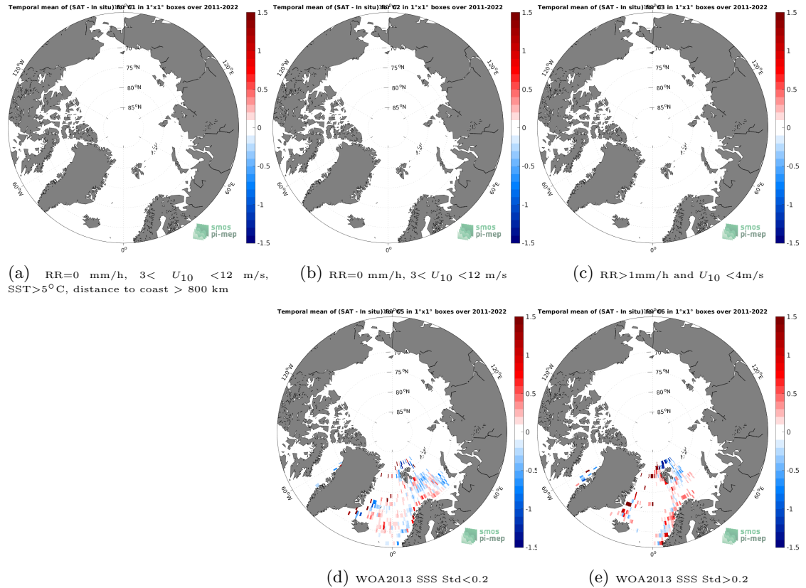
Figure 12: Temporal mean gridded over spatial boxes of size 1^{\circ}\times 1^{\circ} of \Delta\text{SSS} (SMAP SSS L4 OI v2 - 7 Days (ESR) - ICES) for 5 different subdatasets corresponding to:RR=0 mm/h, 3 < U_{10} < 12 m/s, SST >5^{\circ}\text{C} , distance to coast > 800 km (a), RR=0 mm/h, 3 < U_{10} < 12 m/s (b), RR >1 mm/h and U_{10} < 4 m/s (c), WOA2013 SSS Std <0.2 (d), WOA2013 SSS Std >0.2 (e).
