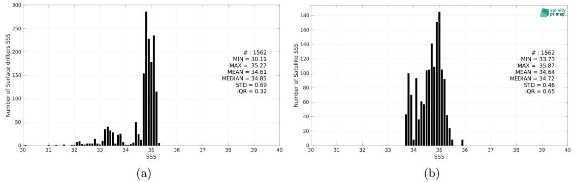
Figure 2: Histograms of SSS from Surface drifters (a) and SMAP SSS L4 OI v2 - 7 Days (ESR) (b) considering all match-up pairs per bins of 0.1 over the Arctic Ocean Pi-MEP region and for the full satellite product period.
