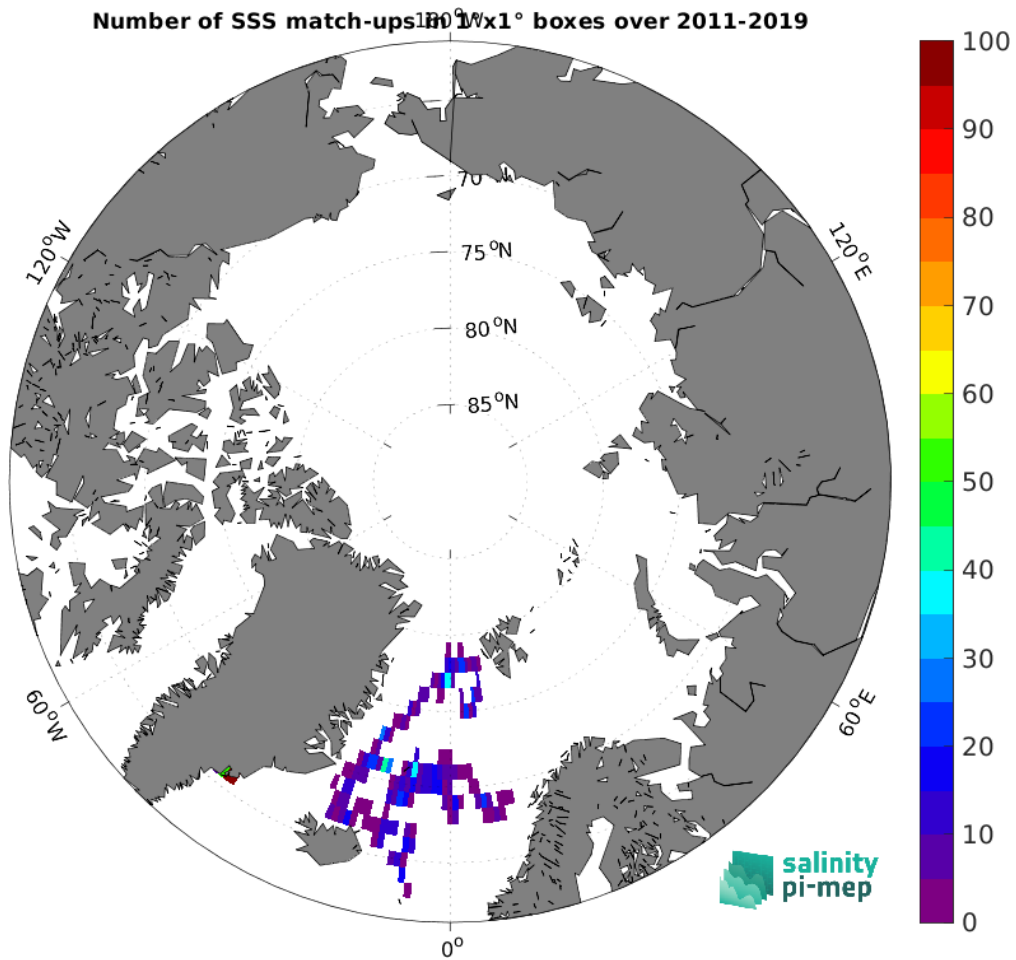
Figure 3: Number of SSS match-ups between Surface drifters SSS and the SMAP SSS L4 OI v2 - 7 Days (ESR) SSS product for the Arctic Ocean Pi-MEP region over 1^\circ \times 1^\circ boxes and for the full satellite product period.
