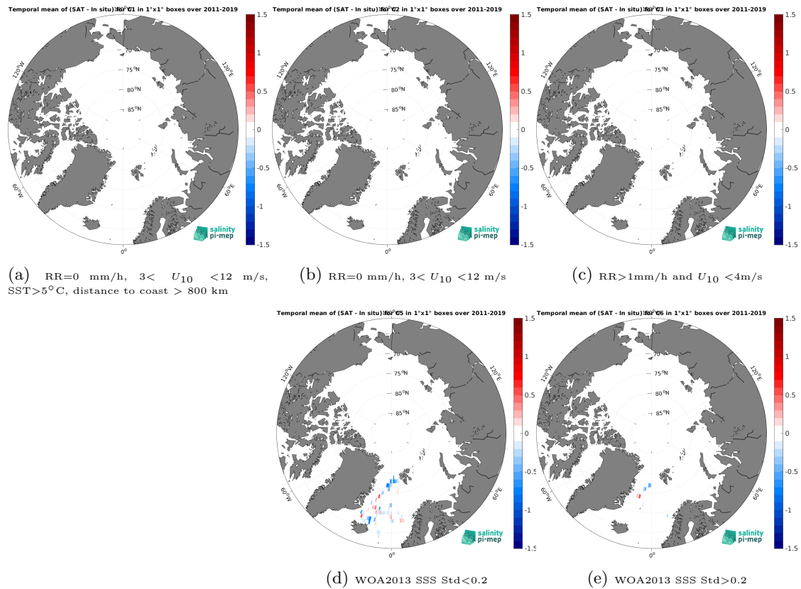
Figure 11: Temporal mean gridded over spatial boxes of size 1^{\circ}\times 1^{\circ} of \Delta\text{SSS} (SMAP SSS L4 OI v2 - 7 Days (ESR) - Surface drifters) for 5 different subdatasets corresponding to:RR=0 mm/h, 3 < U_{10} < 12 m/s, SST > 5^{\circ}\text{C} , distance to coast > 800 km (a), RR=0 mm/h, 3 < U_{10} < 12 m/s (b), RR > 1 mm/h and U_{10} < 4 m/s (c), WOA2013 SSS Std < 0.2 (d), WOA2013 SSS Std > 0.2 (e).
