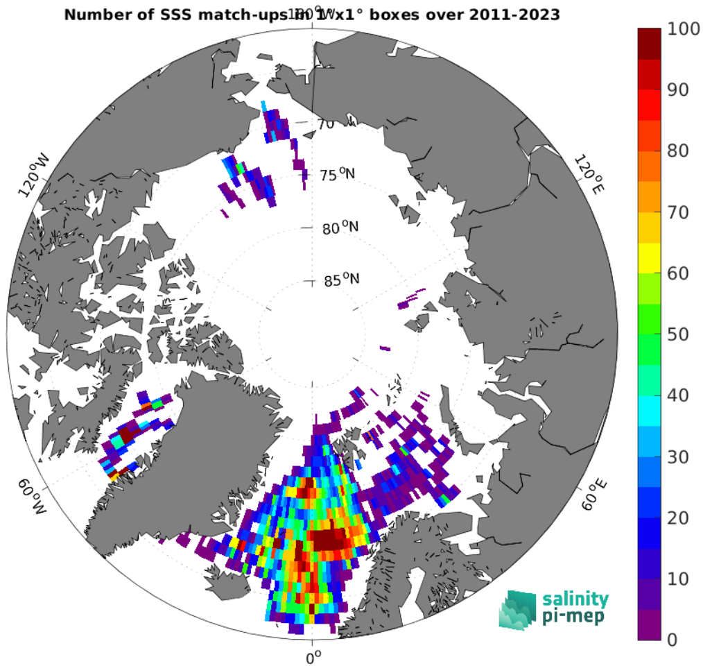
Figure 4: Number of SSS match-ups between Argo SSS and the SMAP SSS L4 OI v2 - 7 Days (ESR) SSS product for the Arctic Ocean Pi-MEP region over 1^\circ \times 1^\circ boxes and for the full satellite product period.
