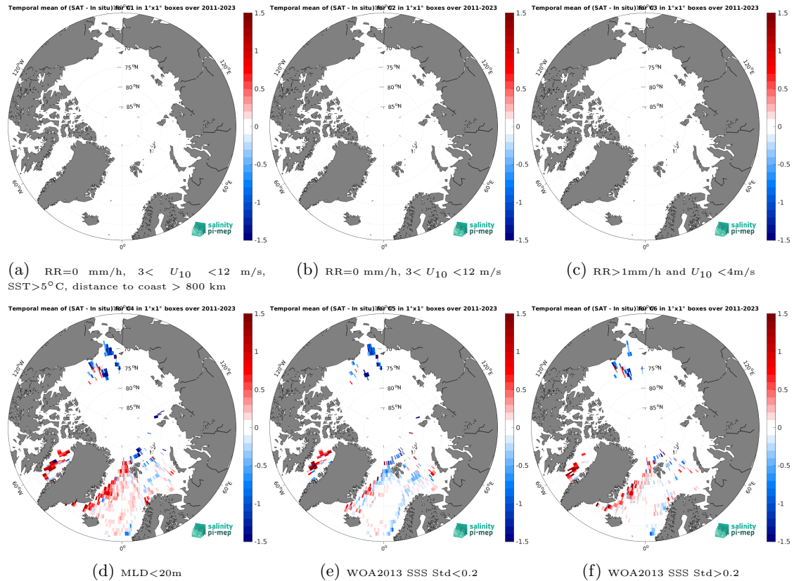
Figure 12: Temporal mean gridded over spatial boxes of size 1^{\circ}\times 1^{\circ} of \Delta\text{SSS} (SMAP SSS L4 OI v2 - 7 Days (ESR) - Argo) for 6 different subdatasets corresponding to: RR=0 mm/h, 3 < U_{10} < 12 m/s, SST > 5^{\circ}\text{C} , distance to coast > 800 km (a), RR=0 mm/h, 3 < U_{10} < 12 m/s (b), RR > 1\text{mm/h} and U_{10} < 4\text{m/s} (c), MLD < 20\text{m} (d), WOA2013 SSS Std < 0.2 (e), WOA2013 SSS Std > 0.2 (f).
