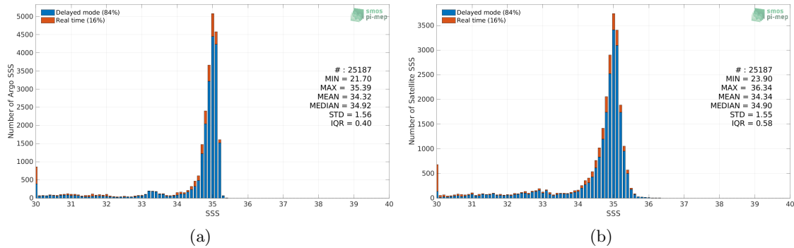
Figure 2: Histograms of SSS from Argo (a) and SMAP SSS L4 OI v2 - 7 Days (ESR) (b) considering all match-up pairs per bins of 0.1 over the Arctic Ocean Pi-MEP region and for the full satellite product period.
