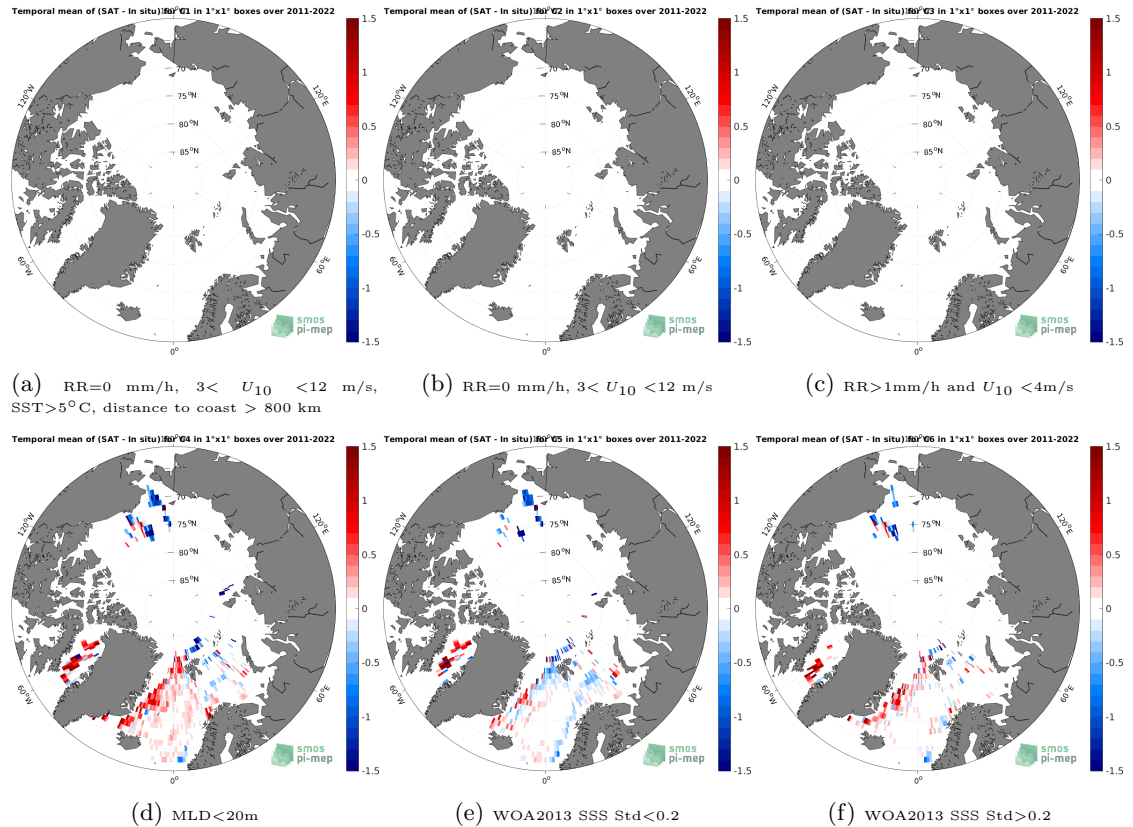
Figure 12: Temporal mean gridded over spatial boxes of size 1^{\circ}\times 1^{\circ} of \Delta\text{SSS} (SMAP SSS L4 OI v2 - 7 Days (ESR) - Argo) for 6 different subdatasets corresponding to:RR=0 mm/h, 3 < U_{10} < 12 m/s, SST > 5^{\circ}\text{C} , distance to coast > 800 km (a), RR=0 mm/h, 3 < U_{10} < 12 m/s (b), RR > 1\text{mm/h} and U_{10} < 4\text{m/s} (c),MLD < 20\text{m} (d),WOA2013 SSS Std < 0.2 (e),WOA2013 SSS Std > 0.2 (f).
