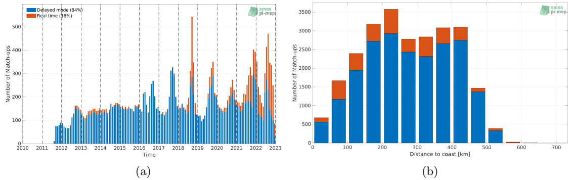
Figure 1: Number of match-ups between Argo and SMAP SSS L4 OI v2 - 7 Days (ESR) SSS as a function of time (a) and as function of the distance to coast (b) over the Arctic Ocean Pi-MEP region and for the full satellite product period.
