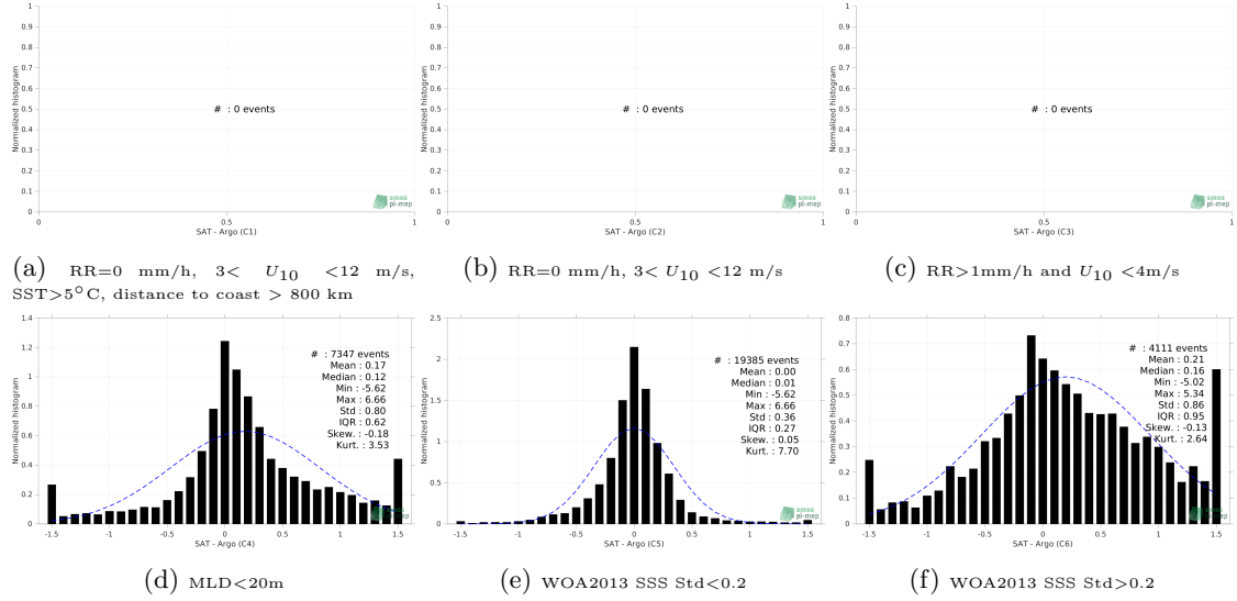
Figure 13: Normalized histogram of \Delta SSS (SMAP SSS L4 OI v2 - 7 Days (ESR) - Argo) for 6 different subdatasets corresponding to: RR=0 mm/h, 3 < U_{10} < 12 m/s, SST > 5°C, distance to coast > 800 km (a), RR=0 mm/h, 3 < U_{10} < 12 m/s (b), RR > 1mm/h and U_{10} < 4 m/s (c), MLD < 20m (d), WOA2013 SSS Std < 0.2 (e), WOA2013 SSS Std > 0.2 (f).
