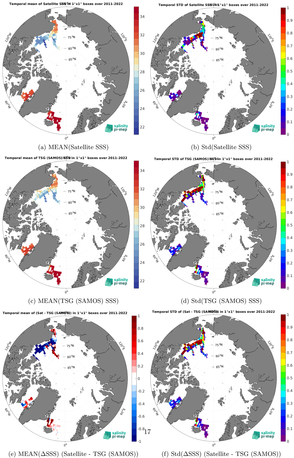
Figure 6: Temporal mean (left) and Std (right) of SSS from SMAP SSS L4 OI v2 - Monthly (IPRC) (top), TSG (SAMOS) (middle), and of \Delta SSS (Satellite - TSG (SAMOS)). Only match-up pairs are used to generate these maps.
