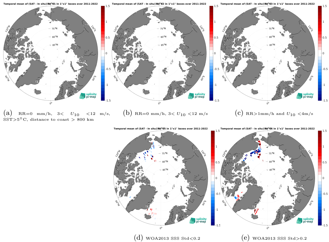
Figure 12: Temporal mean gridded over spatial boxes of size 1^{\circ}\times 1^{\circ} of \Delta\text{SSS} (SMAP SSS L4 OI v2 - Monthly (IPRC) - TSG (SAMOS)) for 5 different subdatasets corresponding to:RR=0 mm/h, 3 < U_{10} < 12 m/s, SST >5^{\circ}\text{C} , distance to coast > 800 km (a), RR=0 mm/h, 3 < U_{10} < 12 m/s (b), RR >1 mm/h and U_{10} < 4 m/s (c), WOA2013 SSS Std <0.2 (d), WOA2013 SSS Std >0.2 (e).
