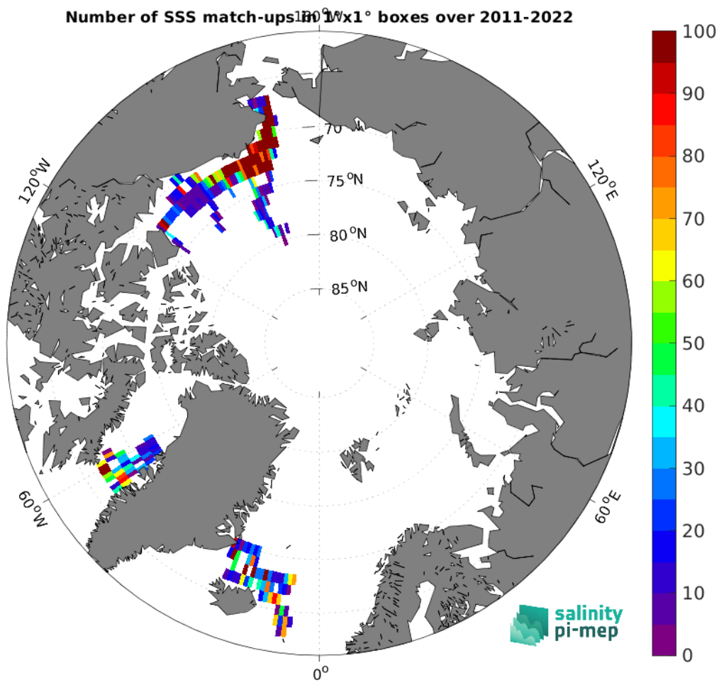
Figure 4: Number of SSS match-ups between TSG (SAMOS) SSS and the SMAP SSS L4 OI v2 - Monthly (IPRC) SSS product for the Arctic Ocean Pi-MEP region over 1^\circ \times 1^\circ boxes and for the full satellite product period.
