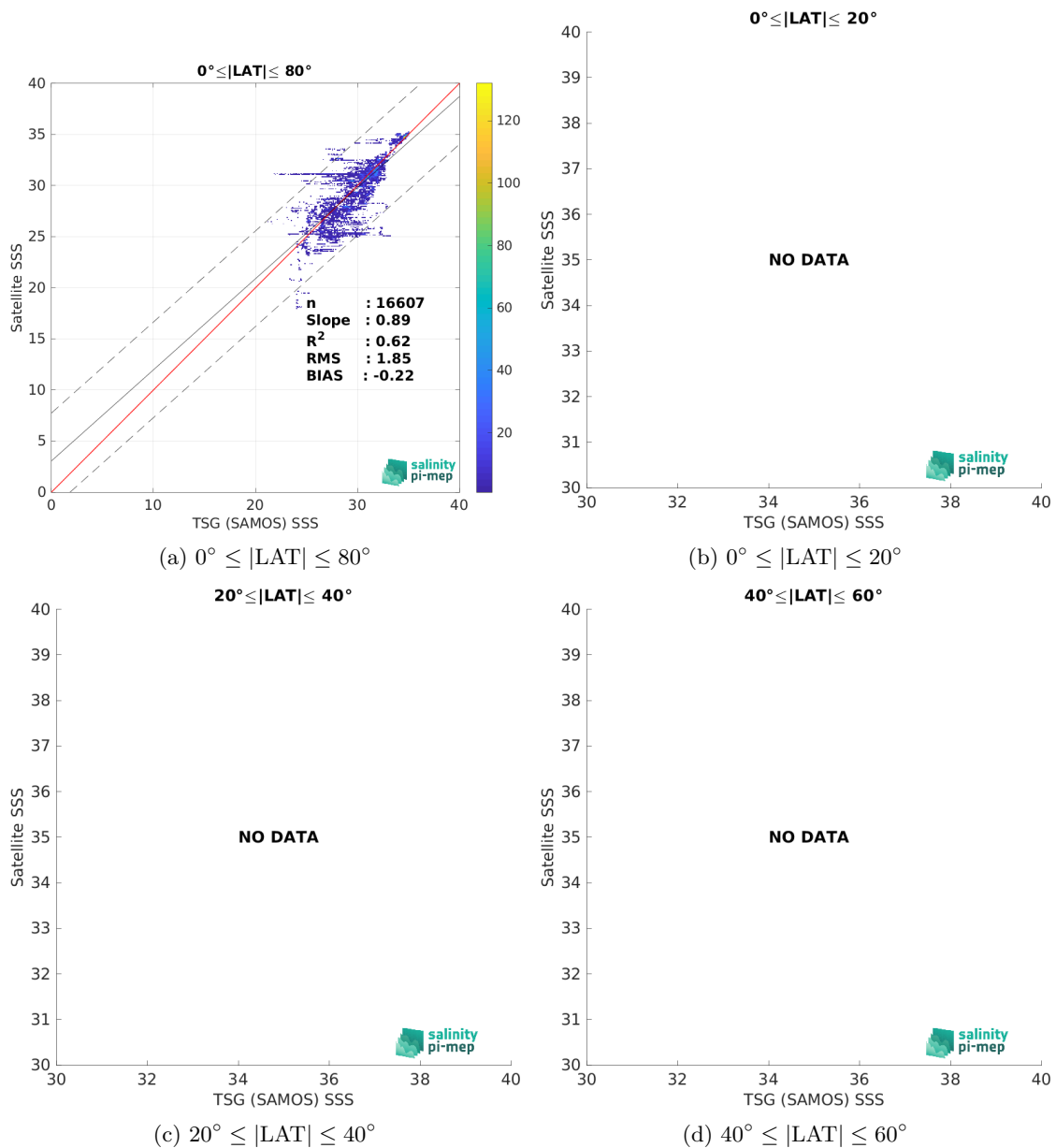
Figure 9: Contour maps of the concentration of SMAP SSS L4 OI v2 - Monthly (IPRC) SSS (y-axis) versus TSG (SAMOS) SSS (x-axis) at match-up pairs for different latitude bands. For each plot, the red line shows x=y . The black thin and dashed lines indicate a linear fit through the data cloud and the \pm 95\% confidence levels, respectively. The number match-up pairs n , the slope and R^2 coefficient of the linear fit, the root mean square (RMS) and the mean bias between satellite and in situ data are indicated for each latitude band in each plots.
