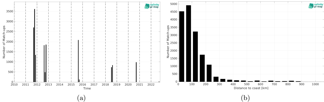
Figure 1: Number of match-ups between TSG (SAMOS) and SMAP SSS L4 OI v2 - Monthly (IPRC) SSS as a function of time (a) and as function of the distance to coast (b) over the Arctic Ocean Pi-MEP region and for the full satellite product period.
