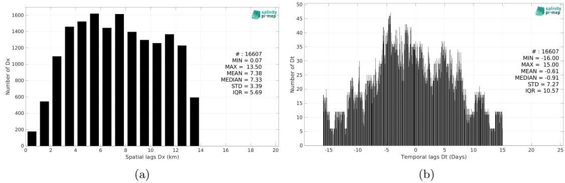
Figure 5: Histograms of the spatial (a) and temporal (b) lags between the location/time of the TSG (SAMOS) measurement and the date of the corresponding SMAP SSS L4 OI v2 - Monthly (IPRC) SSS pixel.
