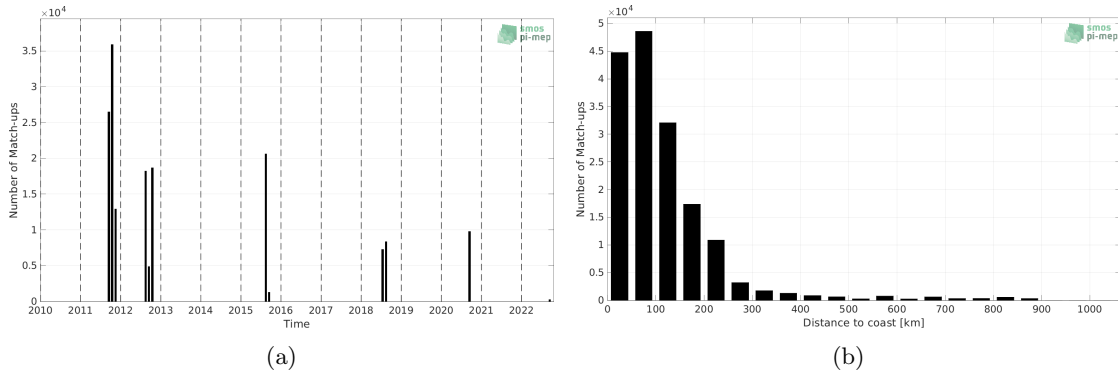
Figure 1: Number of match-ups between TSG (SAMOS) and SMAP SSS L4 OI v2 - Monthly (IPRC) SSS as a function of time (a) and as function of the distance to coast (b) over the Arctic Ocean Pi-MEP region and for the full satellite product period.
