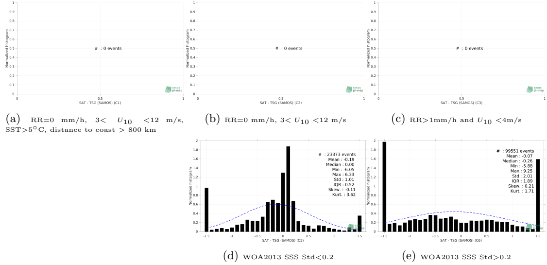
Figure 13: Normalized histogram of \Delta SSS (SMAP SSS L4 OI v2 - Monthly (IPRC) - TSG (SAMOS)) for 5 different subdatasets corresponding to: RR=0 mm/h, 3 < U_{10} < 12 m/s, SST >5^{\circ} C, distance to coast > 800 km (a), RR=0 mm/h, 3 < U_{10} < 12 m/s (b), RR >1 mm/h and U_{10} < 4 m/s (c), WOA2013 SSS Std <0.2 (d), WOA2013 SSS Std >0.2 (e).
