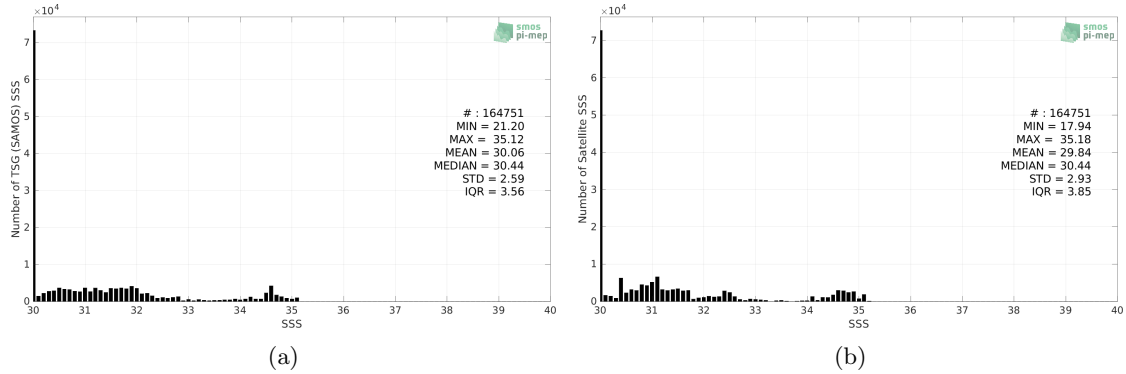
Figure 2: Histograms of SSS from TSG (SAMOS) (a) and SMAP SSS L4 OI v2 - Monthly (IPRC) (b) considering all match-up pairs per bins of 0.1 over the Arctic Ocean Pi-MEP region and for the full satellite product period.
