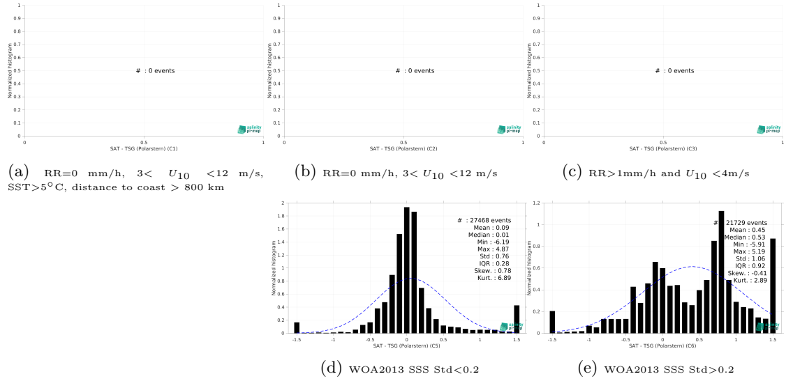
Figure 13: Normalized histogram of \Delta\text{SSS} (SMAP SSS L4 OI v2 - Monthly (IPRC) - TSG (Polarstern)) for 5 different subdatasets corresponding to: RR=0 mm/h, 3 < U_{10} < 12 m/s, SST > 5^\circ\text{C} , distance to coast > 800 km (a), RR=0 mm/h, 3 < U_{10} < 12 m/s (b), RR > 1\text{mm/h} and U_{10} < 4\text{m/s} (c), WOA2013 SSS Std < 0.2 (d), WOA2013 SSS Std > 0.2 (e).
