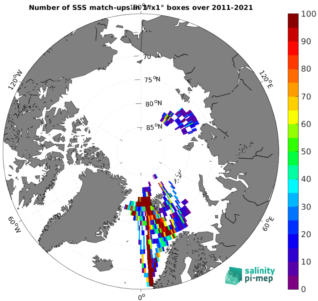
Figure 4: Number of SSS match-ups between TSG (Polarstern) SSS and the SMAP SSS L4 OI v2 - Monthly (IPRC) SSS product for the Arctic Ocean Pi-MEP region over 1^\circ \times 1^\circ boxes and for the full satellite product period.
