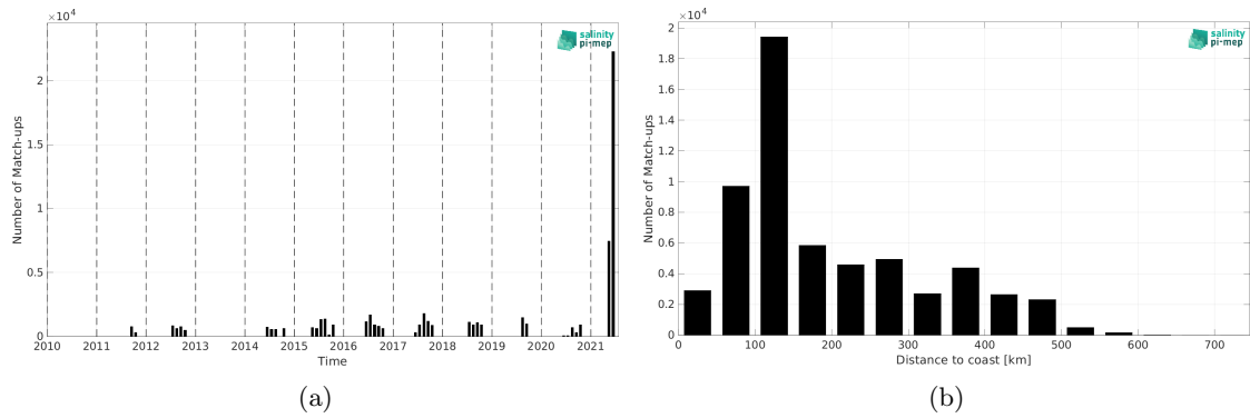
Figure 1: Number of match-ups between TSG (Polarstern) and SMAP SSS L4 OI v2 - Monthly (IPRC) SSS as a function of time (a) and as function of the distance to coast (b) over the Arctic Ocean Pi-MEP region and for the full satellite product period.
