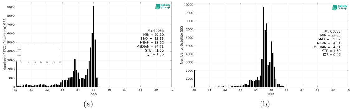
Figure 2: Histograms of SSS from TSG (Polarstern) (a) and SMAP SSS L4 OI v2 - Monthly (IPRC) (b) considering all match-up pairs per bins of 0.1 over the Arctic Ocean Pi-MEP region and for the full satellite product period.
