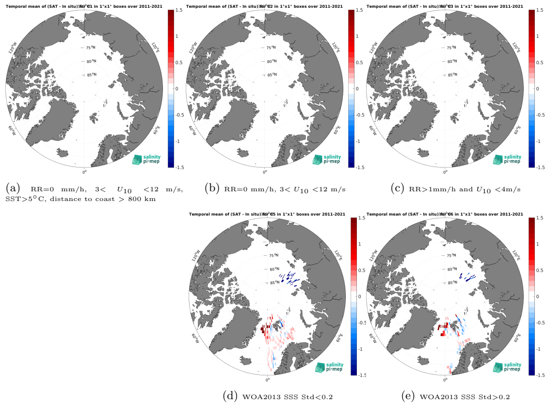
Figure 12: Temporal mean gridded over spatial boxes of size 1^{\circ}\times 1^{\circ} of \Delta\text{SSS} (SMAP SSS L4 OI v2 - Monthly (IPRC) - TSG (Polarstern)) for 5 different subdatasets corresponding to:RR=0 mm/h, 3 < U_{10} < 12 m/s, SST >5^{\circ}\text{C} , distance to coast > 800 km (a), RR=0 mm/h, 3 < U_{10} < 12 m/s (b), RR >1 mm/h and U_{10} < 4 m/s (c), WOA2013 SSS Std <0.2 (d), WOA2013 SSS Std >0.2 (e).
