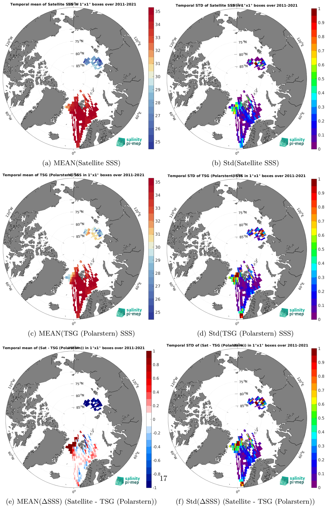
Figure 6: Temporal mean (left) and Std (right) of SSS from SMAP SSS L4 OI v2 - Monthly (IPRC) (top), TSG (Polarstern) (middle), and of \Delta SSS (Satellite - TSG (Polarstern)). Only match-up pairs are used to generate these maps.
