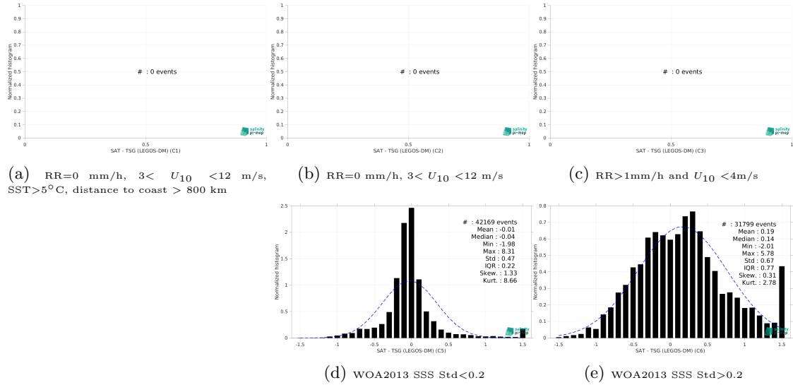
Figure 13: Normalized histogram of \Delta SSS (SMAP SSS L4 OI v2 - Monthly (IPRC) - TSG (LEGOS-DM)) for 5 different subdatasets corresponding to: RR=0 mm/h, 3 < U_{10} < 12 m/s, SST >5^{\circ} C, distance to coast > 800 km (a), RR=0 mm/h, 3 < U_{10} < 12 m/s (b), RR >1 mm/h and U_{10} < 4 m/s (c), WOA2013 SSS Std <0.2 (d), WOA2013 SSS Std >0.2 (e).
