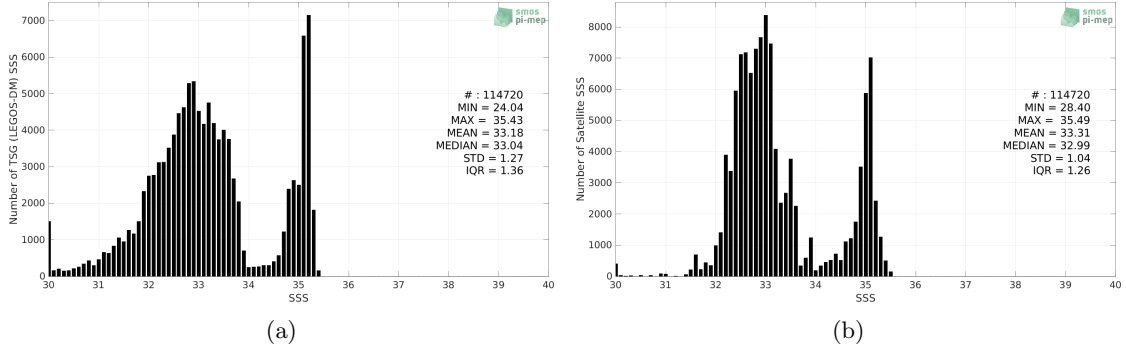
Figure 2: Histograms of SSS from TSG (LEGOS-DM) (a) and SMAP SSS L4 OI v2 - Monthly (IPRC) (b) considering all match-up pairs per bins of 0.1 over the Arctic Ocean Pi-MEP region and for the full satellite product period.
