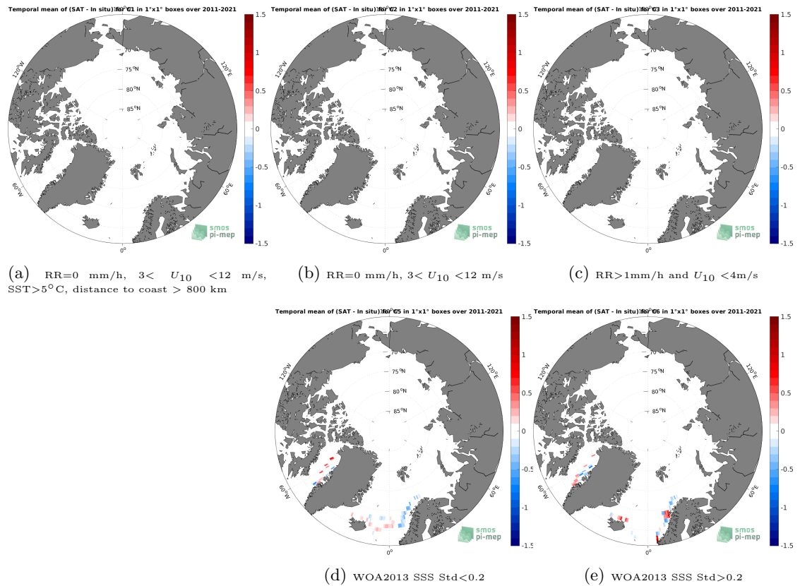
Figure 12: Temporal mean gridded over spatial boxes of size 1^{\circ}\times 1^{\circ} of \Delta\text{SSS} (SMAP SSS L4 OI v2 - Monthly (IPRC) - TSG (LEGOS-DM)) for 5 different subdatasets corresponding to:RR=0 mm/h, 3 < U_{10} < 12 m/s, SST >5^{\circ}\text{C} , distance to coast > 800 km (a), RR=0 mm/h, 3 < U_{10} < 12 m/s (b), RR >1 mm/h and U_{10} < 4 m/s (c), WOA2013 SSS Std <0.2 (d), WOA2013 SSS Std >0.2 (e).
