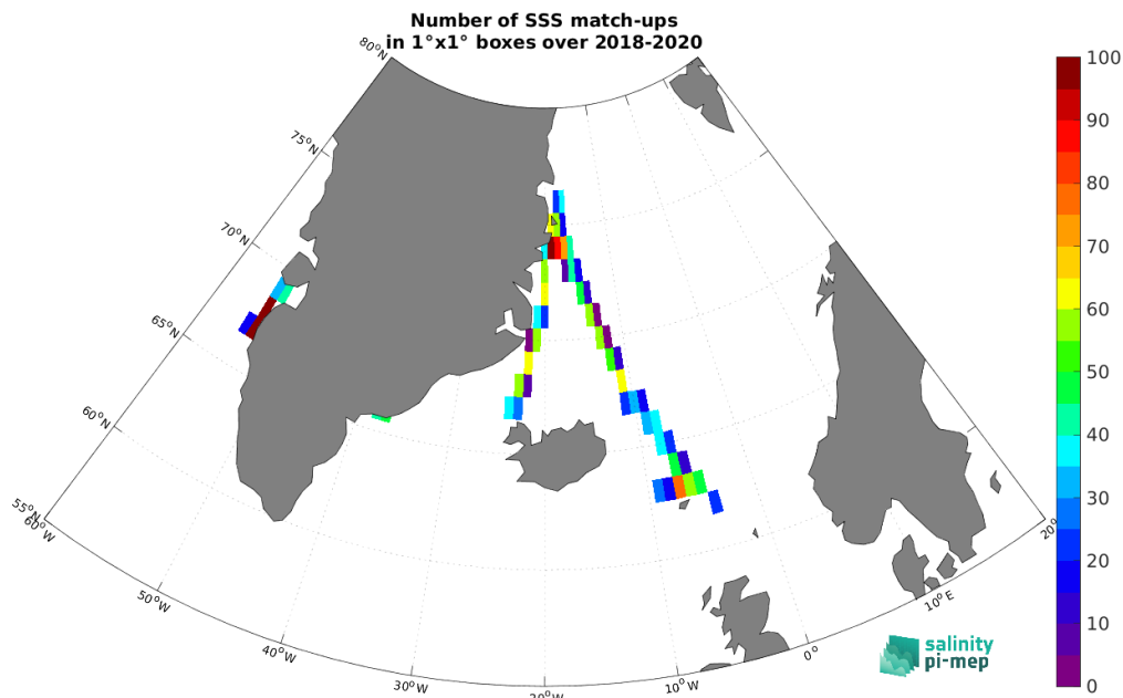
Figure 4: Number of SSS match-ups between TSG (Lauge-Koch) SSS and the SMAP SSS L4 OI v2 - Monthly (IPRC) SSS product for the Arctic Ocean Pi-MEP region over 1^\circ \times 1^\circ boxes and for the full satellite product period.
