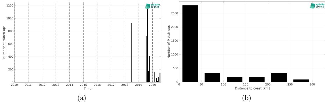
Figure 1: Number of match-ups between TSG (Lauge-Koch) and SMAP SSS L4 OI v2 - Monthly (IPRC) SSS as a function of time (a) and as function of the distance to coast (b) over the Arctic Ocean Pi-MEP region and for the full satellite product period.
