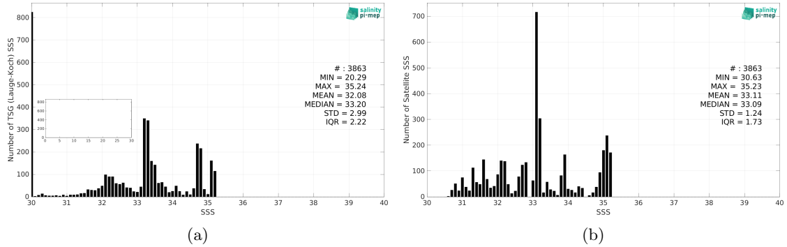
Figure 2: Histograms of SSS from TSG (Lauge-Koch) (a) and SMAP SSS L4 OI v2 - Monthly (IPRC) (b) considering all match-up pairs per bins of 0.1 over the Arctic Ocean Pi-MEP region and for the full satellite product period.
