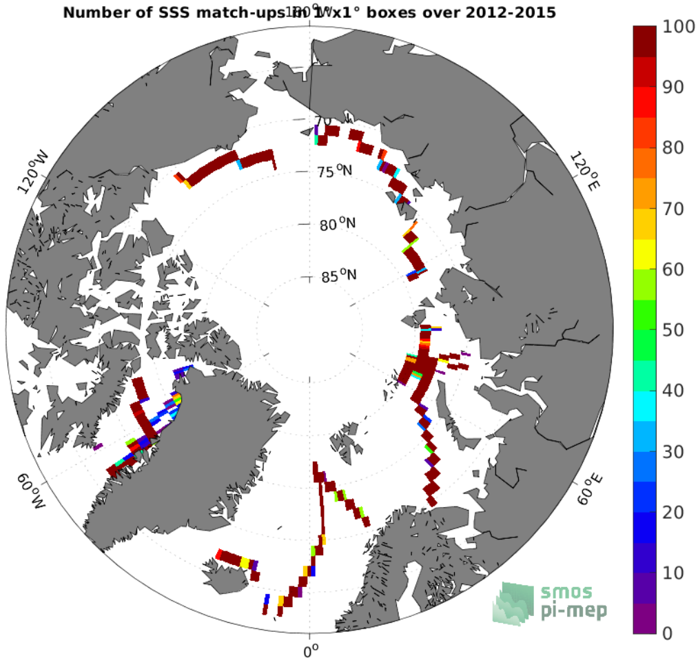
Figure 4: Number of SSS match-ups between TSG (GOSUD-Sailing-ship) SSS and the SMAP SSS L4 OI v2 - Monthly (IPRC) SSS product for the Arctic Ocean Pi-MEP region over 1^\circ \times 1^\circ boxes and for the full satellite product period.
