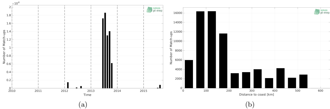
Figure 1: Number of match-ups between TSG (GOSUD-Sailing-ship) and SMAP SSS L4 OI v2 - Monthly (IPRC) SSS as a function of time (a) and as function of the distance to coast (b) over the Arctic Ocean Pi-MEP region and for the full satellite product period.
