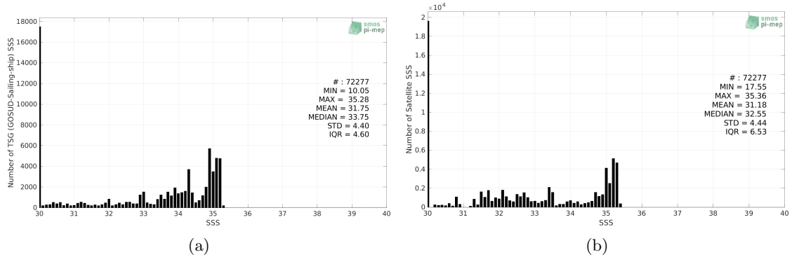
Figure 2: Histograms of SSS from TSG (GOSUD-Sailing-ship) (a) and SMAP SSS L4 OI v2 - Monthly (IPRC) (b) considering all match-up pairs per bins of 0.1 over the Arctic Ocean Pi-MEP region and for the full satellite product period.
