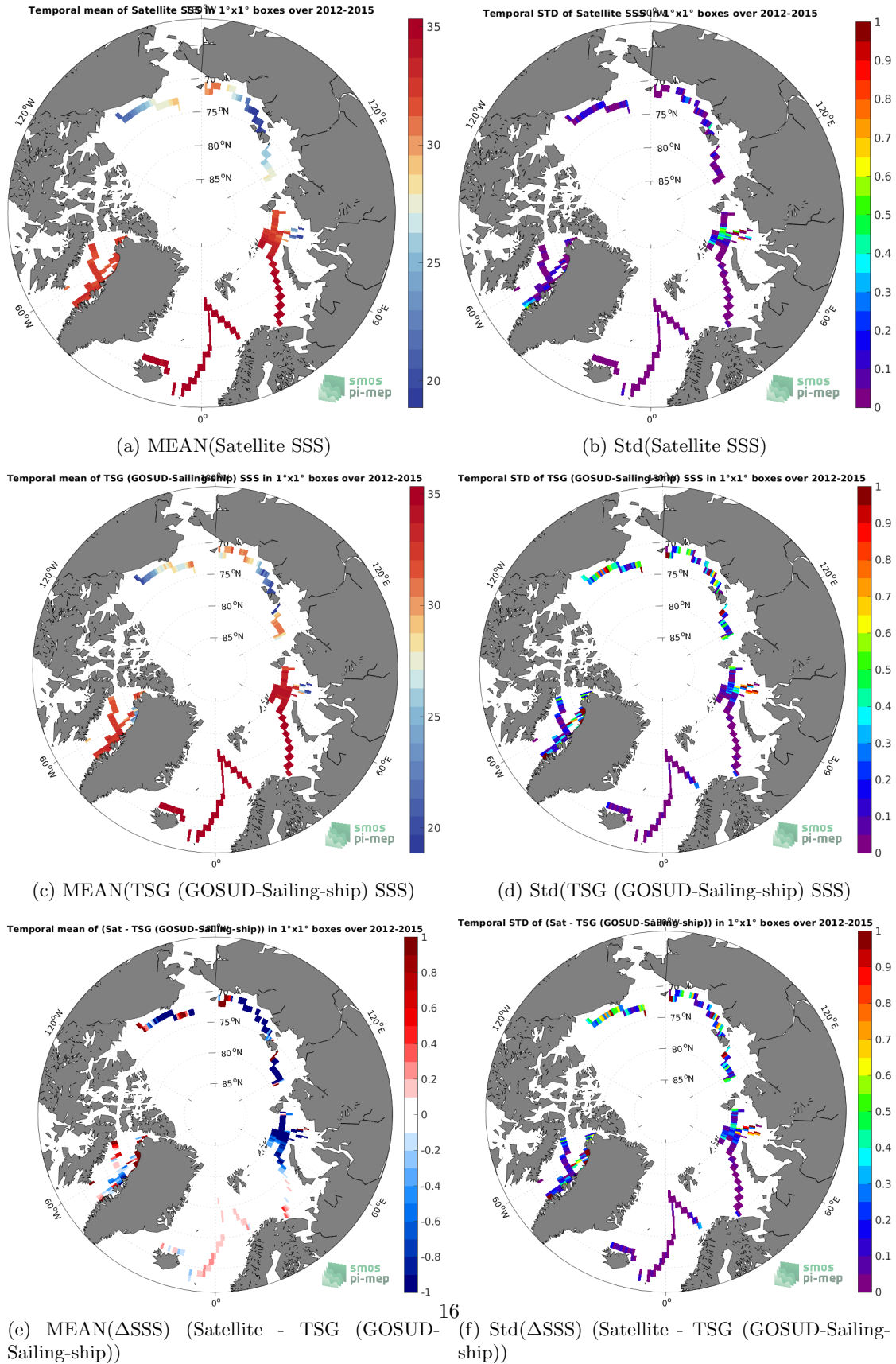
Figure 6: Temporal mean (left) and Std (right) of SSS from SMAP SSS L4 OI v2 - Monthly (IPRC) (top), TSG (GOSUD-Sailing-ship) (middle), and of \Delta SSS (Satellite - TSG (GOSUD-Sailing-ship)). Only match-up pairs are used to generate these maps.
