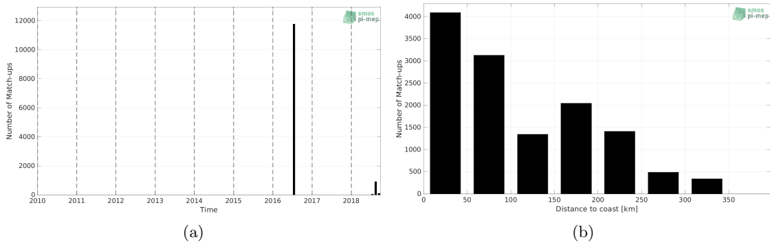
Figure 1: Number of match-ups between TSG (GOSUD-Research-vessel) and SMAP SSS L4 OI v2 - Monthly (IPRC) SSS as a function of time (a) and as function of the distance to coast (b) over the Arctic Ocean Pi-MEP region and for the full satellite product period.
