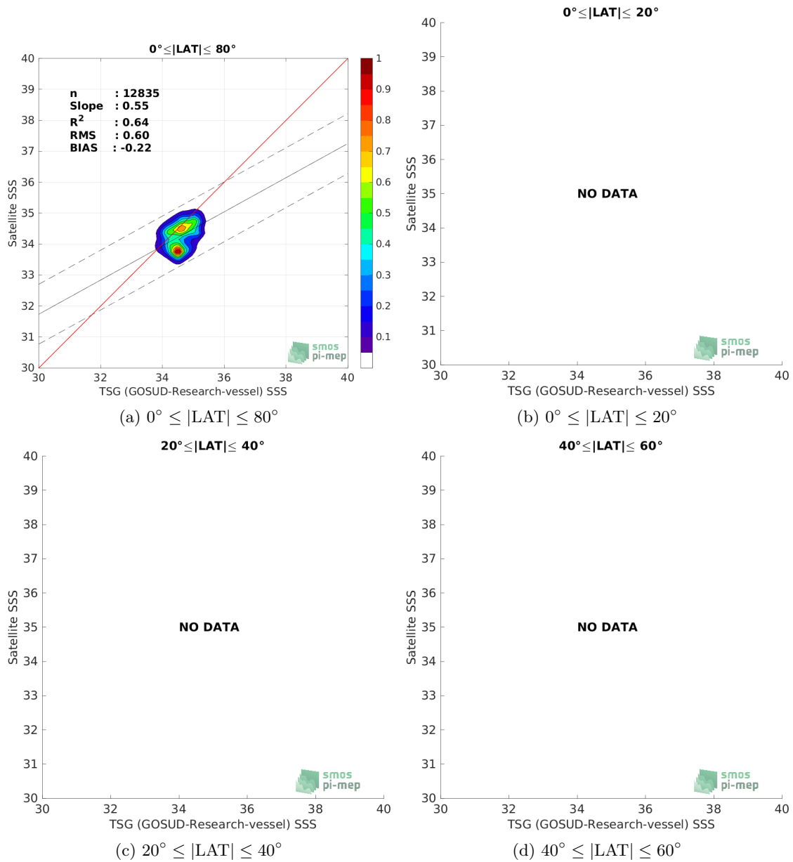
Figure 9: Contour maps of the concentration of SMAP SSS L4 OI v2 - Monthly (IPRC) SSS (y-axis) versus TSG (GOSUD-Research-vessel) SSS (x-axis) at match-up pairs for different latitude bands. For each plot, the red line shows x=y . The black thin and dashed lines indicate a linear fit through the data cloud and the \pm 95\% confidence levels, respectively. The number match-up pairs n , the slope and R^2 coefficient of the linear fit, the root mean square (RMS) and the mean bias between satellite and in situ data are indicated for each latitude band in each plot.
