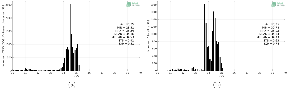
Figure 2: Histograms of SSS from TSG (GOSUD-Research-vessel) (a) and SMAP SSS L4 OI v2 - Monthly (IPRC) (b) considering all match-up pairs per bins of 0.1 over the Arctic Ocean Pi-MEP region and for the full satellite product period.
