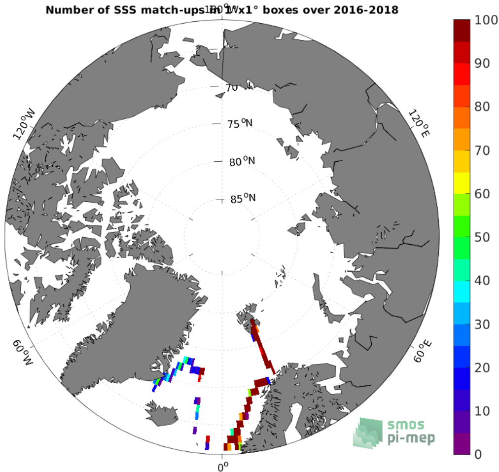
Figure 4: Number of SSS match-ups between TSG (GOSUD-Research-vessel) SSS and the SMAP SSS L4 OI v2 - Monthly (IPRC) SSS product for the Arctic Ocean Pi-MEP region over 1^\circ \times 1^\circ boxes and for the full satellite product period.
