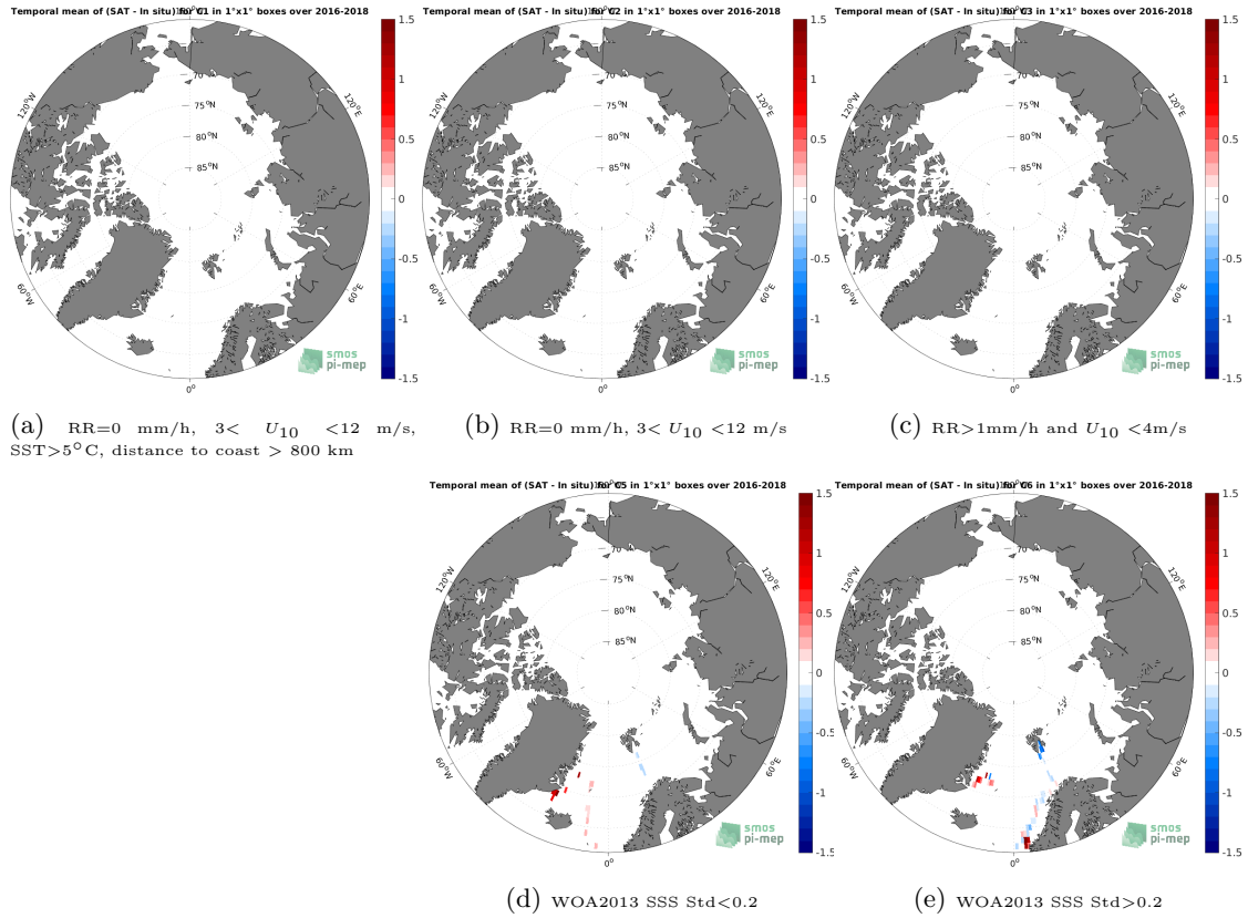
Figure 12: Temporal mean gridded over spatial boxes of size 1^\circ \times 1^\circ of \Delta SSS (SMAP SSS L4 OI v2 - Monthly (IPRC) - TSG (GOSUD-Research-vessel)) for 5 different subdatasets corresponding to: RR=0 mm/h, 3 < U_{10} < 12 m/s, SST>5°C, distance to coast > 800 km (a), RR=0 mm/h, 3 < U_{10} < 12 m/s (b), RR>1mm/h and U_{10} < 4 m/s (c), WOA2013 SSS Std<0.2 (d), WOA2013 SSS Std>0.2 (e).
