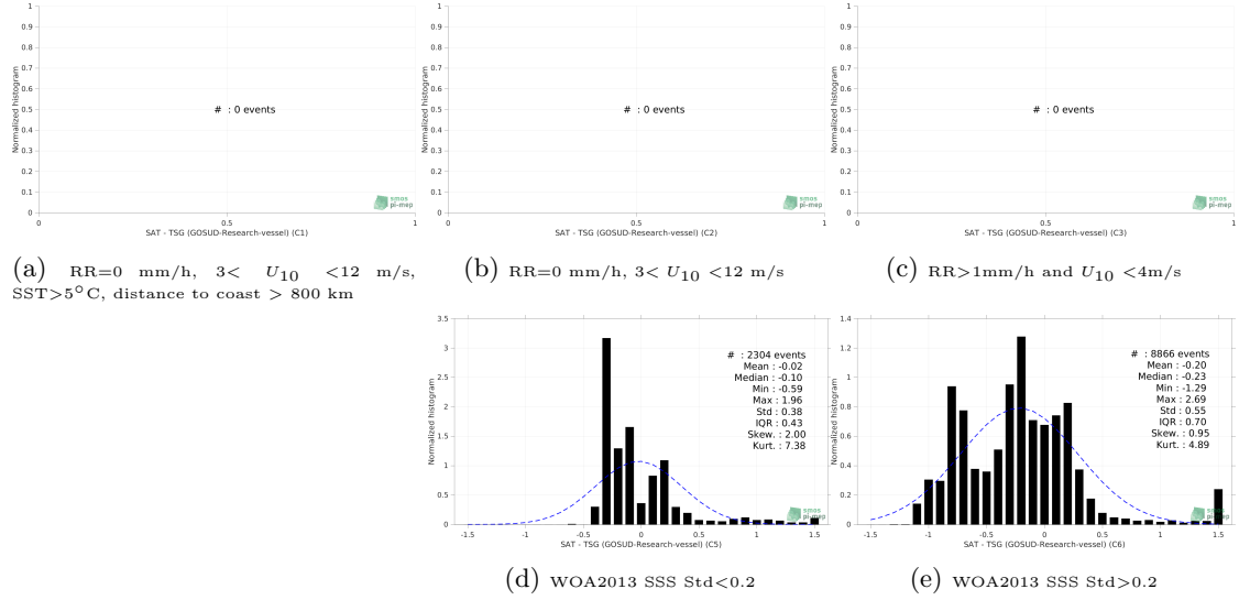
Figure 13: Normalized histogram of \Delta SSS (SMAP SSS L4 OI v2 - Monthly (IPRC) - TSG (GOSUD-Research-vessel)) for 5 different subdatasets corresponding to: RR=0 mm/h, 3 < U_{10} < 12 m/s, SST > 5°C, distance to coast > 800 km (a), RR=0 mm/h, 3 < U_{10} < 12 m/s (b), RR > 1mm/h and U_{10} < 4 m/s (c), WOA2013 SSS Std < 0.2 (d), WOA2013 SSS Std > 0.2 (e).
