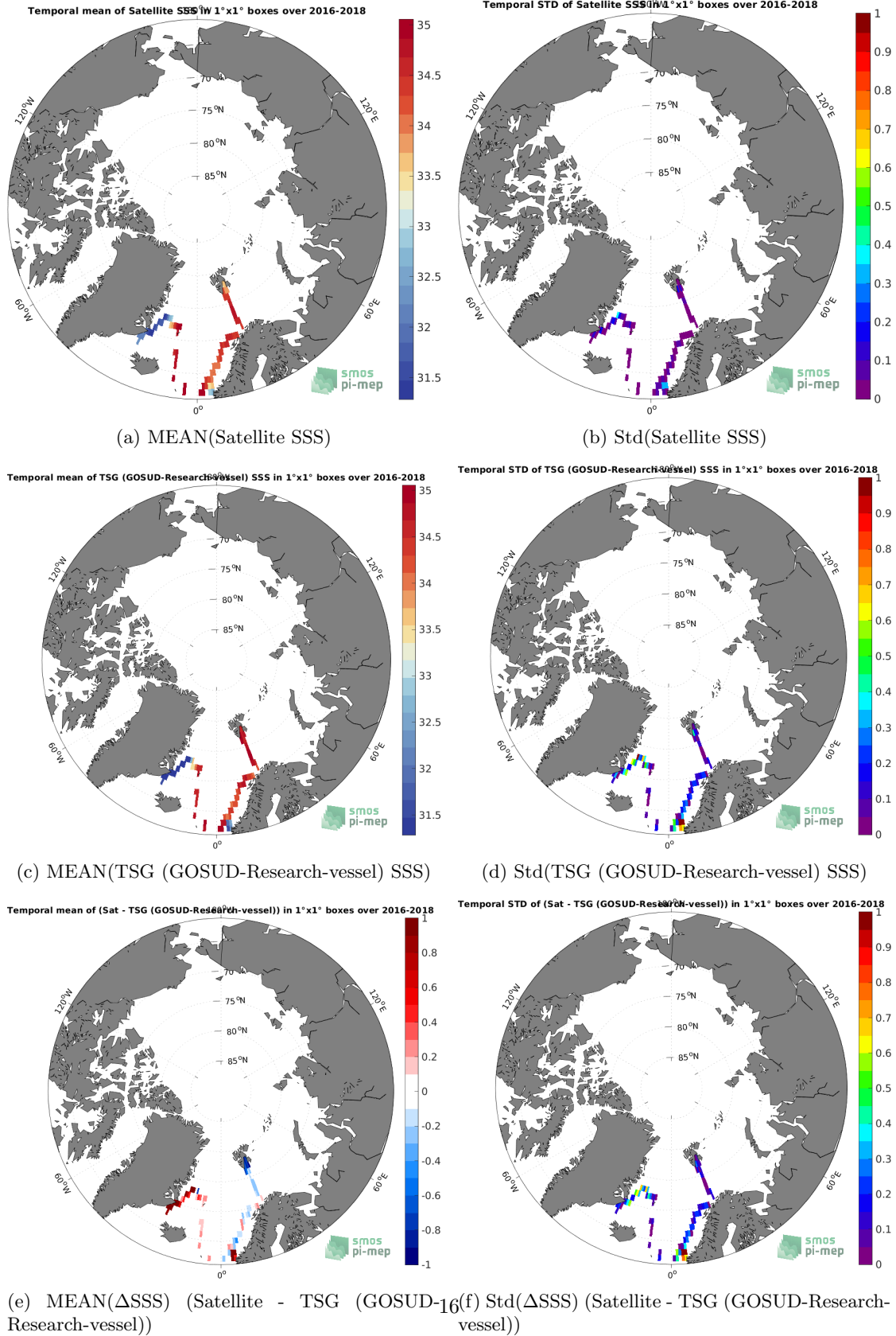
Figure 6: Temporal mean (left) and Std (right) of SSS from SMAP SSS L4 OI v2 - Monthly (IPRC) (top), TSG (GOSUD-Research-vessel) (middle), and of \Delta SSS (Satellite - TSG (GOSUD-Research-vessel)). Only match-up pairs are used to generate these maps.
