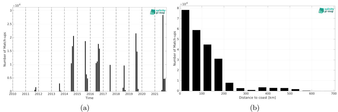
Figure 1: Number of match-ups between TSG (Amundsen) and SMAP SSS L4 OI v2 - Monthly (IPRC) SSS as a function of time (a) and as function of the distance to coast (b) over the Arctic Ocean Pi-MEP region and for the full satellite product period.
