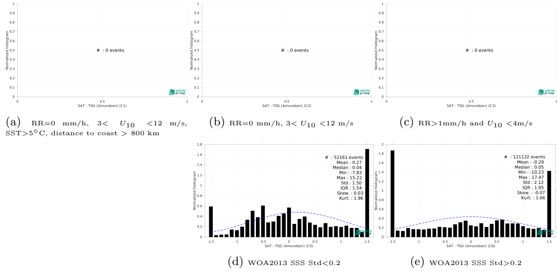
Figure 13: Normalized histogram of \Delta SSS (SMAP SSS L4 OI v2 - Monthly (IPRC) - TSG (Amundsen)) for 5 different subdatasets corresponding to: RR=0 mm/h, 3 < U_{10} < 12 m/s, SST>5°C, distance to coast > 800 km (a), RR=0 mm/h, 3 < U_{10} < 12 m/s (b), RR>1mm/h and U_{10} < 4 m/s (c), WOA2013 SSS Std<0.2 (d), WOA2013 SSS Std>0.2 (e).
