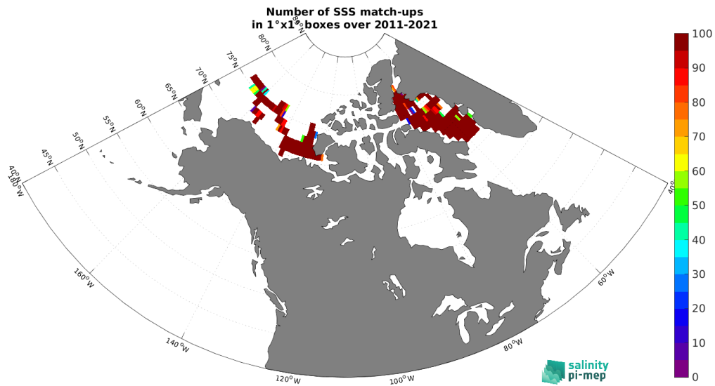
Figure 4: Number of SSS match-ups between TSG (Amundsen) SSS and the SMAP SSS L4 OI v2 - Monthly (IPRC) SSS product for the Arctic Ocean Pi-MEP region over 1^\circ \times 1^\circ boxes and for the full satellite product period.
