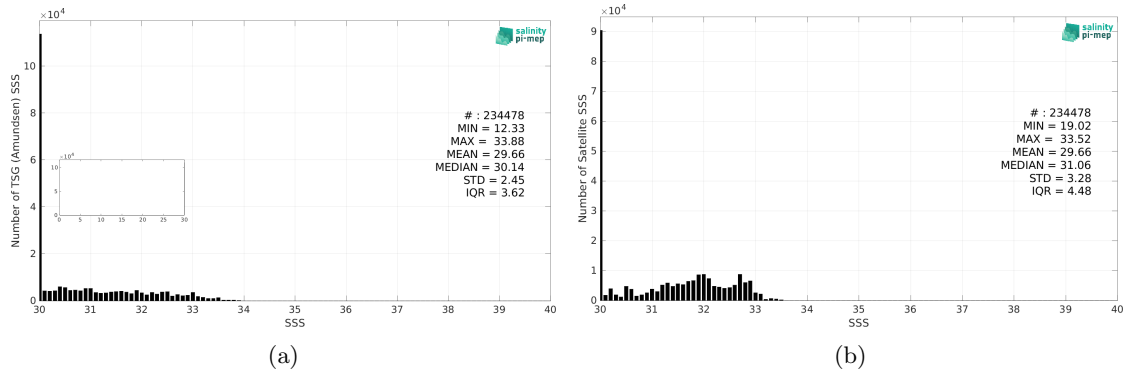
Figure 2: Histograms of SSS from TSG (Amundsen) (a) and SMAP SSS L4 OI v2 - Monthly (IPRC) (b) considering all match-up pairs per bins of 0.1 over the Arctic Ocean Pi-MEP region and for the full satellite product period.
