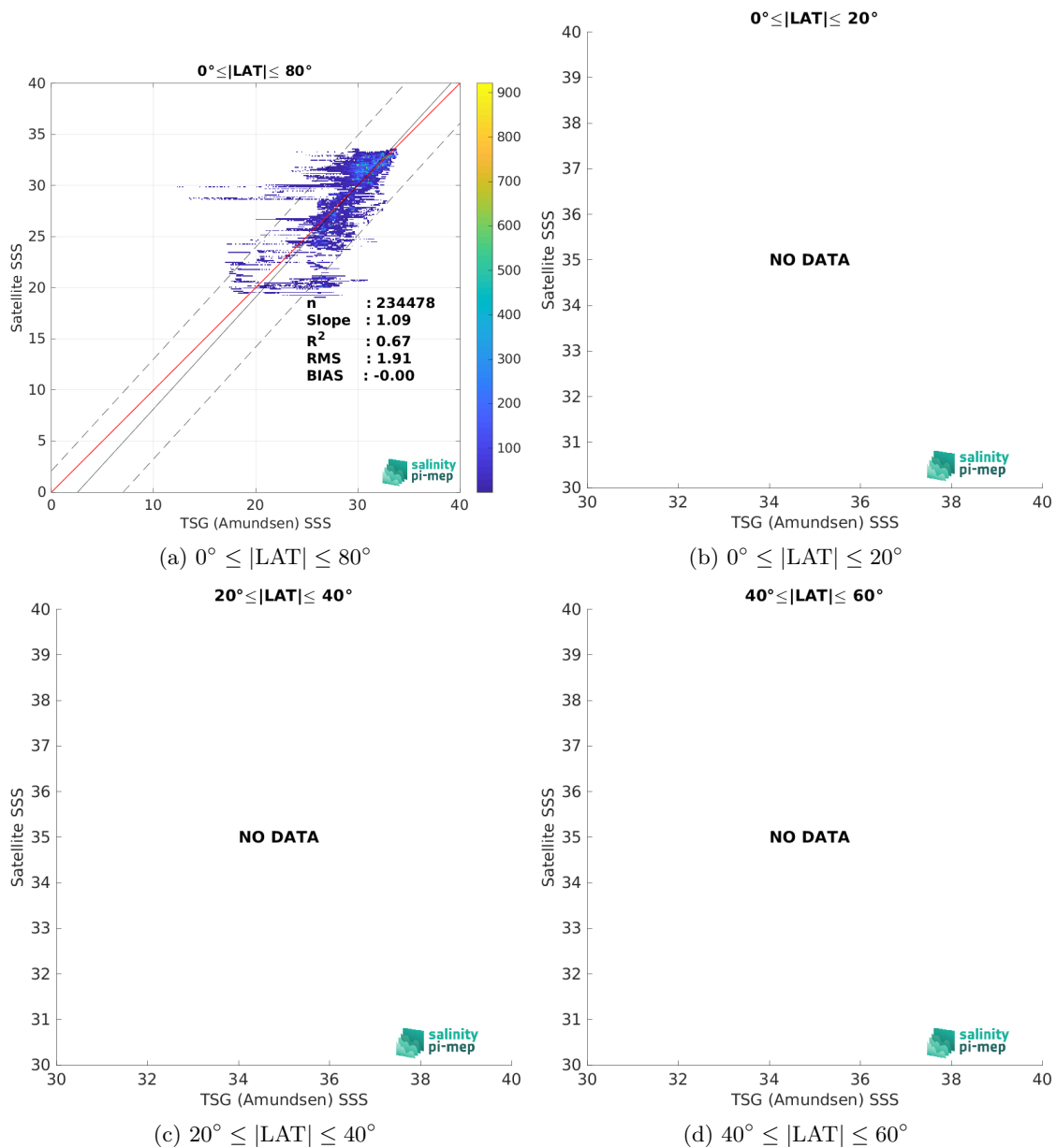
Figure 9: Contour maps of the concentration of SMAP SSS L4 OI v2 - Monthly (IPRC) SSS (y-axis) versus TSG (Amundsen) SSS (x-axis) at match-up pairs for different latitude bands. For each plot, the red line shows x=y . The black thin and dashed lines indicate a linear fit through the data cloud and the \pm 95\% confidence levels, respectively. The number match-up pairs n , the slope and R^2 coefficient of the linear fit, the root mean square (RMS) and the mean bias between satellite and in situ data are indicated for each latitude band in each plots.
