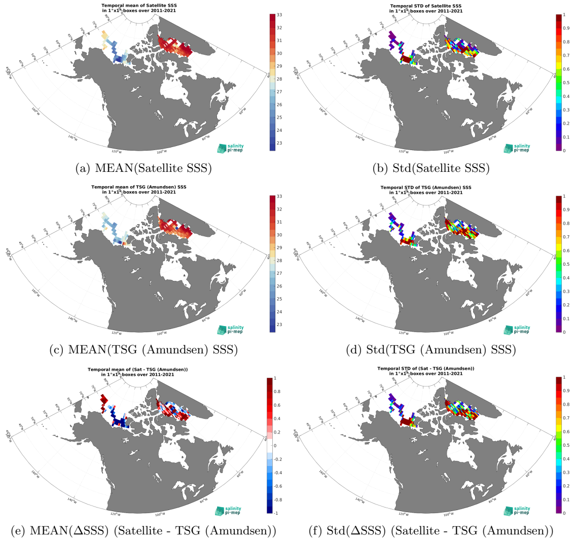
Figure 6: Temporal mean (left) and Std (right) of SSS from SMAP SSS L4 OI v2 - Monthly (IPRC) (top), TSG (Amundsen) (middle), and of \Delta SSS (Satellite - TSG (Amundsen)). Only match-up pairs are used to generate these maps.
