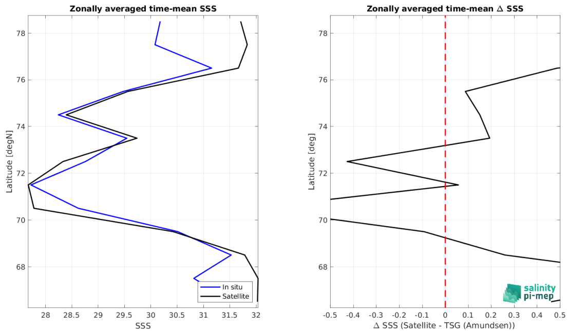
Figure 8: Left panel: Zonal mean SSS from SMAP SSS L4 OI v2 - Monthly (IPRC) satellite product (black) and from TSG (Amundsen) (blue). Right panel: Zonal mean of \Delta SSS (Satellite - TSG (Amundsen)) for all the collected Pi-MEP match-up pairs estimated over the full satellite product period.
