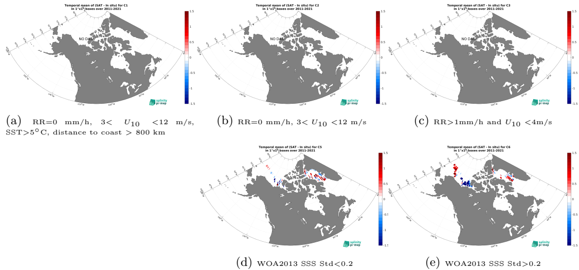
Figure 12: Temporal mean gridded over spatial boxes of size 1^{\circ}\times 1^{\circ} of \Delta\text{SSS} (SMAP SSS L4 OI v2 - Monthly (IPRC) - TSG (Amundsen)) for 5 different subdatasets corresponding to:RR=0 mm/h, 3 < U_{10} < 12 m/s, SST >5^{\circ}\text{C} , distance to coast > 800 km (a), RR=0 mm/h, 3 < U_{10} < 12 m/s (b), RR >1 mm/h and U_{10} < 4 m/s (c), WOA2013 SSS Std <0.2 (d), WOA2013 SSS Std >0.2 (e).
