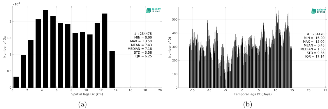
Figure 5: Histograms of the spatial (a) and temporal (b) lags between the location/time of the TSG (Amundsen) measurement and the date of the corresponding SMAP SSS L4 OI v2 - Monthly (IPRC) SSS pixel.
