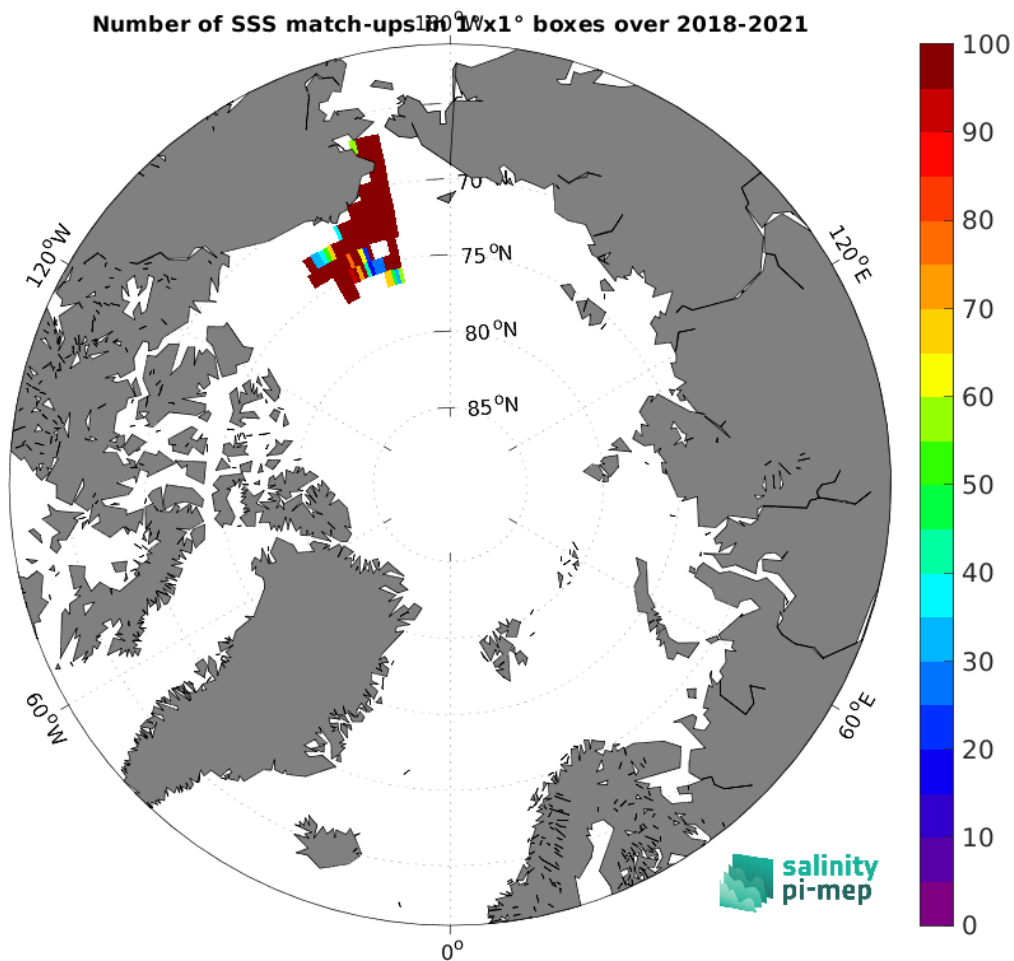
Figure 4: Number of SSS match-ups between Saildrone SSS and the SMAP SSS L4 OI v2 - Monthly (IPRC) SSS product for the Arctic Ocean Pi-MEP region over 1^{\circ} \times 1^{\circ} boxes and for the full satellite product period.
