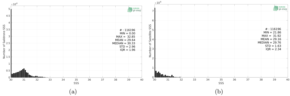
Figure 2: Histograms of SSS from Saildrone (a) and SMAP SSS L4 OI v2 - Monthly (IPRC) (b) considering all match-up pairs per bins of 0.1 over the Arctic Ocean Pi-MEP region and for the full satellite product period.
