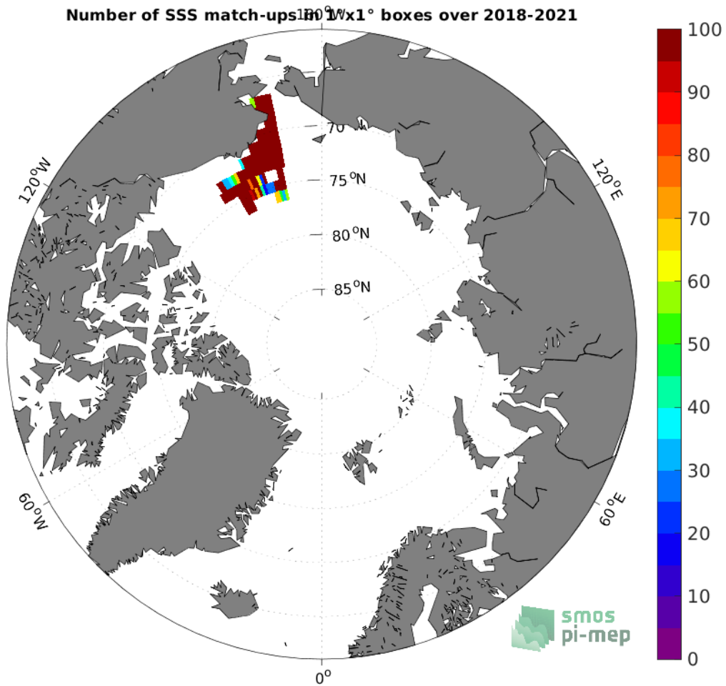
Figure 4: Number of SSS match-ups between Sairdrone SSS and the SMAP SSS L4 OI v2 - Monthly (IPRC) SSS product for the Arctic Ocean Pi-MEP region over 1^{\circ} \times 1^{\circ} boxes and for the full satellite product period.
