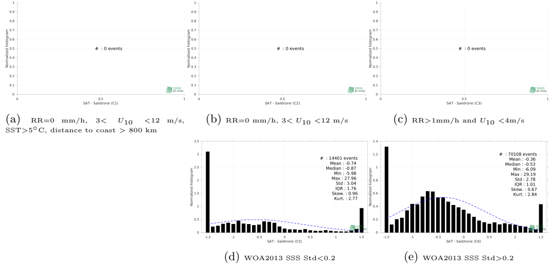
Figure 13: Normalized histogram of \Delta SSS (SMAP SSS L4 OI v2 - Monthly (IPRC) - Sairdrone) for 5 different subdatasets corresponding to: RR=0 mm/h, 3 < U_{10} < 12 m/s, SST>5°C, distance to coast > 800 km (a), RR=0 mm/h, 3 < U_{10} < 12 m/s (b), RR>1mm/h and U_{10} < 4 m/s (c), WOA2013 SSS Std<0.2 (d), WOA2013 SSS Std>0.2 (e).
