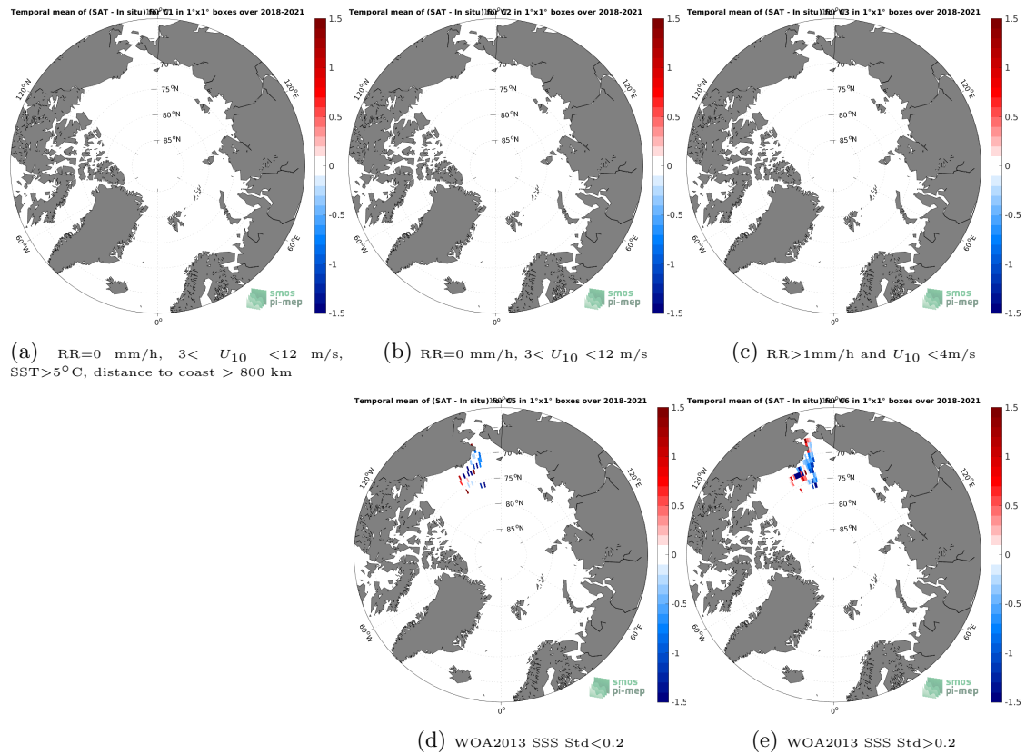
Figure 12: Temporal mean gridded over spatial boxes of size 1^{\circ}\times 1^{\circ} of \Delta\text{SSS} (SMAP SSS L4 OI v2 - Monthly (IPRC) - Saildrone) for 5 different subdatasets corresponding to:RR=0 mm/h, 3 < U_{10} < 12 m/s, SST > 5^{\circ}\text{C} , distance to coast > 800 km (a), RR=0 mm/h, 3 < U_{10} < 12 m/s (b), RR > 1 mm/h and U_{10} < 4 m/s (c), WOA2013 SSS Std < 0.2 (d), WOA2013 SSS Std > 0.2 (e).
