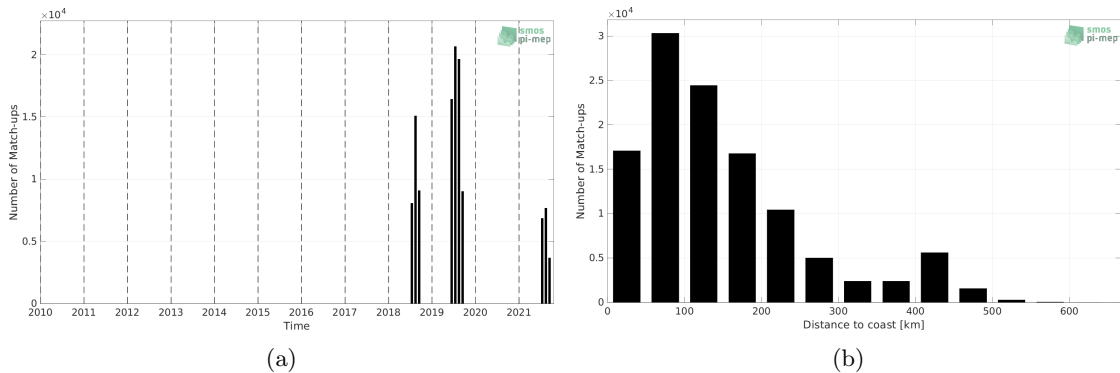
Figure 1: Number of match-ups between Saildrone and SMAP SSS L4 OI v2 - Monthly (IPRC) SSS as a function of time (a) and as function of the distance to coast (b) over the Arctic Ocean Pi-MEP region and for the full satellite product period.
