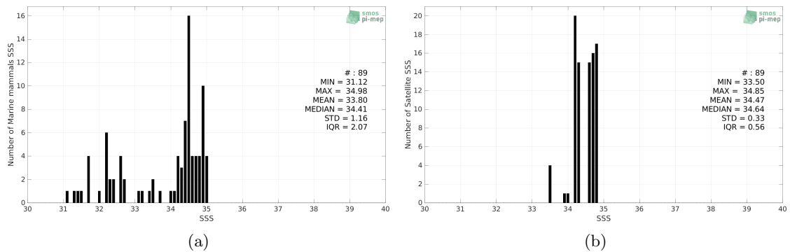
Figure 2: Histograms of SSS from Marine mammals (a) and SMAP SSS L4 OI v2 - Monthly (IPRC) (b) considering all match-up pairs per bins of 0.1 over the Arctic Ocean Pi-MEP region and for the full satellite product period.
