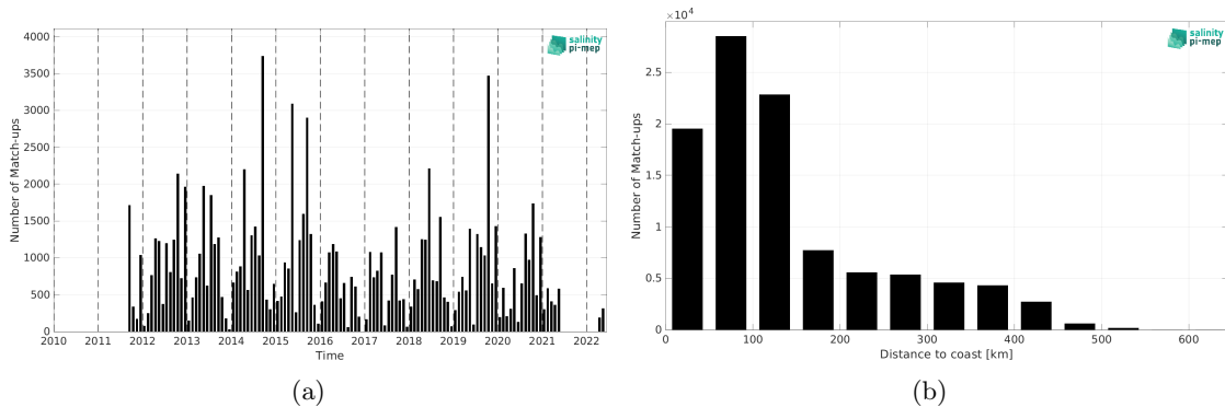
Figure 1: Number of match-ups between ICES and SMAP SSS L4 OI v2 - Monthly (IPRC) SSS as a function of time (a) and as function of the distance to coast (b) over the Arctic Ocean Pi-MEP region and for the full satellite product period.
