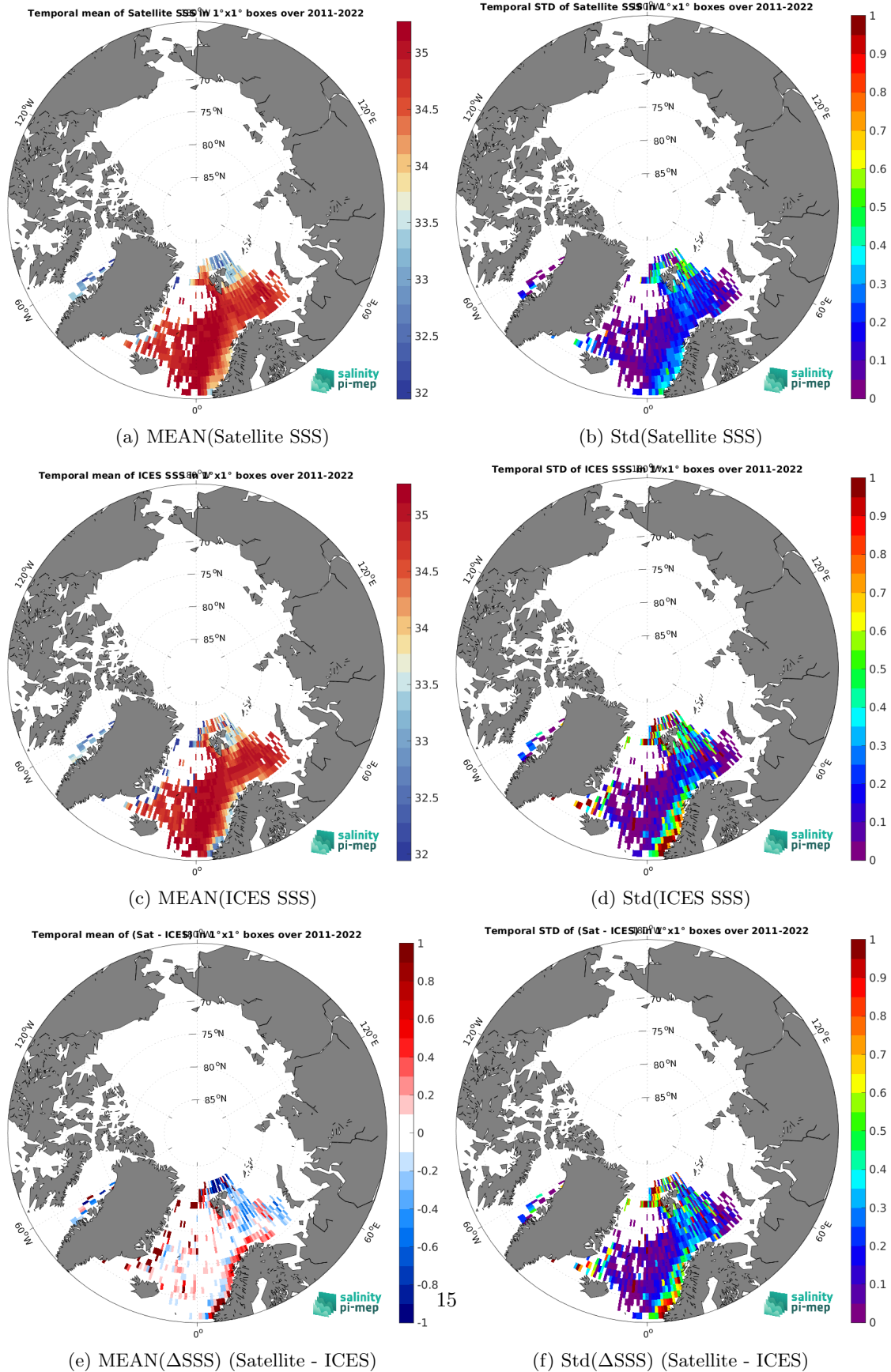
Figure 6: Temporal mean (left) and Std (right) of SSS from SMAP SSS L4 OI v2 - Monthly (IPRC) (top), ICES (middle), and of \Delta SSS (Satellite - ICES). Only match-up pairs are used to generate these maps.
