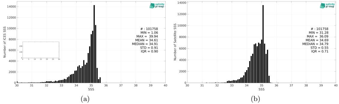
Figure 2: Histograms of SSS from ICES (a) and SMAP SSS L4 OI v2 - Monthly (IPRC) (b) considering all match-up pairs per bins of 0.1 over the Arctic Ocean Pi-MEP region and for the full satellite product period.
