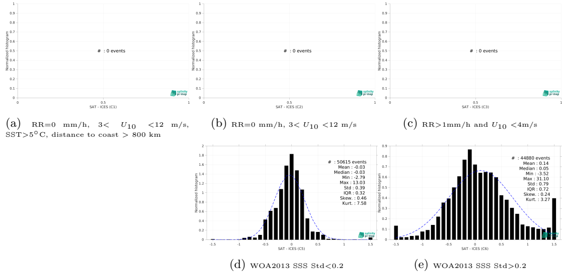
Figure 13: Normalized histogram of \Delta SSS (SMAP SSS L4 OI v2 - Monthly (IPRC) - ICES) for 5 different subdatasets corresponding to: RR=0 mm/h, 3 < U_{10} < 12 m/s, SST>5°C, distance to coast > 800 km (a), RR=0 mm/h, 3 < U_{10} < 12 m/s (b), RR>1mm/h and U_{10} < 4 m/s (c), WOA2013 SSS Std<0.2 (d), WOA2013 SSS Std>0.2 (e).
