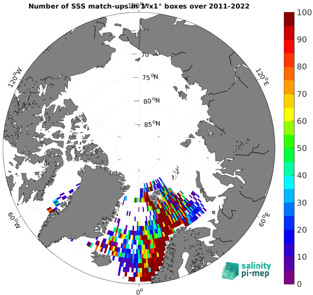
Figure 4: Number of SSS match-ups between ICES SSS and the SMAP SSS L4 OI v2 - Monthly (IPRC) SSS product for the Arctic Ocean Pi-MEP region over 1^\circ \times 1^\circ boxes and for the full satellite product period.
