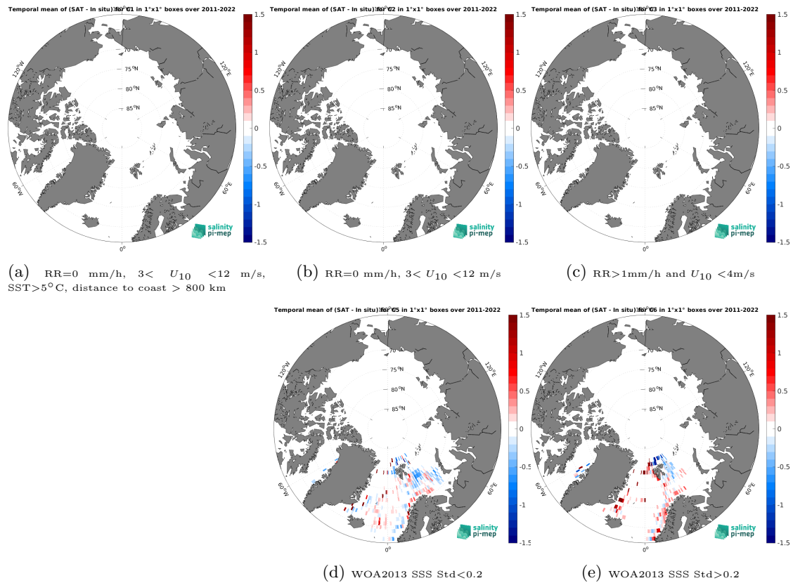
Figure 12: Temporal mean gridded over spatial boxes of size 1^{\circ}\times 1^{\circ} of \Delta\text{SSS} (SMAP SSS L4 OI v2 - Monthly (IPRC) - ICES) for 5 different subdatasets corresponding to: RR=0 mm/h, 3 < U_{10} < 12 m/s, SST > 5^{\circ}\text{C} , distance to coast > 800 km (a), RR=0 mm/h, 3 < U_{10} < 12 m/s (b), RR > 1 mm/h and U_{10} < 4 m/s (c), WOA2013 SSS Std < 0.2 (d), WOA2013 SSS Std > 0.2 (e).
