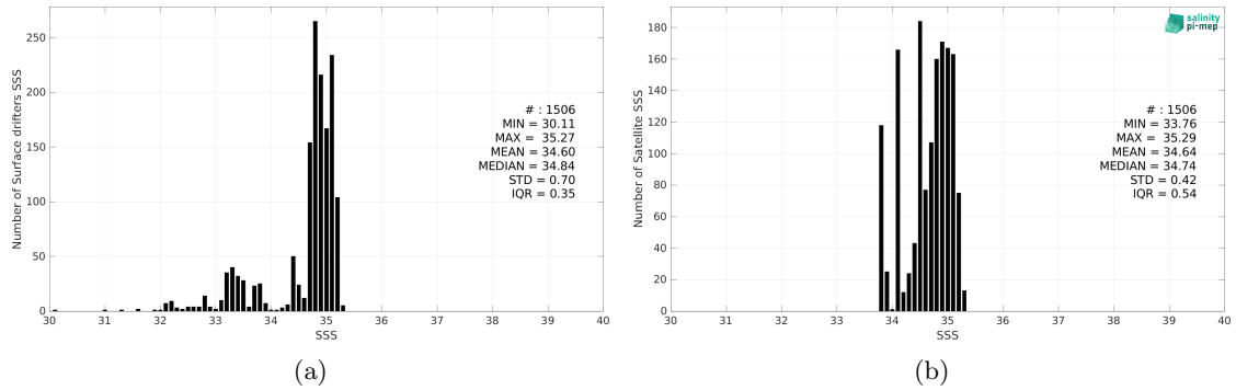
Figure 2: Histograms of SSS from Surface drifters (a) and SMAP SSS L4 OI v2 - Monthly (IPRC) (b) considering all match-up pairs per bins of 0.1 over the Arctic Ocean Pi-MEP region and for the full satellite product period.
