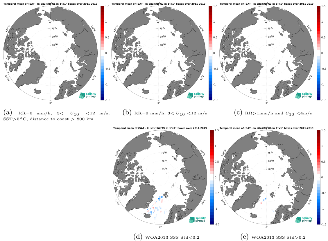
Figure 11: Temporal mean gridded over spatial boxes of size 1^{\circ}\times 1^{\circ} of \Delta\text{SSS} (SMAP SSS L4 OI v2 - Monthly (IPRC) - Surface drifters) for 5 different subdatasets corresponding to:RR=0 mm/h, 3 < U_{10} < 12 m/s, SST > 5^{\circ}\text{C} , distance to coast > 800 km (a), RR=0 mm/h, 3 < U_{10} < 12 m/s (b), RR > 1 mm/h and U_{10} < 4 m/s (c), WOA2013 SSS Std < 0.2 (d), WOA2013 SSS Std > 0.2 (e).
