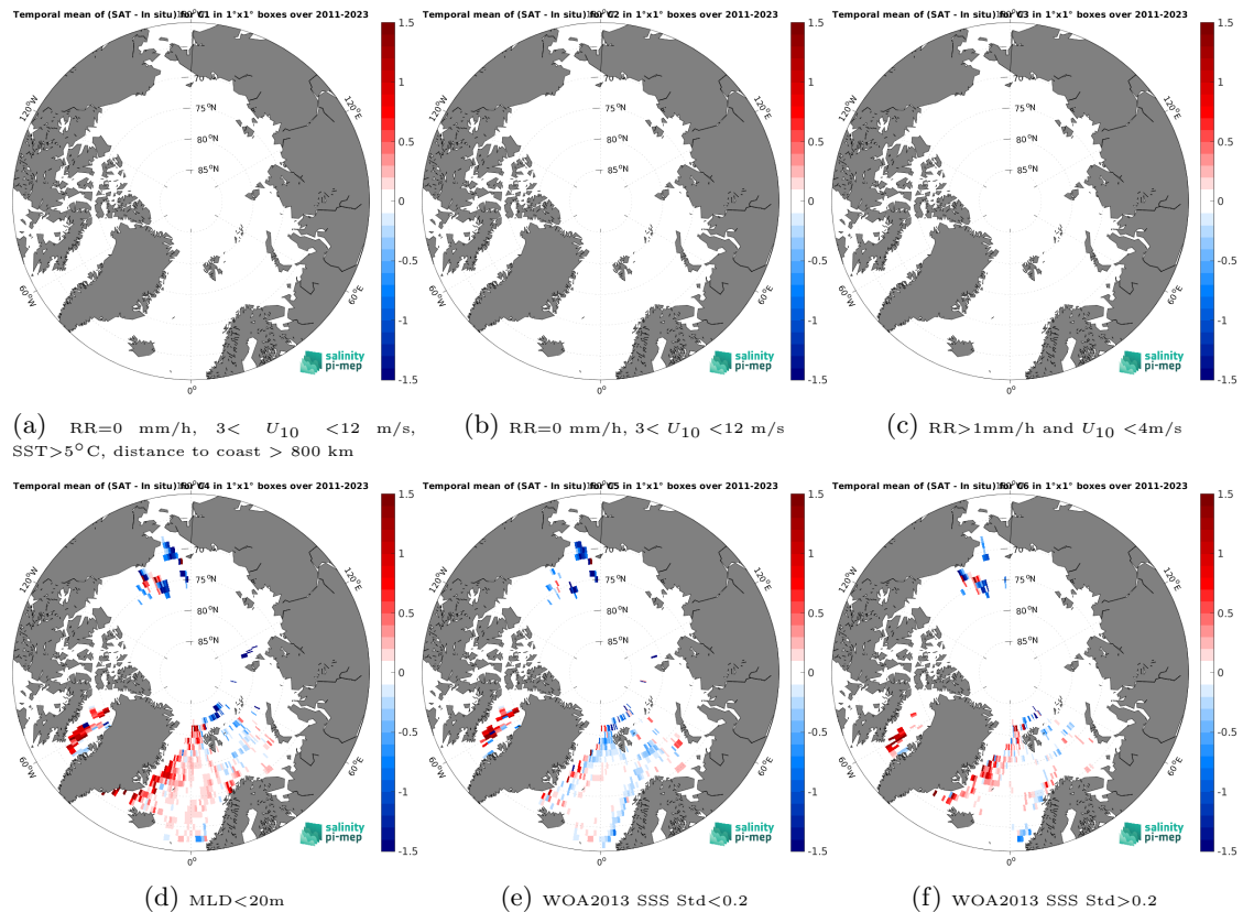
Figure 12: Temporal mean gridded over spatial boxes of size 1^{\circ}\times 1^{\circ} of \Delta\text{SSS} (SMAP SSS L4 OI v2 - Monthly (IPRC) - Argo) for 6 different subdatasets corresponding to:RR=0 mm/h, 3 < U_{10} < 12 m/s, SST >5^{\circ}\text{C} , distance to coast > 800 km (a), RR=0 mm/h, 3 < U_{10} < 12 m/s (b), RR >1 mm/h and U_{10} < 4 m/s (c),MLD <20 m (d),WOA2013 SSS Std <0.2 (e),WOA2013 SSS Std >0.2 (f).
