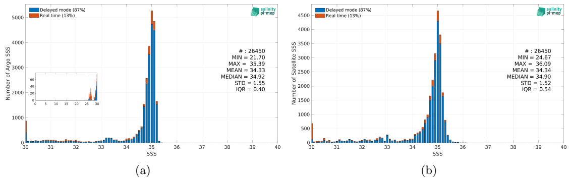
Figure 2: Histograms of SSS from Argo (a) and SMAP SSS L4 OI v2 - Monthly (IPRC) (b) considering all match-up pairs per bins of 0.1 over the Arctic Ocean Pi-MEP region and for the full satellite product period.
