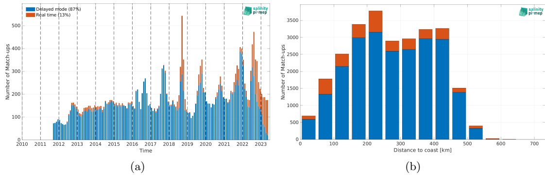
Figure 1: Number of match-ups between Argo and SMAP SSS L4 OI v2 - Monthly (IPRC) SSS as a function of time (a) and as function of the distance to coast (b) over the Arctic Ocean Pi-MEP region and for the full satellite product period.
