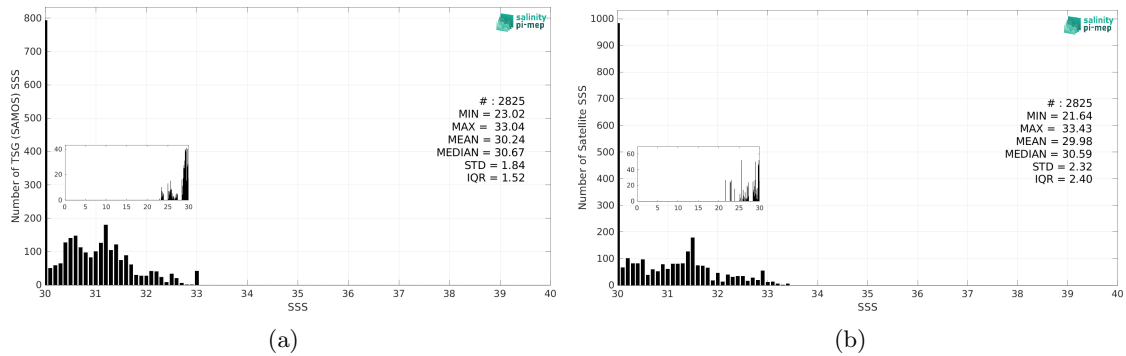
Figure 3: Histograms of SSS from TSG (SAMOS) (a) and SMAP SSS L3 v6 - 8-Day running (RSS) (b) considering all match-up pairs per bins of 0.1 over the Arctic Ocean Pi-MEP region and for the full satellite product period.
