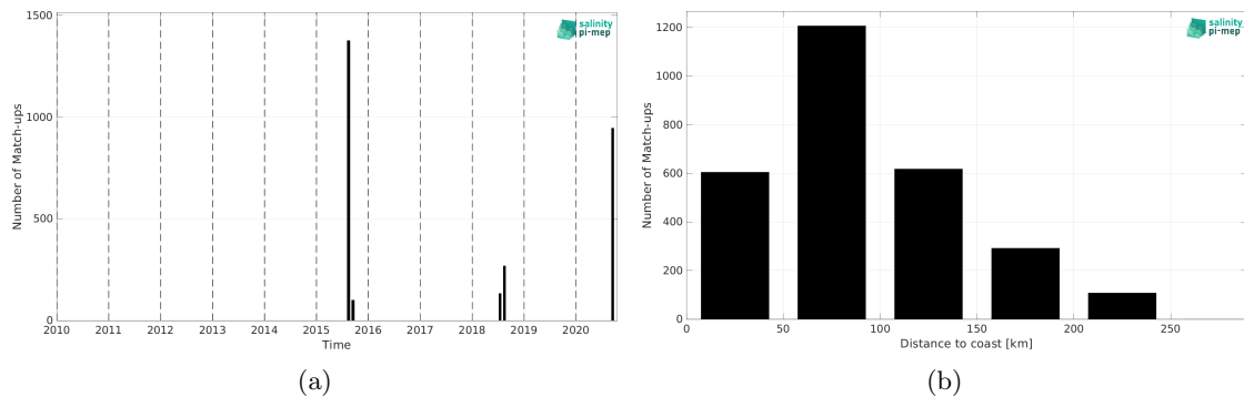
Figure 2: Number of match-ups between TSG (SAMOS) and SMAP SSS L3 v6 - 8-Day running (RSS) SSS as a function of time (a) and as function of the distance to coast (b) over the Arctic Ocean Pi-MEP region and for the full satellite product period.
