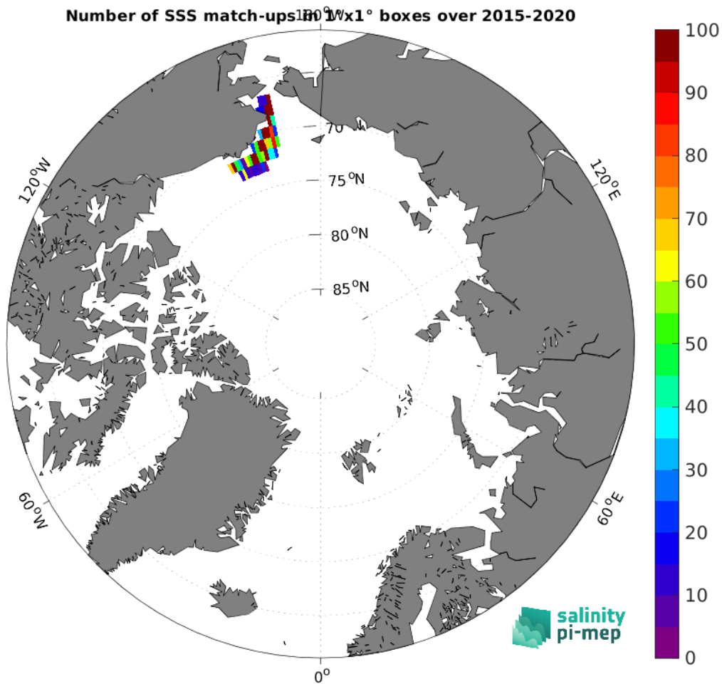
Figure 5: Number of SSS match-ups between TSG (SAMOS) SSS and the SMAP SSS L3 v6 - 8-Day running (RSS) SSS product for the Arctic Ocean Pi-MEP region over 1^\circ \times 1^\circ boxes and for the full satellite product period.
