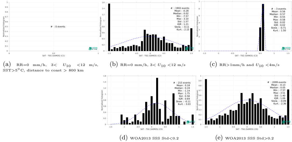
Figure 15: Normalized histogram of \Delta\text{SSS} (SMAP SSS L3 v6 - 8-Day running (RSS) - TSG (SAMOS)) for 5 different subdatasets corresponding to: RR=0 mm/h, 3 < U_{10} < 12 m/s, SST >5^{\circ}\text{C} , distance to coast > 800 km (a), RR=0 mm/h, 3 < U_{10} < 12 m/s (b), RR>1\text{mm/h} and U_{10} < 4\text{m/s} (c), WOA2013 SSS Std <0.2 (d), WOA2013 SSS Std >0.2 (e).
