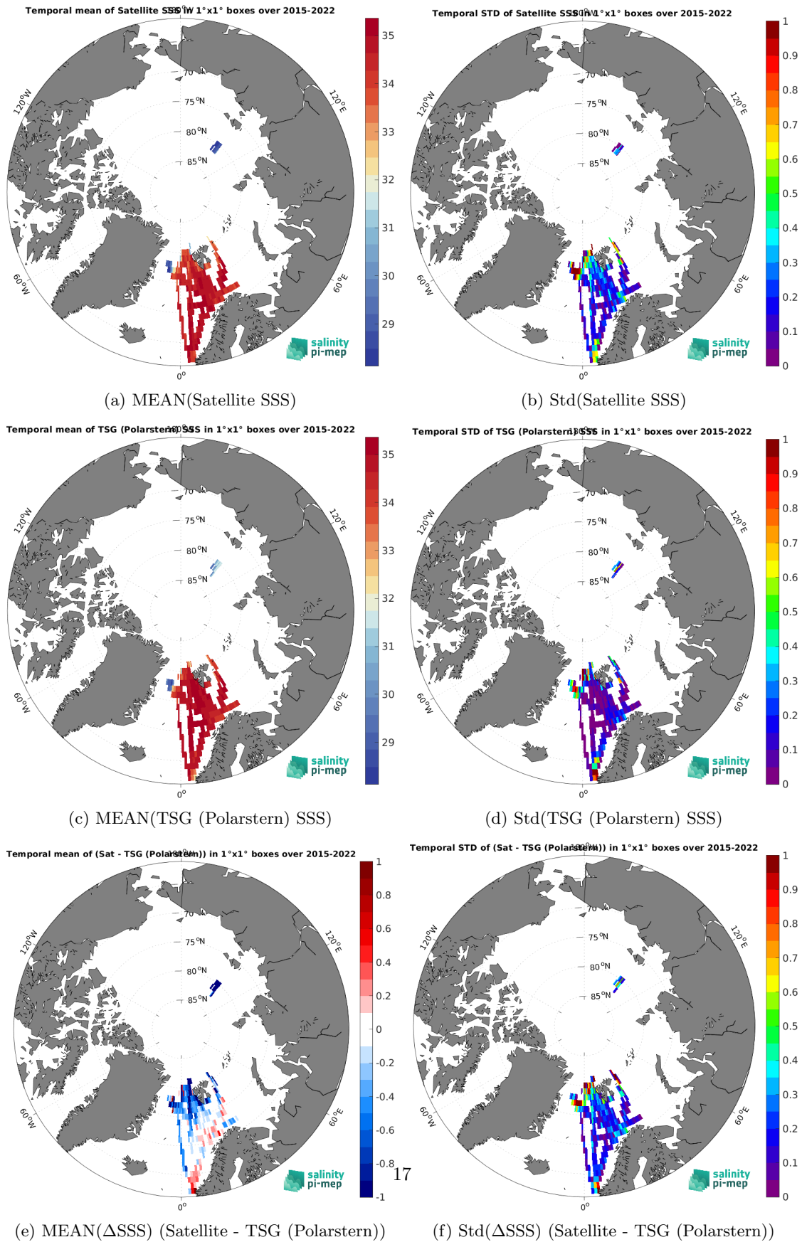
Figure 7: Temporal mean (left) and Std (right) of SSS from SMAP SSS L3 v6 - 8-Day running (RSS) (top), TSG (Polarstern) (middle), and of \Delta SSS (Satellite - TSG (Polarstern)). Only match-up pairs are used to generate these maps.
