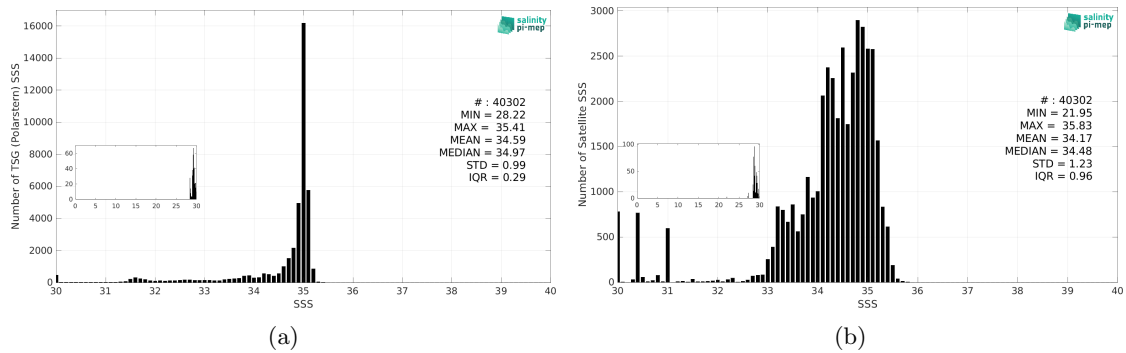
Figure 3: Histograms of SSS from TSG (Polarstern) (a) and SMAP SSS L3 v6 - 8-Day running (RSS) (b) considering all match-up pairs per bins of 0.1 over the Arctic Ocean Pi-MEP region and for the full satellite product period.
