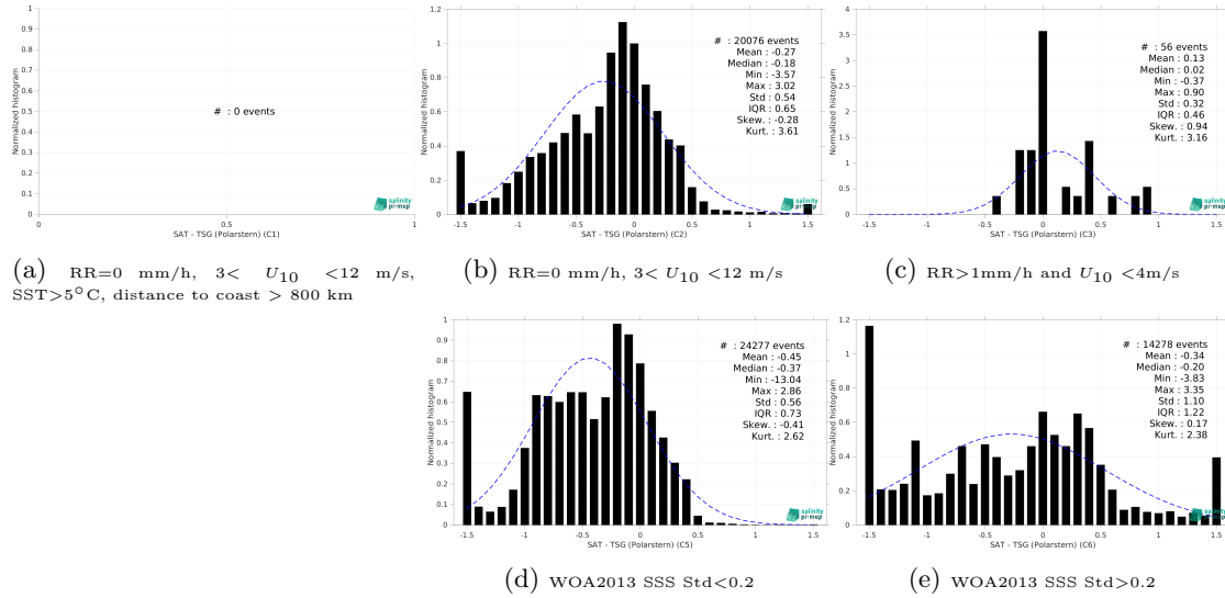
Figure 15: Normalized histogram of \Delta SSS (SMAP SSS L3 v6 - 8-Day running (RSS) - TSG (Polarstern)) for 5 different subdatasets corresponding to: RR=0 mm/h, 3 < U_{10} < 12 m/s, SST > 5°C, distance to coast > 800 km (a), RR=0 mm/h, 3 < U_{10} < 12 m/s (b), RR > 1mm/h and U_{10} < 4 m/s (c), WOA2013 SSS Std < 0.2 (d), WOA2013 SSS Std > 0.2 (e).
