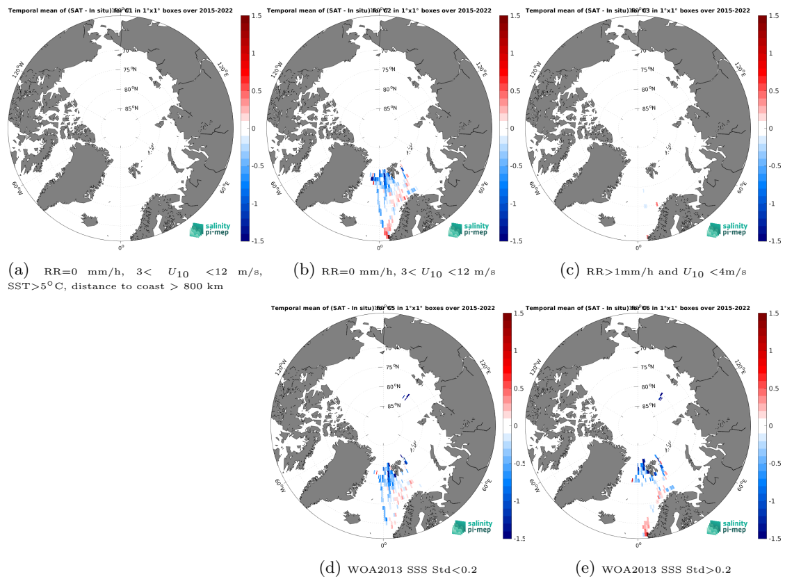
Figure 14: Temporal mean gridded over spatial boxes of size 1^\circ \times 1^\circ of \Delta SSS (SMAP SSS L3 v6 - 8-Day running (RSS) - TSG (Polarstern)) for 5 different subdatasets corresponding to: RR=0 mm/h, 3 < U_{10} < 12 m/s, SST > 5°C, distance to coast > 800 km (a), RR=0 mm/h, 3 < U_{10} < 12 m/s (b), RR > 1mm/h and U_{10} < 4 m/s (c), WOA2013 SSS Std < 0.2 (d), WOA2013 SSS Std > 0.2 (e).
