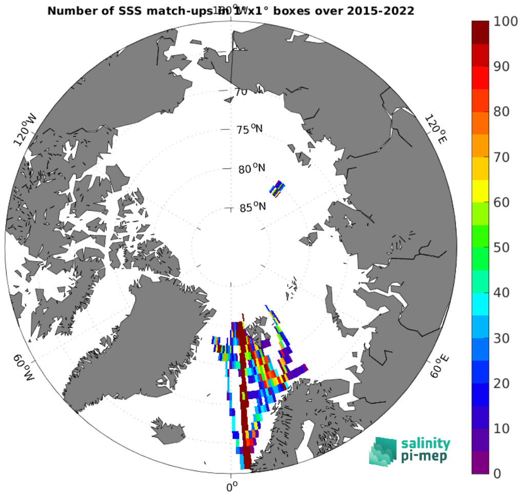
Figure 5: Number of SSS match-ups between TSG (Polarstern) SSS and the SMAP SSS L3 v6 - 8-Day running (RSS) SSS product for the Arctic Ocean Pi-MEP region over 1^\circ \times 1^\circ boxes and for the full satellite product period.
