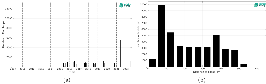
Figure 2: Number of match-ups between TSG (Polarstern) and SMAP SSS L3 v6 - 8-Day running (RSS) SSS as a function of time (a) and as function of the distance to coast (b) over the Arctic Ocean Pi-MEP region and for the full satellite product period.
