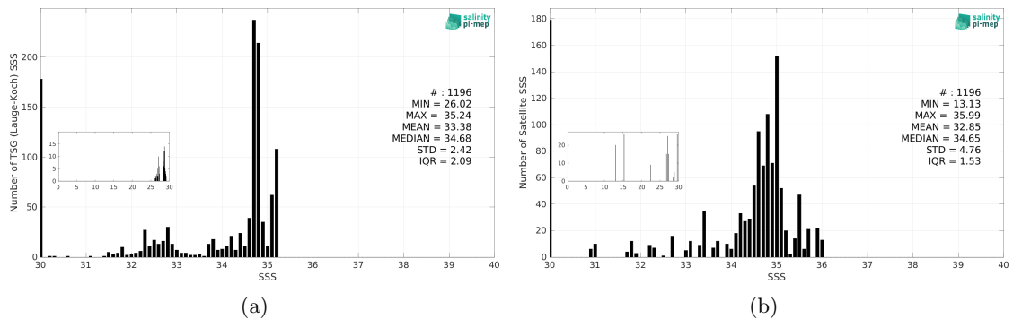
Figure 3: Histograms of SSS from TSG (Lauge-Koch) (a) and SMAP SSS L3 v6 - 8-Day running (RSS) (b) considering all match-up pairs per bins of 0.1 over the Arctic Ocean Pi-MEP region and for the full satellite product period.
