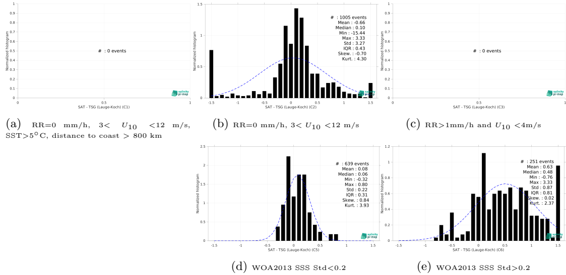
Figure 15: Normalized histogram of \Delta SSS (SMAP SSS L3 v6 - 8-Day running (RSS) - TSG (Lauge-Koch)) for 5 different subdatasets corresponding to: RR=0 mm/h, 3 < U_{10} < 12 m/s, SST >5^{\circ}\text{C} , distance to coast > 800 km (a), RR=0 mm/h, 3 < U_{10} < 12 m/s (b), RR >1 mm/h and U_{10} < 4 m/s (c), WOA2013 SSS Std <0.2 (d), WOA2013 SSS Std >0.2 (e).
