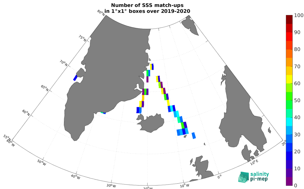
Figure 5: Number of SSS match-ups between TSG (Lauge-Koch) SSS and the SMAP SSS L3 v6 - 8-Day running (RSS) SSS product for the Arctic Ocean Pi-MEP region over 1^\circ \times 1^\circ boxes and for the full satellite product period.
