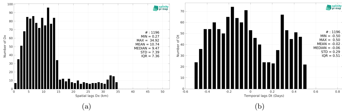
Figure 6: Histograms of the spatial (a) and temporal (b) lags between the location/time of the TSG (Lauge-Koch) measurement and the date of the corresponding SMAP SSS L3 v6 - 8-Day running (RSS) SSS pixel.
