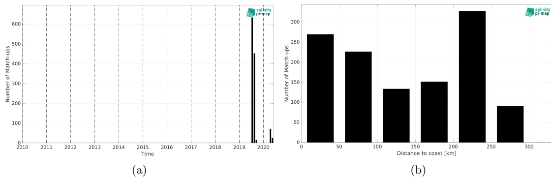
Figure 2: Number of match-ups between TSG (Lauge-Koch) and SMAP SSS L3 v6 - 8-Day running (RSS) SSS as a function of time (a) and as function of the distance to coast (b) over the Arctic Ocean Pi-MEP region and for the full satellite product period.
