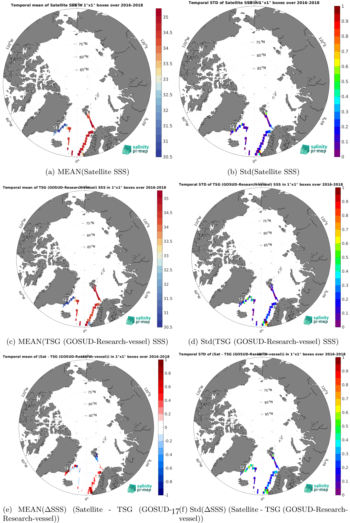
Figure 7: Temporal mean (left) and Std (right) of SSS from SMAP SSS L3 v6 - 8-Day running (RSS) (top), TSG (GOSUD-Research-vessel) (middle), and of \Delta SSS (Satellite - TSG (GOSUD-Research-vessel)). Only match-up pairs are used to generate these maps.
