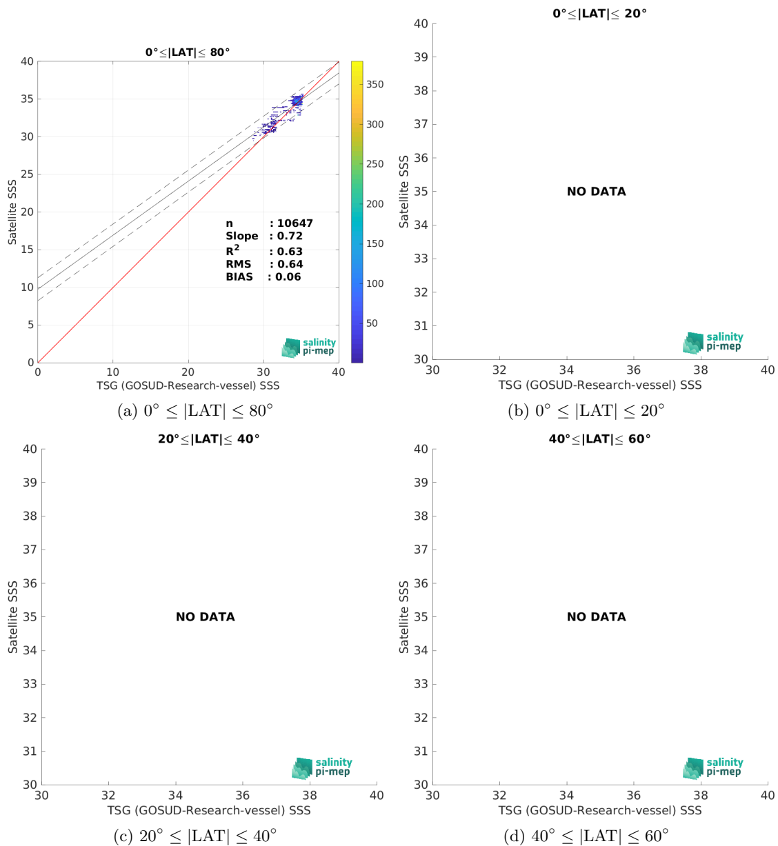
Figure 10: Contour maps of the concentration of SMAP SSS L3 v6 - 8-Day running (RSS) SSS (y-axis) versus TSG (GOSUD-Research-vessel) SSS (x-axis) at match-up pairs for different latitude bands. For each plot, the red line shows x=y . The black thin and dashed lines indicate a linear fit through the data cloud and the \pm 95\% confidence levels, respectively. The number match-up pairs n , the slope and R^2 coefficient of the linear fit, the root mean square (RMS) and the mean bias between satellite and in situ data are indicated for each latitude band in each plots.
