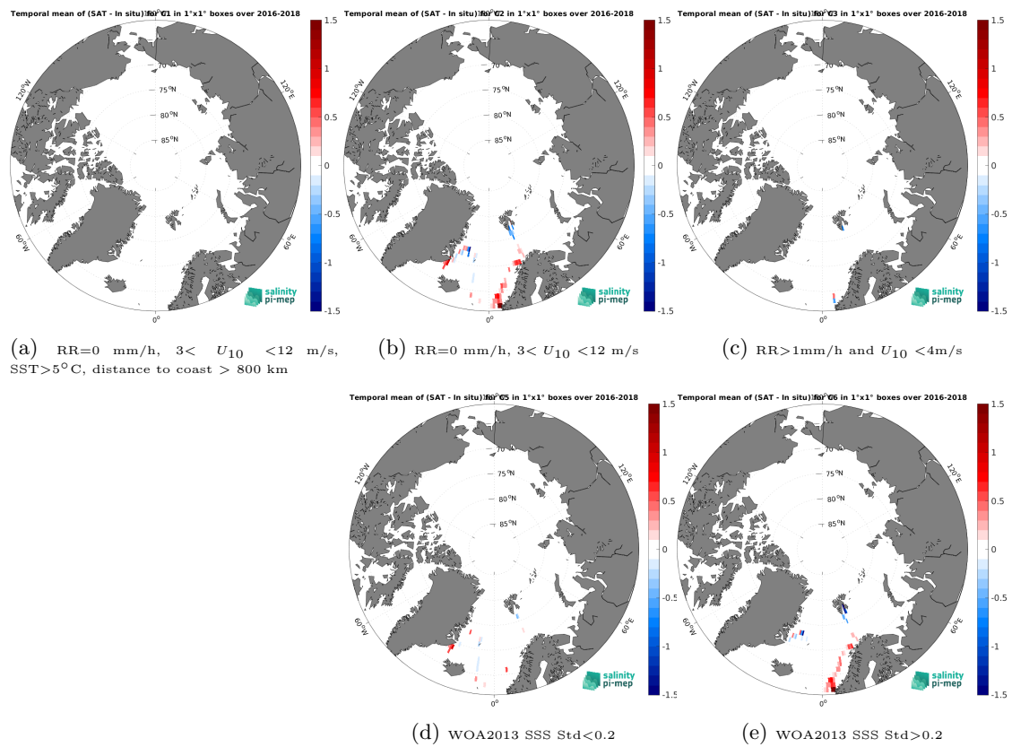
Figure 14: Temporal mean gridded over spatial boxes of size 1^\circ \times 1^\circ of \Delta SSS (SMAP SSS L3 v6 - 8-Day running (RSS) - TSG (GOSUD-Research-vessel)) for 5 different subdatasets corresponding to:RR=0 mm/h, 3 < U_{10} < 12 m/s, SST >5^\circ C, distance to coast > 800 km (a), RR=0 mm/h, 3 < U_{10} < 12 m/s (b), RR >1 mm/h and U_{10} < 4 m/s (c), WOA2013 SSS Std <0.2 (d), WOA2013 SSS Std >0.2 (e).
