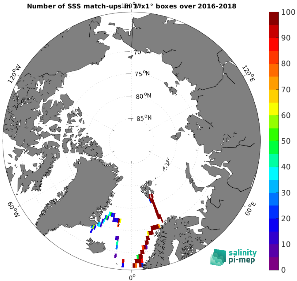
Figure 5: Number of SSS match-ups between TSG (GOSUD-Research-vessel) SSS and the SMAP SSS L3 v6 - 8-Day running (RSS) SSS product for the Arctic Ocean Pi-MEP region over 1^\circ \times 1^\circ boxes and for the full satellite product period.
