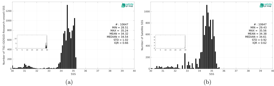
Figure 3: Histograms of SSS from TSG (GOSUD-Research-vessel) (a) and SMAP SSS L3 v6 - 8-Day running (RSS) (b) considering all match-up pairs per bins of 0.1 over the Arctic Ocean Pi-MEP region and for the full satellite product period.
