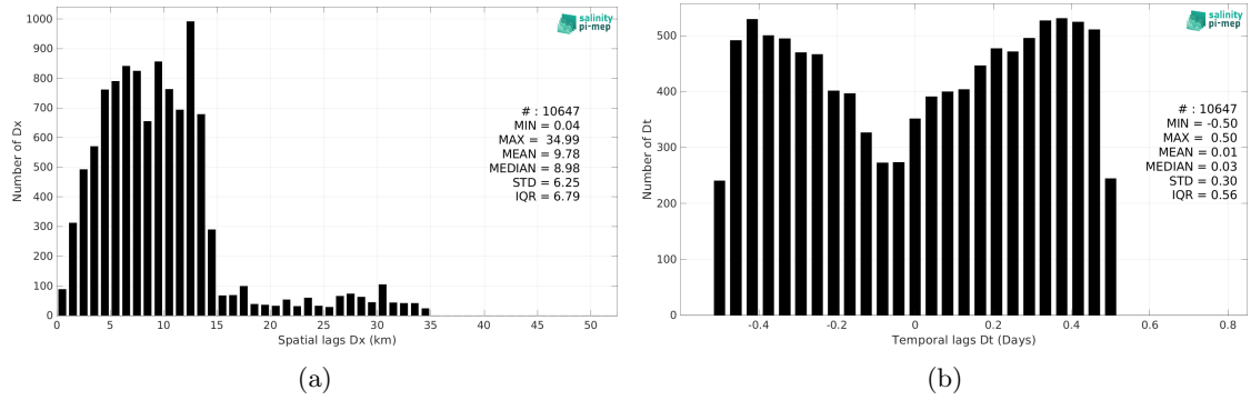
Figure 6: Histograms of the spatial (a) and temporal (b) lags between the location/time of the TSG (GOSUD-Research-vessel) measurement and the date of the corresponding SMAP SSS L3 v6 - 8-Day running (RSS) SSS pixel.
