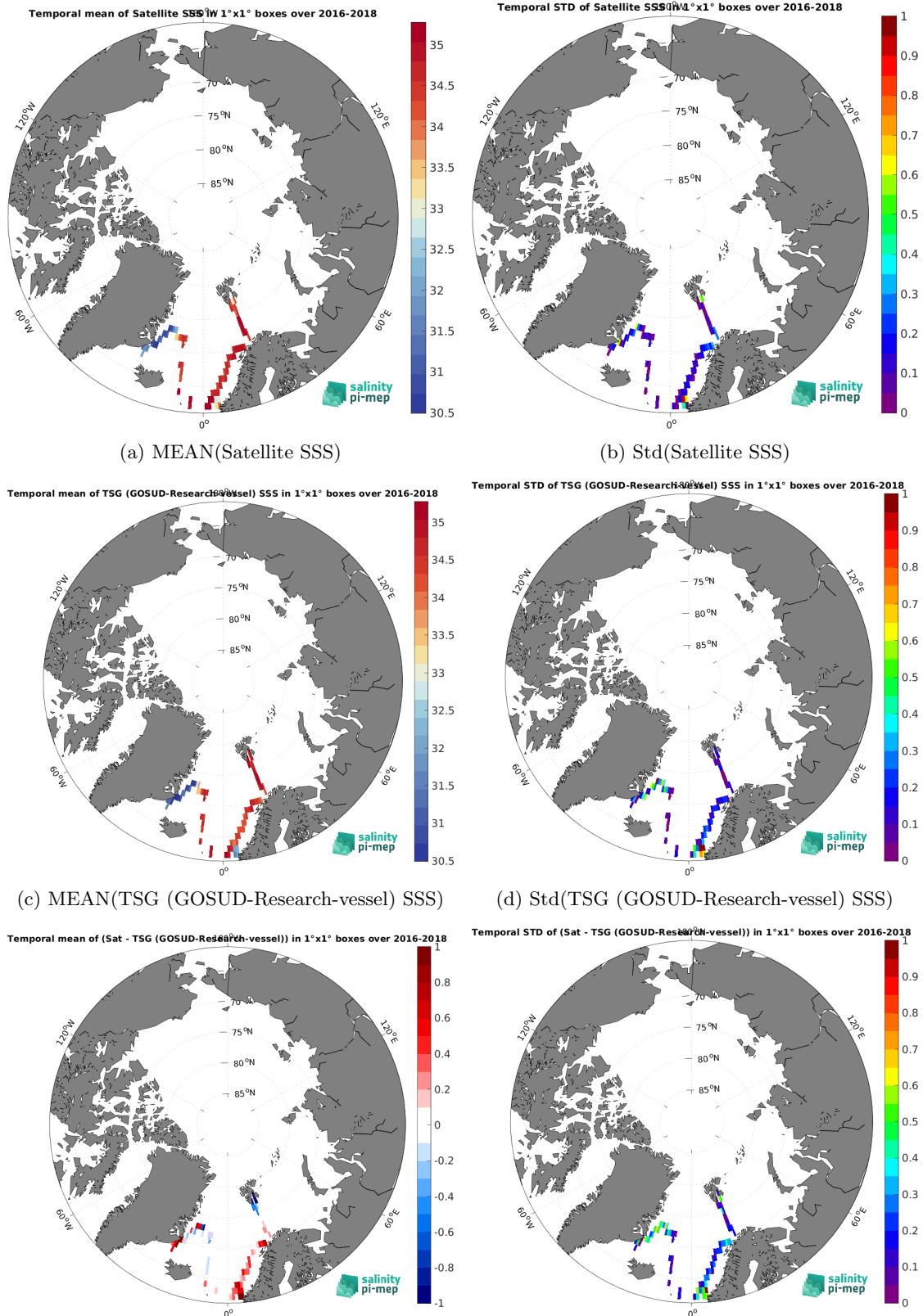
(e) MEAN( \Delta SSS) (Satellite - TSG (GOSUD-Research-vessel))
