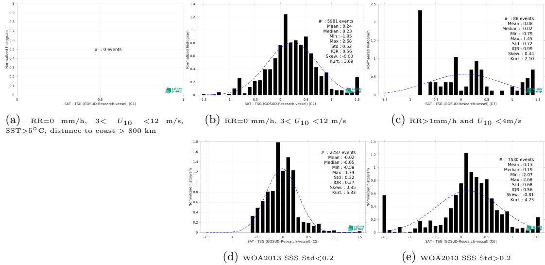
Figure 15: Normalized histogram of \Delta SSS (SMAP SSS L3 v6 - 8-Day running (RSS) - TSG (GOSUD-Research-vessel)) for 5 different subdatasets corresponding to: RR=0 mm/h, 3 < U_{10} < 12 m/s, SST > 5°C, distance to coast > 800 km (a), RR=0 mm/h, 3 < U_{10} < 12 m/s (b), RR > 1mm/h and U_{10} < 4 m/s (c), WOA2013 SSS Std < 0.2 (d), WOA2013 SSS Std > 0.2 (e).
