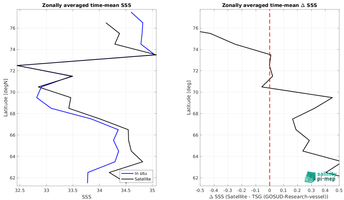
Figure 9: Left panel: Zonal mean SSS from SMAP SSS L3 v6 - 8-Day running (RSS) satellite product (black) and from TSG (GOSUD-Research-vessel) (blue). Right panel: Zonal mean of \Delta SSS (Satellite - TSG (GOSUD-Research-vessel)) for all the collected Pi-MEP match-up pairs estimated over the full satellite product period.
