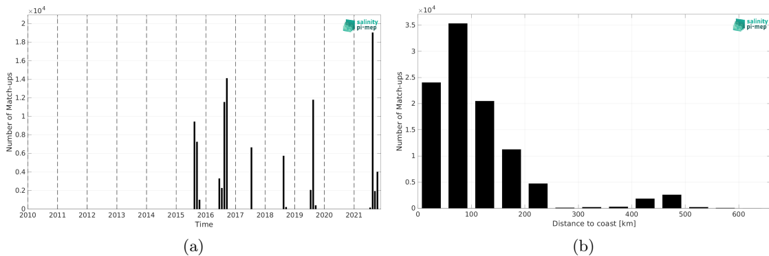
Figure 2: Number of match-ups between TSG (Amundsen) and SMAP SSS L3 v6 - 8-Day running (RSS) SSS as a function of time (a) and as function of the distance to coast (b) over the Arctic Ocean Pi-MEP region and for the full satellite product period.
