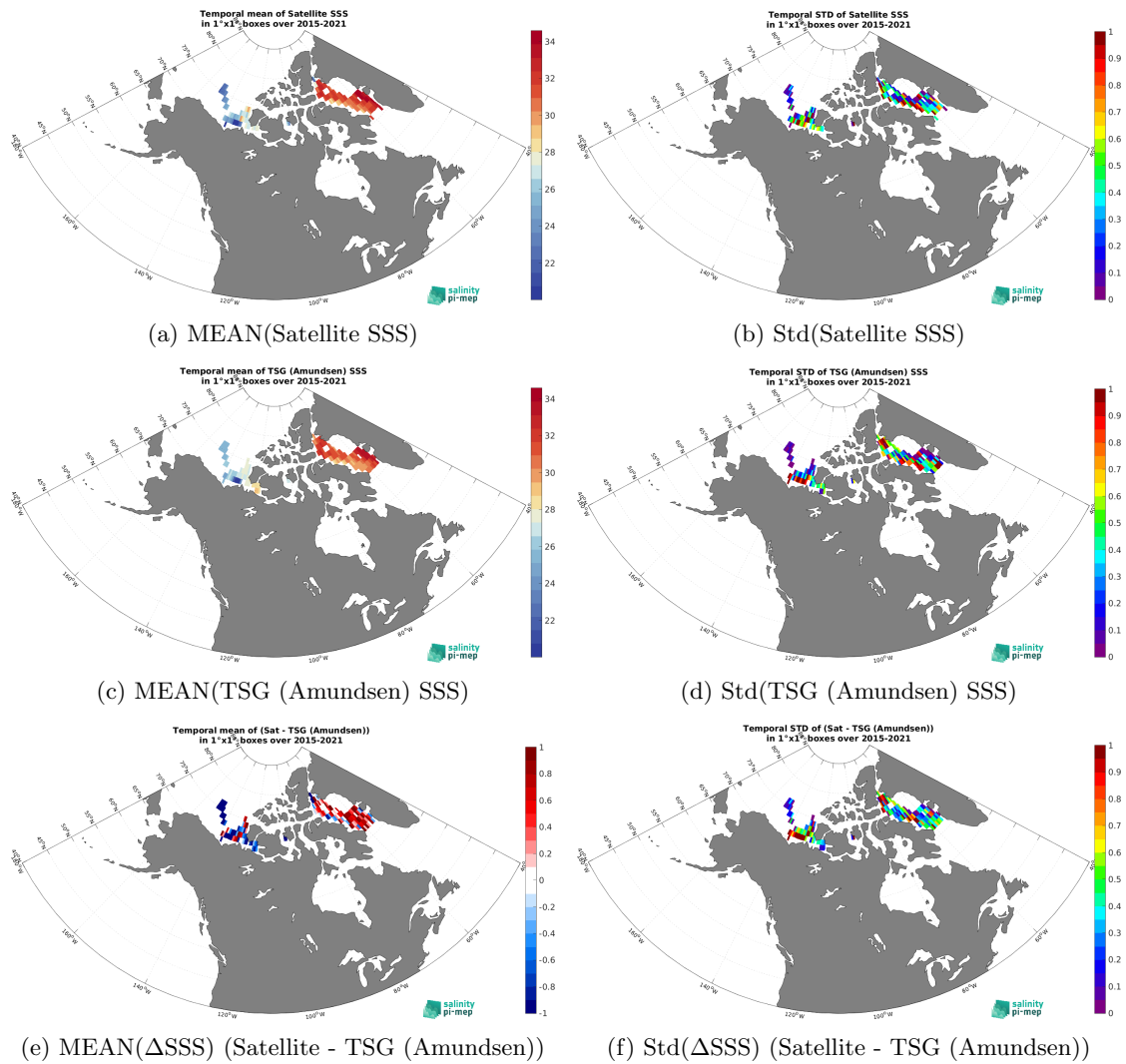
Figure 7: Temporal mean (left) and Std (right) of SSS from SMAP SSS L3 v6 - 8-Day running (RSS) (top), TSG (Amundsen) (middle), and of \Delta SSS (Satellite - TSG (Amundsen)). Only match-up pairs are used to generate these maps.
