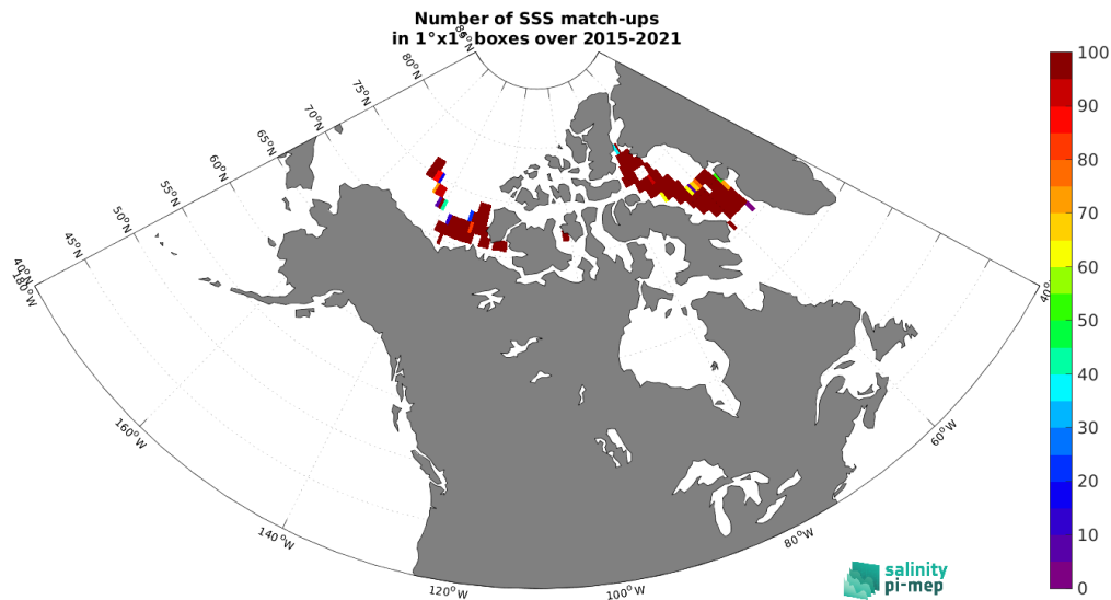
Figure 5: Number of SSS match-ups between TSG (Amundsen) SSS and the SMAP SSS L3 v6 - 8-Day running (RSS) SSS product for the Arctic Ocean Pi-MEP region over 1^\circ \times 1^\circ boxes and for the full satellite product period.
