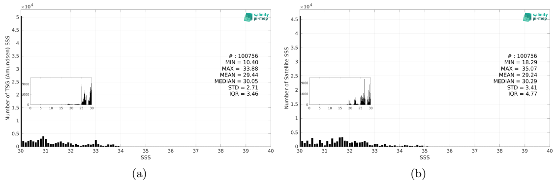
Figure 3: Histograms of SSS from TSG (Amundsen) (a) and SMAP SSS L3 v6 - 8-Day running (RSS) (b) considering all match-up pairs per bins of 0.1 over the Arctic Ocean Pi-MEP region and for the full satellite product period.
