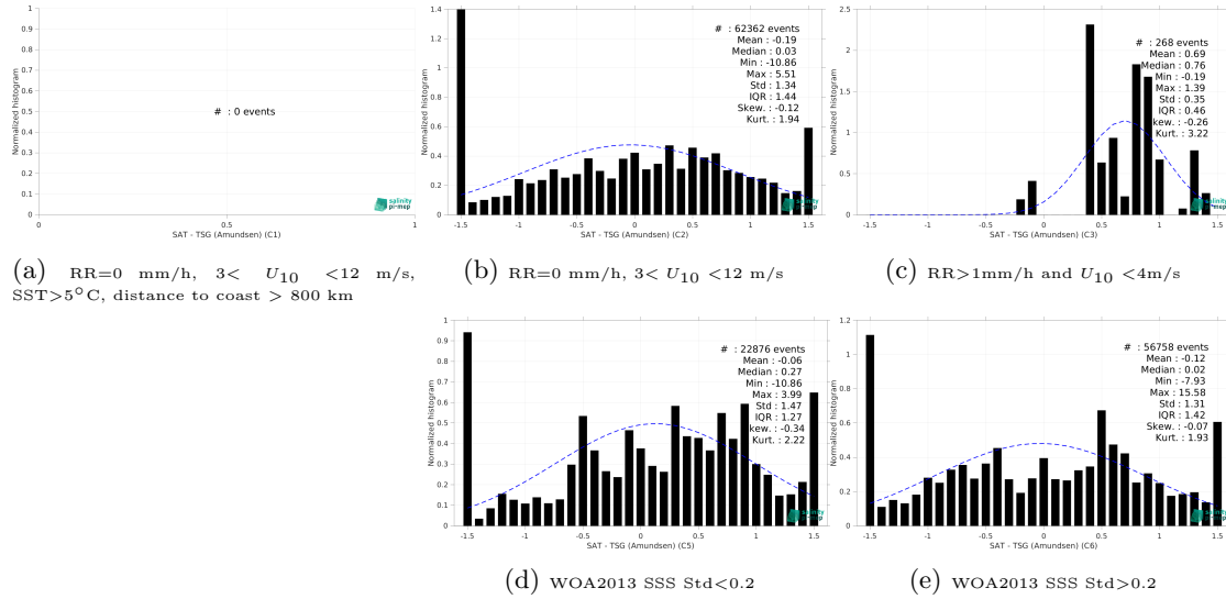
Figure 15: Normalized histogram of \Delta SSS (SMAP SSS L3 v6 - 8-Day running (RSS) - TSG (Amundsen)) for 5 different subdatasets corresponding to: RR=0 mm/h, 3 < U_{10} < 12 m/s, SST>5°C, distance to coast > 800 km (a), RR=0 mm/h, 3 < U_{10} < 12 m/s (b), RR>1mm/h and U_{10} < 4 m/s (c), WOA2013 SSS Std<0.2 (d), WOA2013 SSS Std>0.2 (e).
