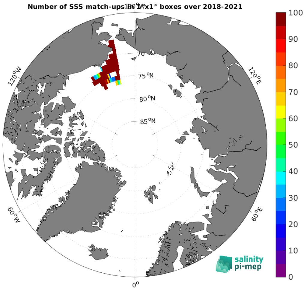
Figure 5: Number of SSS match-ups between Saildrone SSS and the SMAP SSS L3 v6 - 8-Day running (RSS) SSS product for the Arctic Ocean Pi-MEP region over 1^\circ \times 1^\circ boxes and for the full satellite product period.
