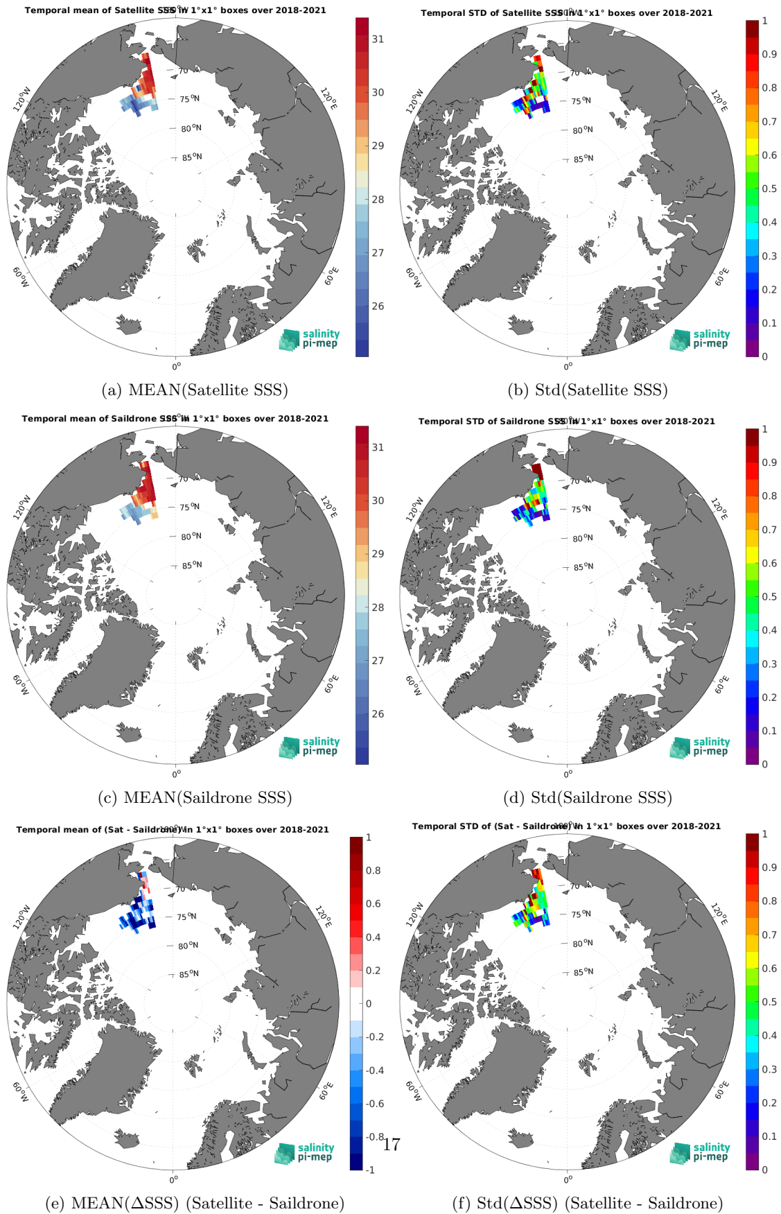
Figure 7: Temporal mean (left) and Std (right) of SSS from SMAP SSS L3 v6 - 8-Day running (RSS) (top), Saildrone (middle), and of \Delta SSS (Satellite - Saildrone). Only match-up pairs are used to generate these maps.
