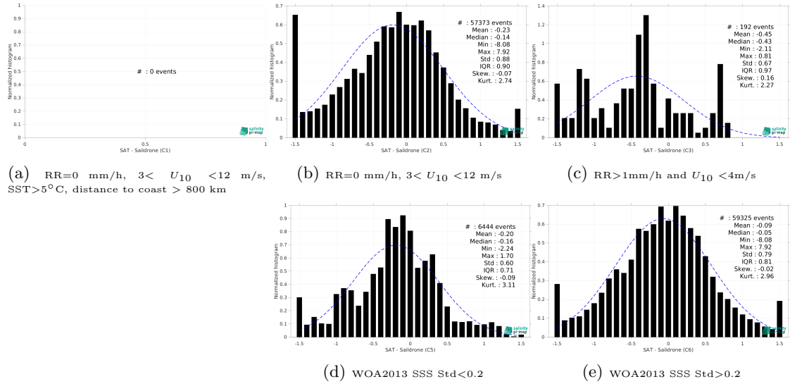
Figure 15: Normalized histogram of \Delta SSS (SMAP SSS L3 v6 - 8-Day running (RSS) - Saldrone) for 5 different subdatasets corresponding to: RR=0 mm/h, 3 < U_{10} < 12 m/s, SST > 5°C, distance to coast > 800 km (a), RR=0 mm/h, 3 < U_{10} < 12 m/s (b), RR > 1mm/h and U_{10} < 4 m/s (c), WOA2013 SSS Std < 0.2 (d), WOA2013 SSS Std > 0.2 (e).
