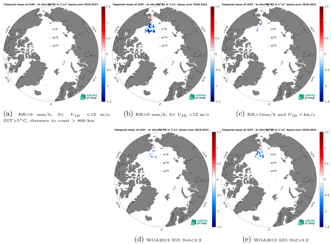
Figure 14: Temporal mean gridded over spatial boxes of size 1^\circ \times 1^\circ of \Delta\text{SSS} (SMAP SSS L3 v6 - 8-Day running (RSS) - Sailability) for 5 different subdatasets corresponding to: RR=0 mm/h, 3 < U_{10} < 12 m/s, SST > 5°C, distance to coast > 800 km (a), RR=0 mm/h, 3 < U_{10} < 12 m/s (b), RR > 1mm/h and U_{10} < 4 m/s (c), WOA2013 SSS Std < 0.2 (d), WOA2013 SSS Std > 0.2 (e).
