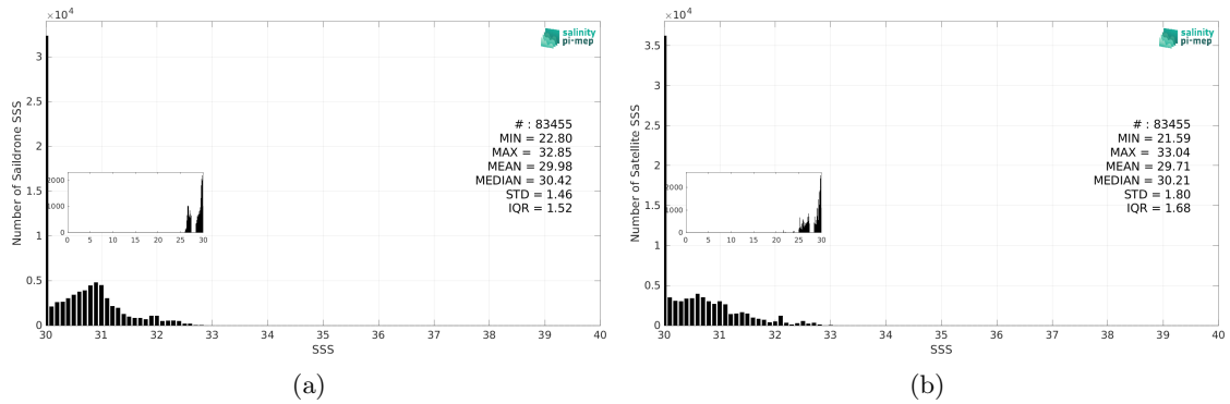
Figure 3: Histograms of SSS from Saildrone (a) and SMAP SSS L3 v6 - 8-Day running (RSS) (b) considering all match-up pairs per bins of 0.1 over the Arctic Ocean Pi-MEP region and for the full satellite product period.
