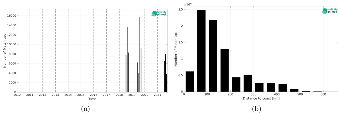
Figure 2: Number of match-ups between Saildrone and SMAP SSS L3 v6 - 8-Day running (RSS) SSS as a function of time (a) and as function of the distance to coast (b) over the Arctic Ocean Pi-MEP region and for the full satellite product period.
