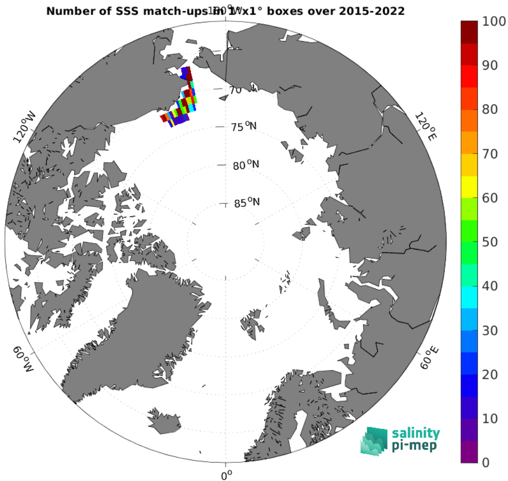
Figure 5: Number of SSS match-ups between TSG (SAMOS) SSS and the SMAP SSS L3 v6 - Monthly (RSS) SSS product for the Arctic Ocean Pi-MEP region over 1^\circ \times 1^\circ boxes and for the full satellite product period.
