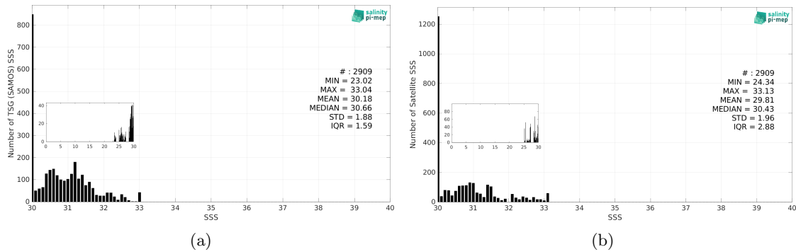
Figure 3: Histograms of SSS from TSG (SAMOS) (a) and SMAP SSS L3 v6 - Monthly (RSS) (b) considering all match-up pairs per bins of 0.1 over the Arctic Ocean Pi-MEP region and for the full satellite product period.
