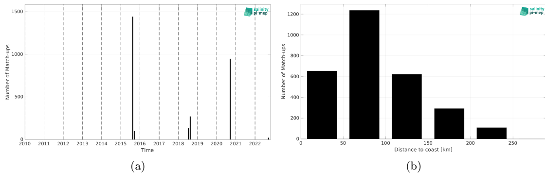
Figure 2: Number of match-ups between TSG (SAMOS) and SMAP SSS L3 v6 - Monthly (RSS) SSS as a function of time (a) and as function of the distance to coast (b) over the Arctic Ocean Pi-MEP region and for the full satellite product period.
