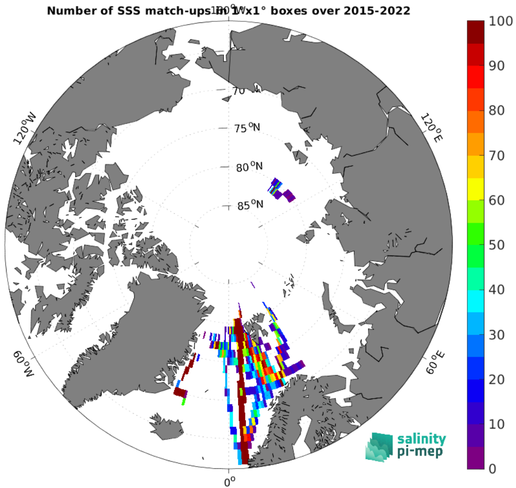
Figure 5: Number of SSS match-ups between TSG (Polarstern) SSS and the SMAP SSS L3 v6 - Monthly (RSS) SSS product for the Arctic Ocean Pi-MEP region over 1^\circ \times 1^\circ boxes and for the full satellite product period.
