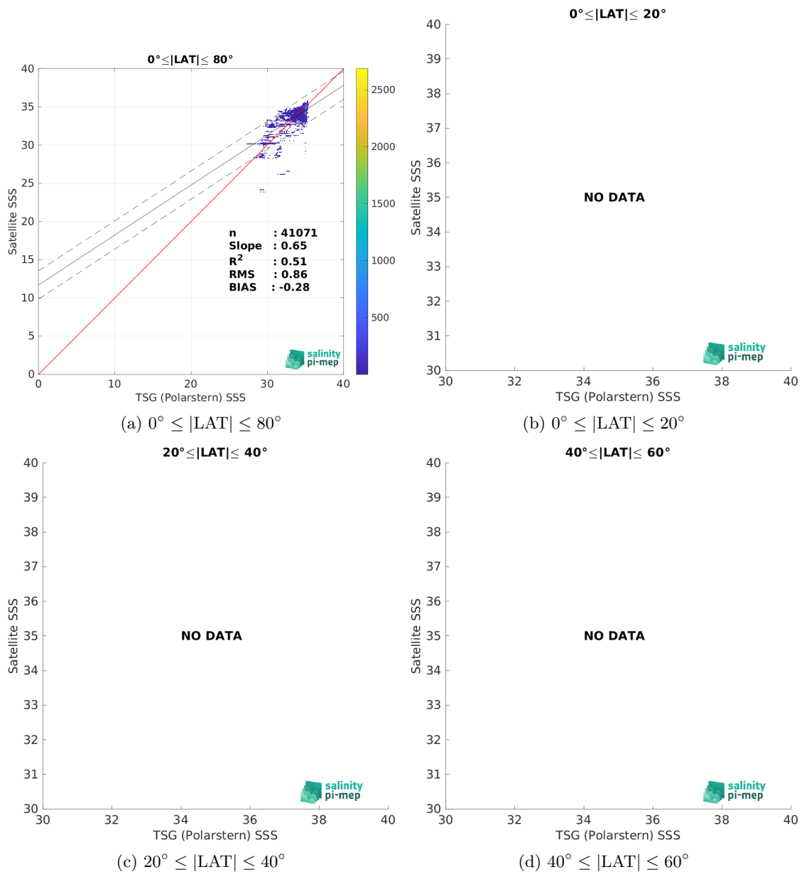
Figure 10: Contour maps of the concentration of SMAP SSS L3 v6 - Monthly (RSS) SSS (y-axis) versus TSG (Polarstern) SSS (x-axis) at match-up pairs for different latitude bands. For each plot, the red line shows x=y . The black thin and dashed lines indicate a linear fit through the data cloud and the \pm 95\% confidence levels, respectively. The number match-up pairs n , the slope and R^2 coefficient of the linear fit, the root mean square (RMS) and the mean bias between satellite and in situ data are indicated for each latitude band in each plots.
