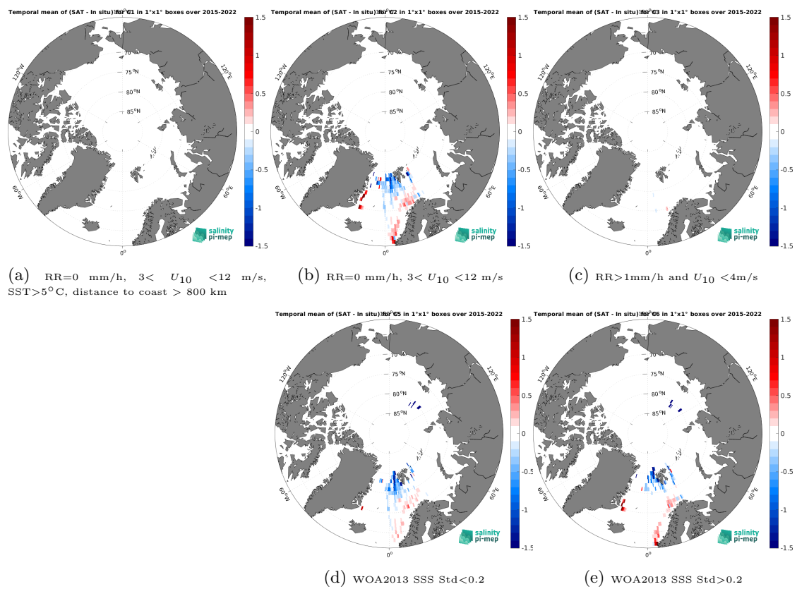
Figure 14: Temporal mean gridded over spatial boxes of size 1^\circ \times 1^\circ of \Delta SSS (SMAP SSS L3 v6 - Monthly (RSS) - TSG (Polarstern)) for 5 different subdatasets corresponding to: RR=0 mm/h, 3 < U_{10} < 12 m/s, SST > 5^\circ\text{C} , distance to coast > 800 km (a), RR=0 mm/h, 3 < U_{10} < 12 m/s (b), RR > 1 mm/h and U_{10} < 4 m/s (c), WOA2013 SSS Std < 0.2 (d), WOA2013 SSS Std > 0.2 (e).
