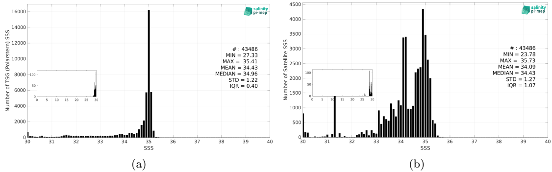
Figure 3: Histograms of SSS from TSG (Polarstern) (a) and SMAP SSS L3 v6 - Monthly (RSS) (b) considering all match-up pairs per bins of 0.1 over the Arctic Ocean Pi-MEP region and for the full satellite product period.
