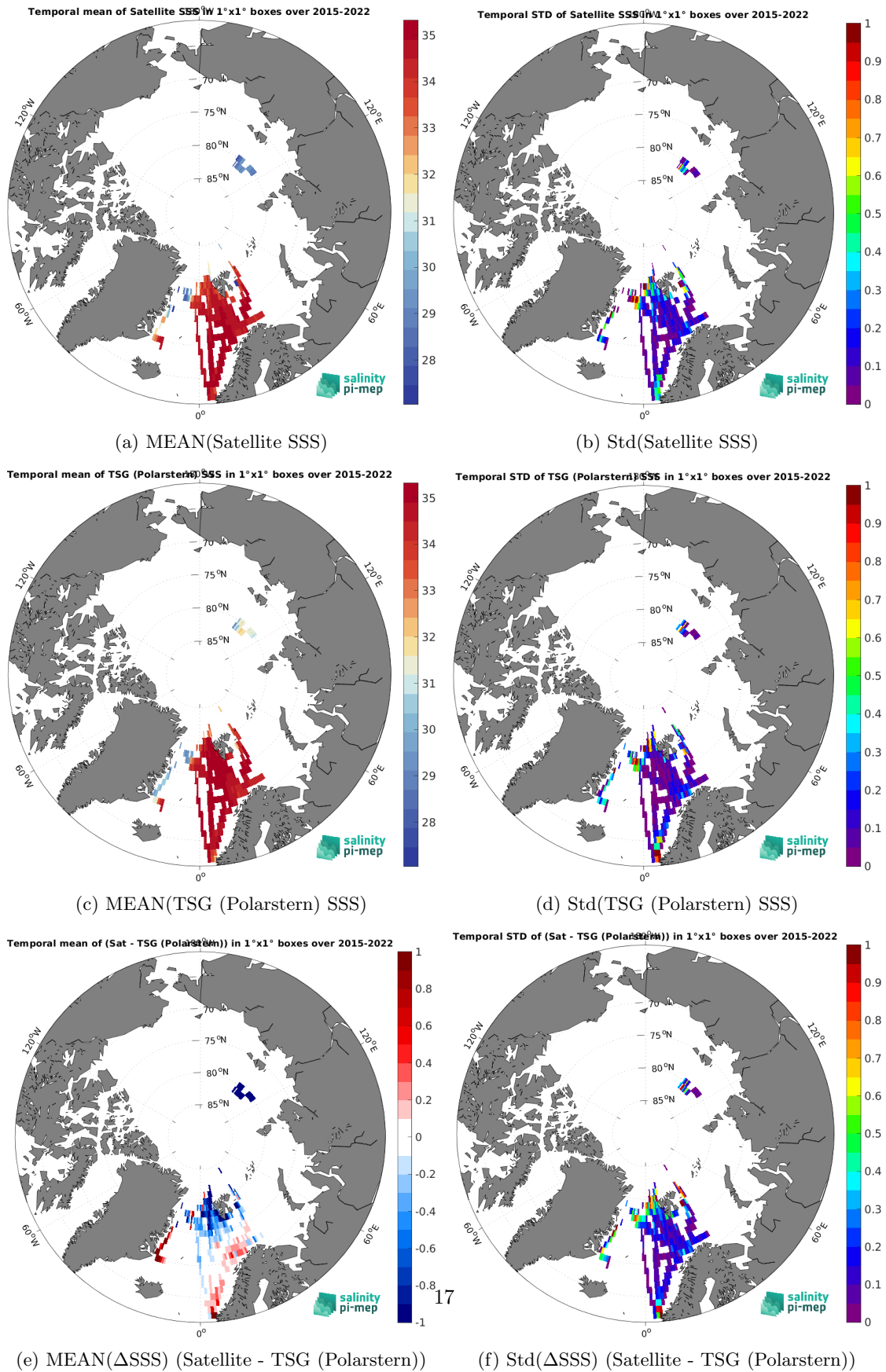
Figure 7: Temporal mean (left) and Std (right) of SSS from SMAP SSS L3 v6 - Monthly (RSS) (top), TSG (Polarstern) (middle), and of \Delta SSS (Satellite - TSG (Polarstern)). Only match-up pairs are used to generate these maps.
