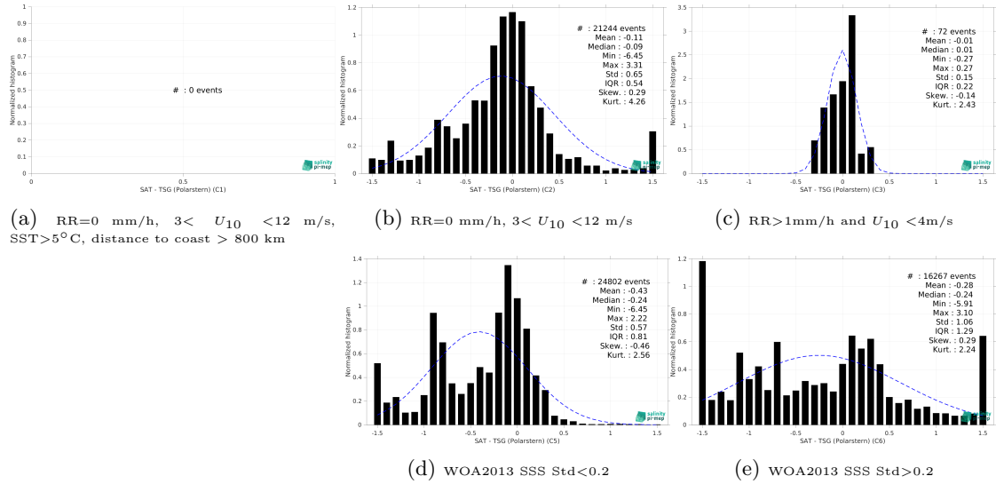
Figure 15: Normalized histogram of \Delta SSS (SMAP SSS L3 v6 - Monthly (RSS) - TSG (Polarstern)) for 5 different subdatasets corresponding to: RR=0 mm/h, 3 < U_{10} < 12 m/s, SST > 5°C, distance to coast > 800 km (a), RR=0 mm/h, 3 < U_{10} < 12 m/s (b), RR > 1mm/h and U_{10} < 4 m/s (c), WOA2013 SSS Std < 0.2 (d), WOA2013 SSS Std > 0.2 (e).
