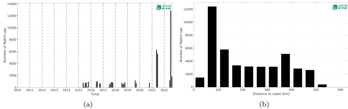
Figure 2: Number of match-ups between TSG (Polarstern) and SMAP SSS L3 v6 - Monthly (RSS) SSS as a function of time (a) and as function of the distance to coast (b) over the Arctic Ocean Pi-MEP region and for the full satellite product period.
