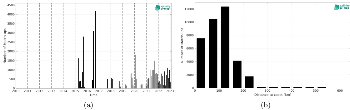
Figure 2: Number of match-ups between TSG (LEGOS-DM) and SMAP SSS L3 v6 - Monthly (RSS) SSS as a function of time (a) and as function of the distance to coast (b) over the Arctic Ocean Pi-MEP region and for the full satellite product period.
