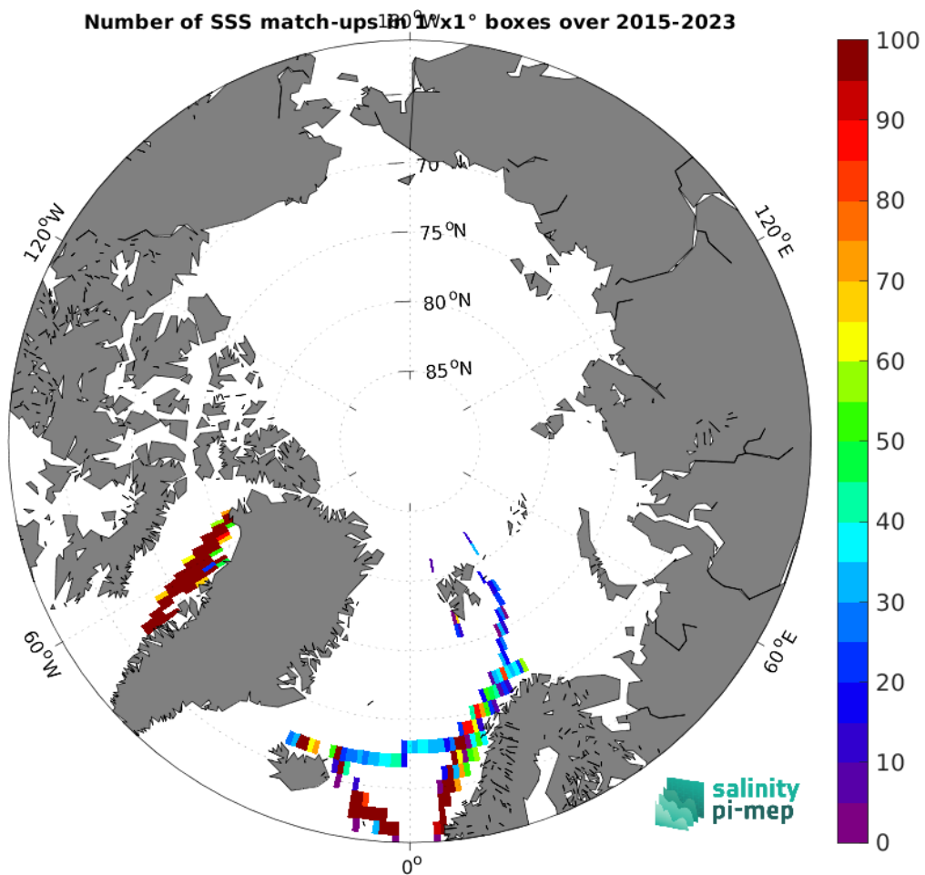
Figure 5: Number of SSS match-ups between TSG (LEGOS-DM) SSS and the SMAP SSS L3 v6 - Monthly (RSS) SSS product for the Arctic Ocean Pi-MEP region over 1^\circ \times 1^\circ boxes and for the full satellite product period.
