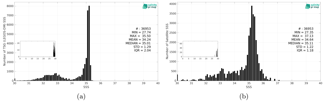
Figure 3: Histograms of SSS from TSG (LEGOS-DM) (a) and SMAP SSS L3 v6 - Monthly (RSS) (b) considering all match-up pairs per bins of 0.1 over the Arctic Ocean Pi-MEP region and for the full satellite product period.
