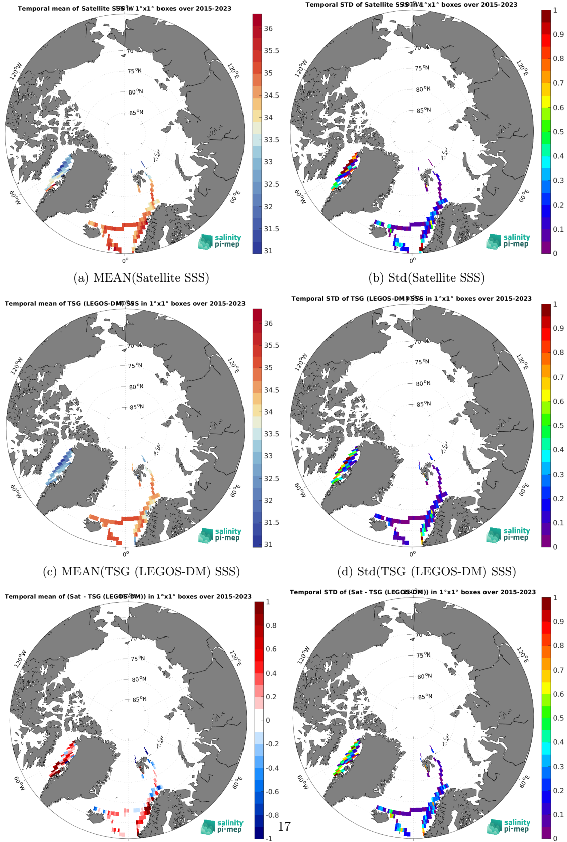
(e) MEAN( \Delta SSS) (Satellite - TSG (LEGOS-DM)) (f) Std( \Delta SSS) (Satellite - TSG (LEGOS-DM)) Figure 7: Temporal mean (left) and Std (right) of SSS from SMAP SSS L3 v6 - Monthly (RSS) (top), TSG (LEGOS-DM) (middle), and of \Delta SSS (Satellite - TSG (LEGOS-DM)). Only match-up pairs are used to generate these maps.
