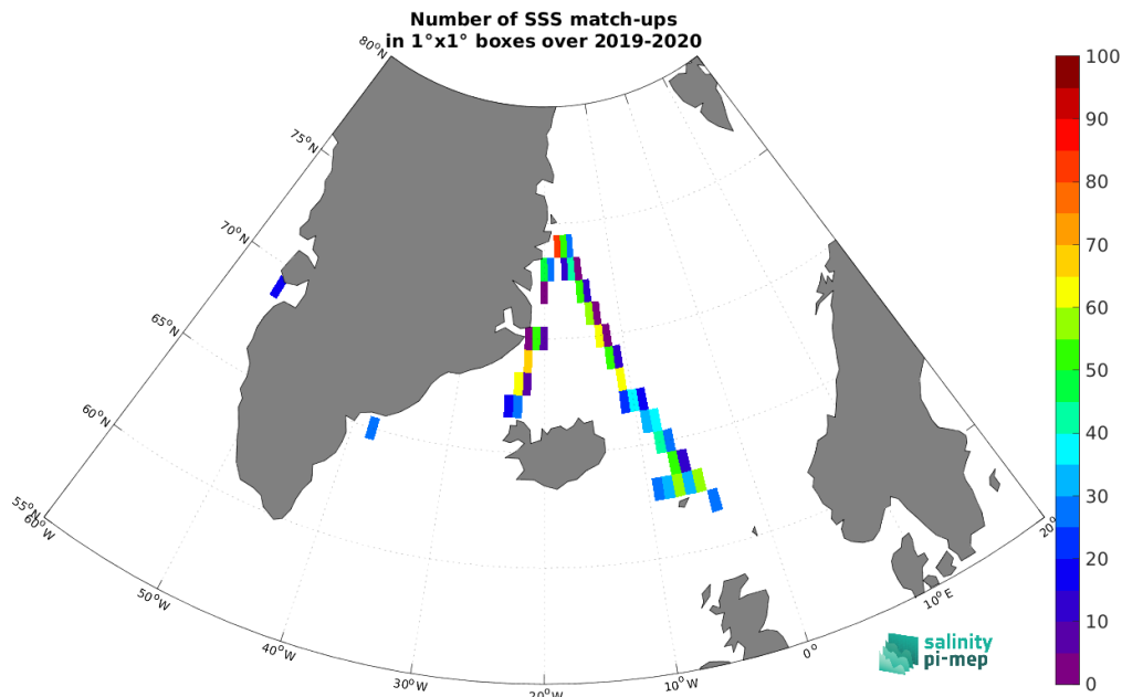
Figure 5: Number of SSS match-ups between TSG (Lauge-Koch) SSS and the SMAP SSS L3 v6 - Monthly (RSS) SSS product for the Arctic Ocean Pi-MEP region over 1^\circ \times 1^\circ boxes and for the full satellite product period.
