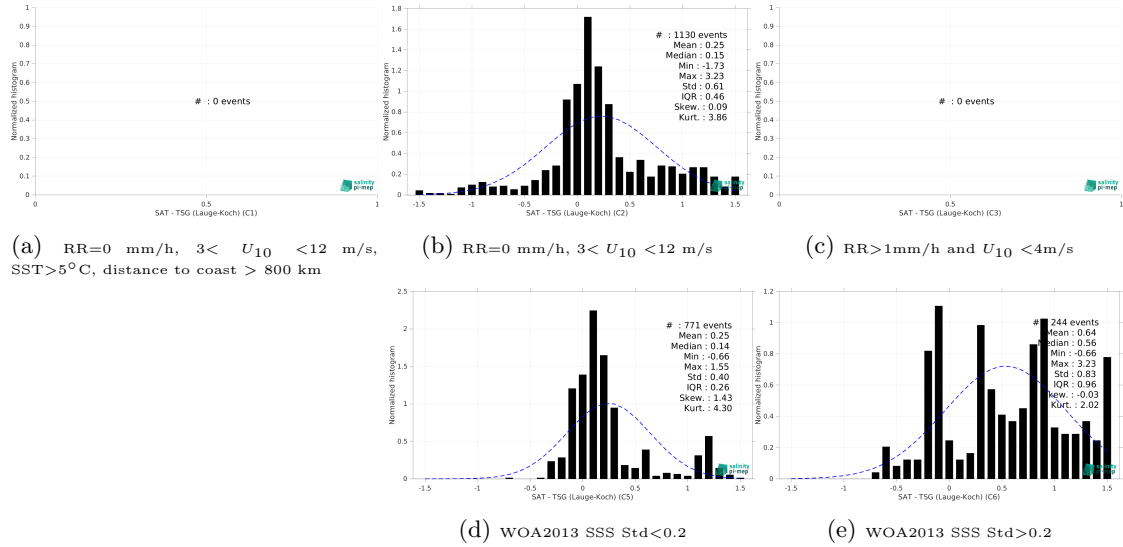
Figure 15: Normalized histogram of \Delta SSS (SMAP SSS L3 v6 - Monthly (RSS) - TSG (Lauge-Koch)) for 5 different subdatasets corresponding to: RR=0 mm/h, 3 < U_{10} < 12 m/s, SST > 5°C, distance to coast > 800 km (a), RR=0 mm/h, 3 < U_{10} < 12 m/s (b), RR > 1mm/h and U_{10} < 4 m/s (c), WOA2013 SSS Std < 0.2 (d), WOA2013 SSS Std > 0.2 (e).
