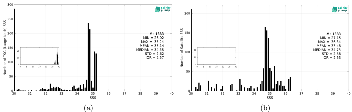
Figure 3: Histograms of SSS from TSG (Lauge-Koch) (a) and SMAP SSS L3 v6 - Monthly (RSS) (b) considering all match-up pairs per bins of 0.1 over the Arctic Ocean Pi-MEP region and for the full satellite product period.
