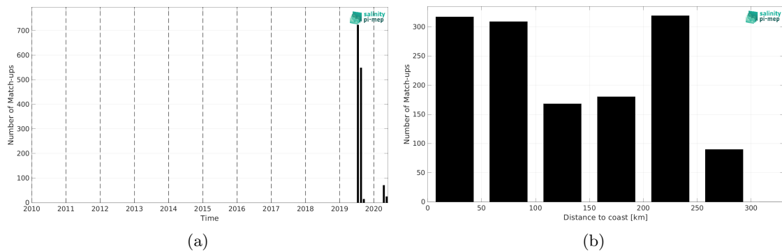
Figure 2: Number of match-ups between TSG (Lauge-Koch) and SMAP SSS L3 v6 - Monthly (RSS) SSS as a function of time (a) and as function of the distance to coast (b) over the Arctic Ocean Pi-MEP region and for the full satellite product period.
