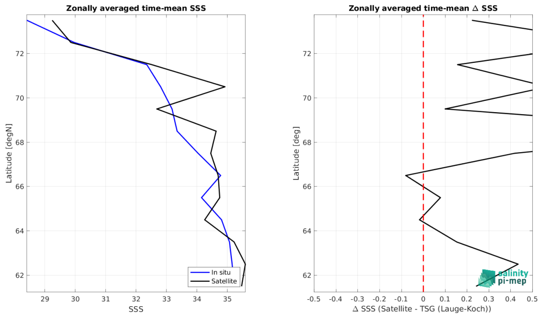
Figure 9: Left panel: Zonal mean SSS from SMAP SSS L3 v6 - Monthly (RSS) satellite product (black) and from TSG (Lauge-Koch) (blue). Right panel: Zonal mean of \Delta SSS (Satellite - TSG (Lauge-Koch)) for all the collected Pi-MEP match-up pairs estimated over the full satellite product period.
