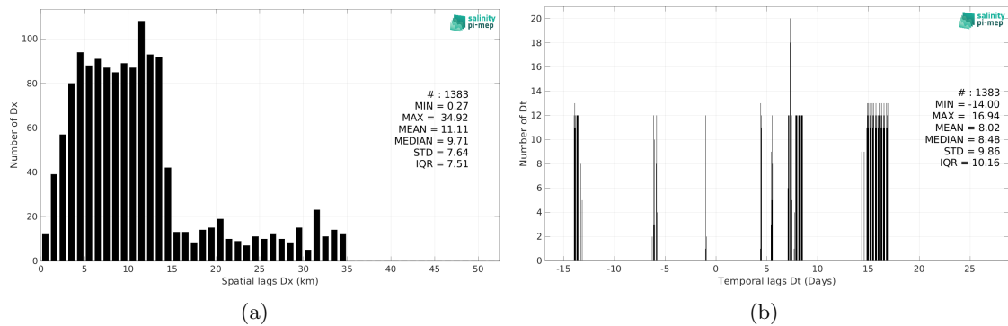
Figure 6: Histograms of the spatial (a) and temporal (b) lags between the location/time of the TSG (Lauge-Koch) measurement and the date of the corresponding SMAP SSS L3 v6 - Monthly (RSS) SSS pixel.
