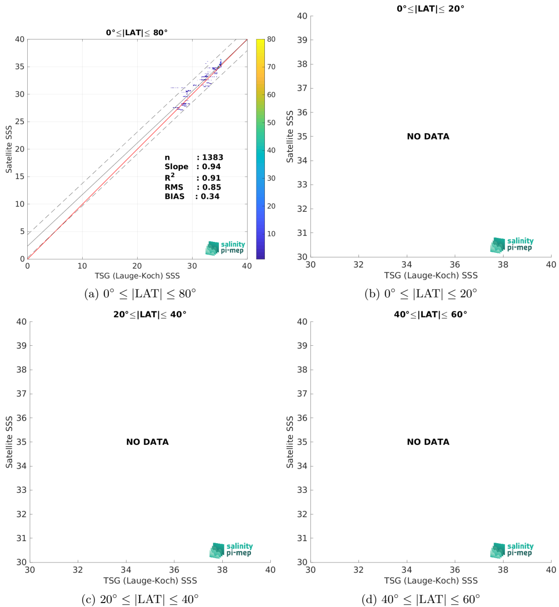
Figure 10: Contour maps of the concentration of SMAP SSS L3 v6 - Monthly (RSS) SSS (y-axis) versus TSG (Lauge-Koch) SSS (x-axis) at match-up pairs for different latitude bands. For each plot, the red line shows x=y . The black thin and dashed lines indicate a linear fit through the data cloud and the \pm 95\% confidence levels, respectively. The number match-up pairs n , the slope and R^2 coefficient of the linear fit, the root mean square (RMS) and the mean bias between satellite and in situ data are indicated for each latitude band in each plots.
