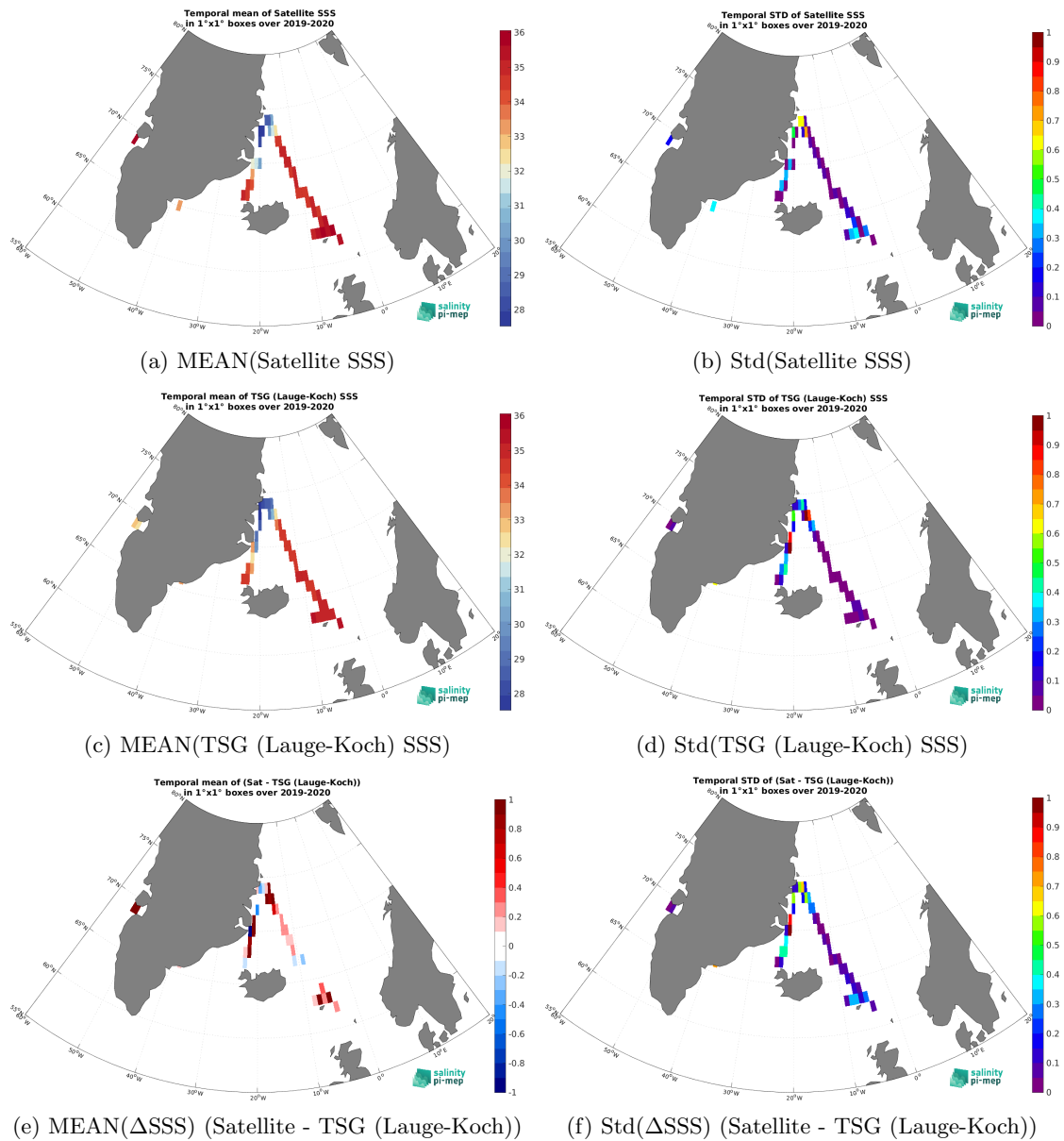
Figure 7: Temporal mean (left) and Std (right) of SSS from SMAP SSS L3 v6 - Monthly (RSS) (top), TSG (Lauge-Koch) (middle), and of \Delta SSS (Satellite - TSG (Lauge-Koch)). Only match-up pairs are used to generate these maps.
