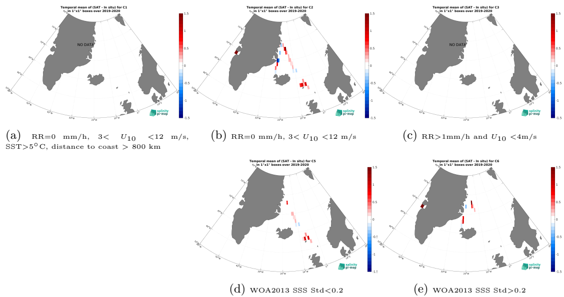
Figure 14: Temporal mean gridded over spatial boxes of size 1^\circ \times 1^\circ of \Delta SSS (SMAP SSS L3 v6 - Monthly (RSS) - TSG (Lauge-Koch)) for 5 different subdatasets corresponding to:RR=0 mm/h, 3 < U_{10} < 12 m/s, SST > 5^\circ\text{C} , distance to coast > 800 km (a), RR=0 mm/h, 3 < U_{10} < 12 m/s (b), RR > 1 mm/h and U_{10} < 4 m/s (c), WOA2013 SSS Std < 0.2 (d), WOA2013 SSS Std > 0.2 (e).
