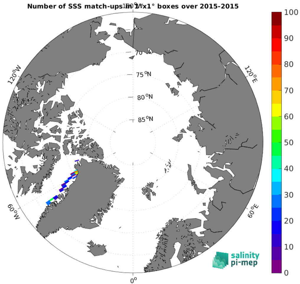
Figure 5: Number of SSS match-ups between TSG (GOSUD-Sailing-ship) SSS and the SMAP SSS L3 v6 - Monthly (RSS) SSS product for the Arctic Ocean Pi-MEP region over 1^\circ \times 1^\circ boxes and for the full satellite product period.
