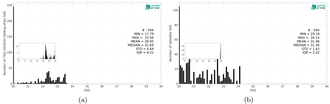
Figure 3: Histograms of SSS from TSG (GOSUD-Sailing-ship) (a) and SMAP SSS L3 v6 - Monthly (RSS) (b) considering all match-up pairs per bins of 0.1 over the Arctic Ocean Pi-MEP region and for the full satellite product period.
