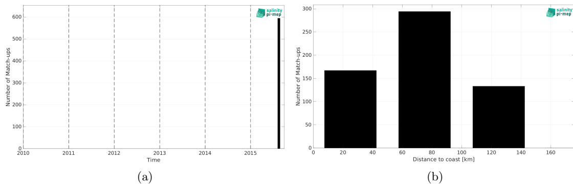
Figure 2: Number of match-ups between TSG (GOSUD-Sailing-ship) and SMAP SSS L3 v6 - Monthly (RSS) SSS as a function of time (a) and as function of the distance to coast (b) over the Arctic Ocean Pi-MEP region and for the full satellite product period.
