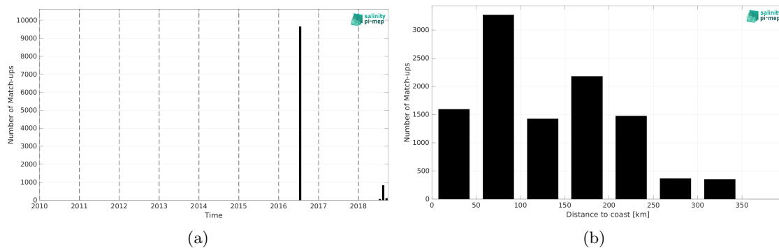
Figure 2: Number of match-ups between TSG (GOSUD-Research-vessel) and SMAP SSS L3 v6 - Monthly (RSS) SSS as a function of time (a) and as function of the distance to coast (b) over the Arctic Ocean Pi-MEP region and for the full satellite product period.
