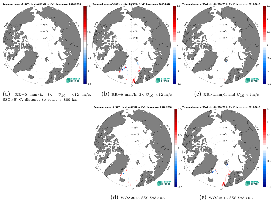
Figure 14: Temporal mean gridded over spatial boxes of size 1^\circ \times 1^\circ of \Delta\text{SSS} (SMAP SSS L3 v6 - Monthly (RSS) - TSG (GOSUD-Research-vessel)) for 5 different subdatasets corresponding to: RR=0 mm/h, 3 < U_{10} < 12 m/s, SST > 5°C, distance to coast > 800 km (a), RR=0 mm/h, 3 < U_{10} < 12 m/s (b), RR > 1mm/h and U_{10} < 4 m/s (c), WOA2013 SSS Std < 0.2 (d), WOA2013 SSS Std > 0.2 (e).
