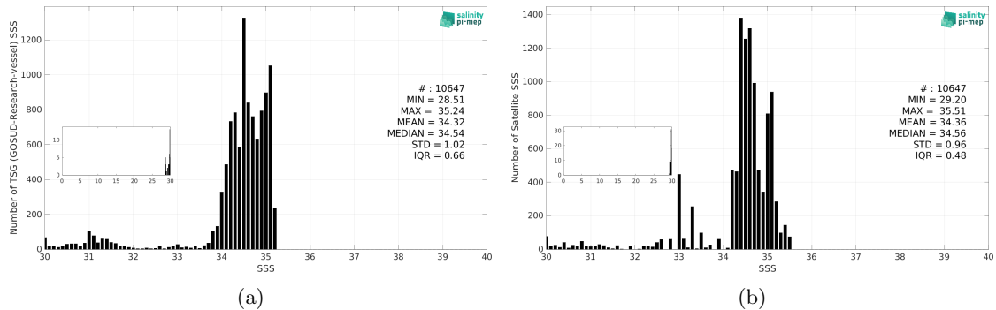
Figure 3: Histograms of SSS from TSG (GOSUD-Research-vessel) (a) and SMAP SSS L3 v6 - Monthly (RSS) (b) considering all match-up pairs per bins of 0.1 over the Arctic Ocean Pi-MEP region and for the full satellite product period.
