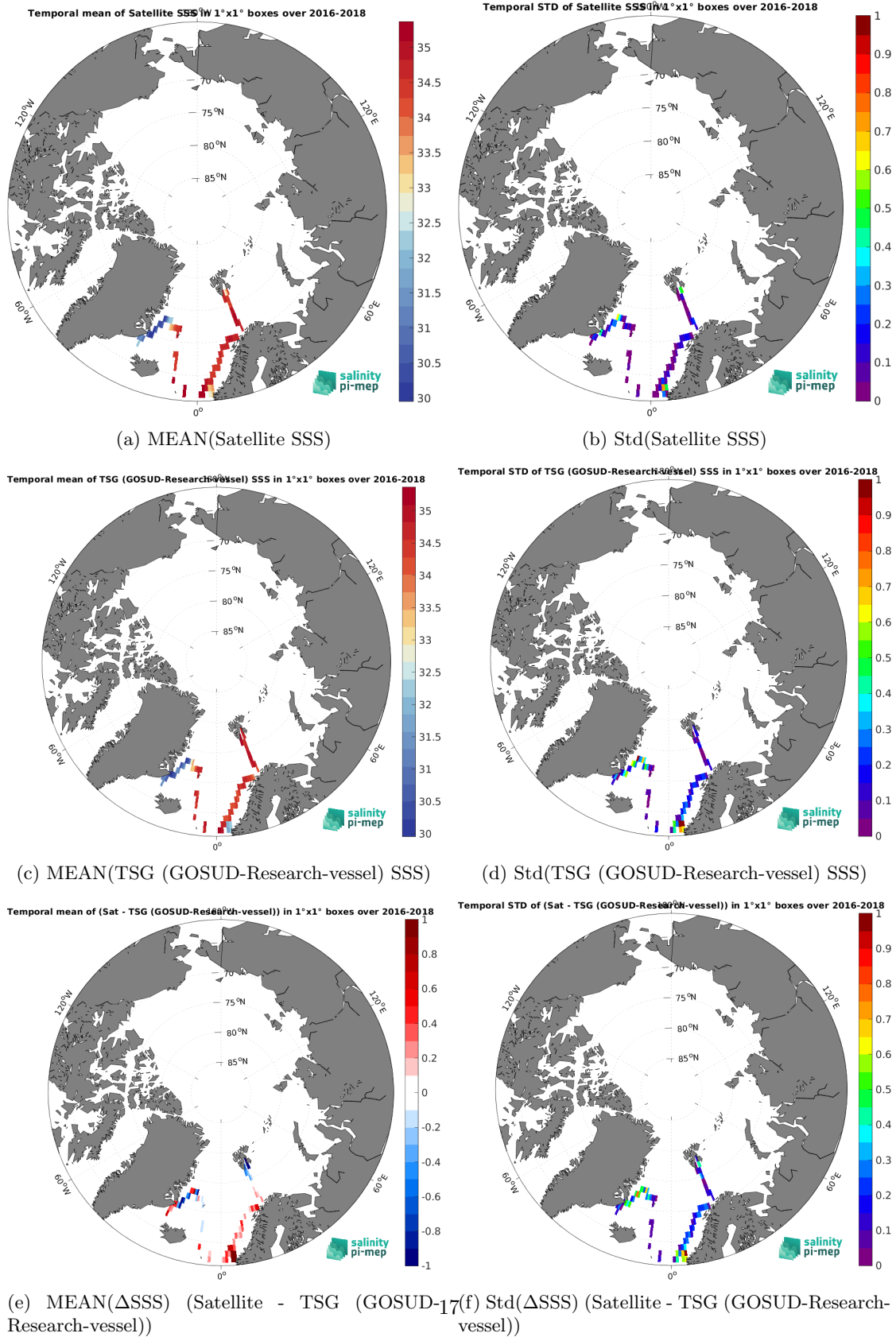
Figure 7: Temporal mean (left) and Std (right) of SSS from SMAP SSS L3 v6 - Monthly (RSS) (top), TSG (GOSUD-Research-vessel) (middle), and of \Delta SSS (Satellite - TSG (GOSUD-Research-vessel)). Only match-up pairs are used to generate these maps.
