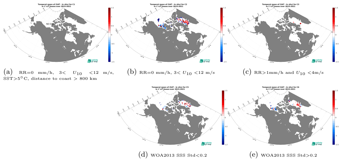
Figure 14: Temporal mean gridded over spatial boxes of size 1^\circ \times 1^\circ of \Delta SSS (SMAP SSS L3 v6 - Monthly (RSS) - TSG (Amundsen)) for 5 different subdatasets corresponding to:RR=0 mm/h, 3 < U_{10} < 12 m/s, SST > 5°C, distance to coast > 800 km (a), RR=0 mm/h, 3 < U_{10} < 12 m/s (b), RR > 1mm/h and U_{10} < 4 m/s (c), WOA2013 SSS Std < 0.2 (d), WOA2013 SSS Std > 0.2 (e).
