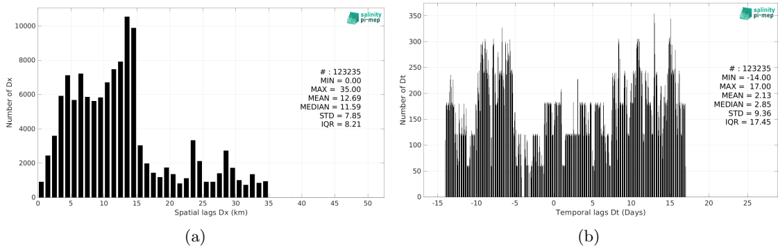
Figure 6: Histograms of the spatial (a) and temporal (b) lags between the location/time of the TSG (Amundsen) measurement and the date of the corresponding SMAP SSS L3 v6 - Monthly (RSS) SSS pixel.
