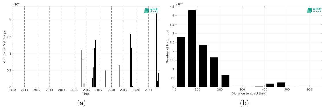
Figure 2: Number of match-ups between TSG (Amundsen) and SMAP SSS L3 v6 - Monthly (RSS) SSS as a function of time (a) and as function of the distance to coast (b) over the Arctic Ocean Pi-MEP region and for the full satellite product period.
