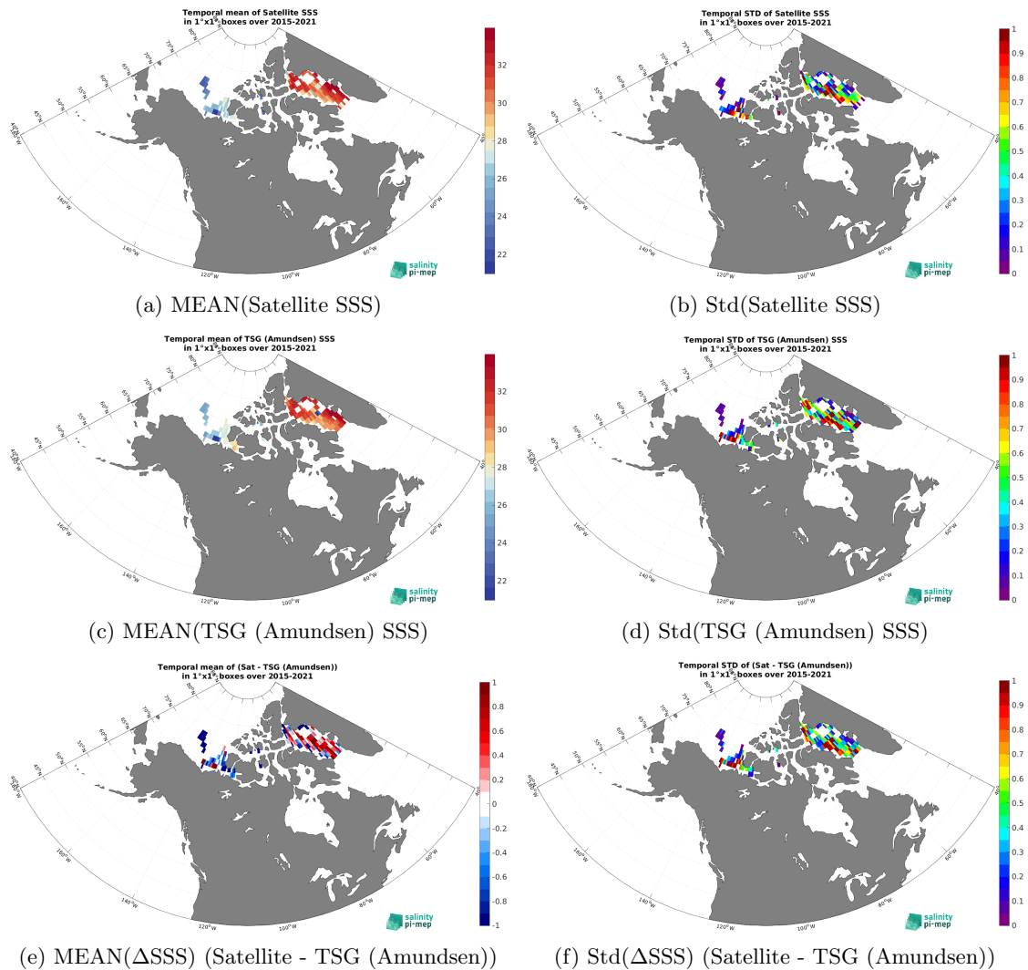
Figure 7: Temporal mean (left) and Std (right) of SSS from SMAP SSS L3 v6 - Monthly (RSS) (top), TSG (Amundsen) (middle), and of \Delta SSS (Satellite - TSG (Amundsen)). Only match-up pairs are used to generate these maps.
