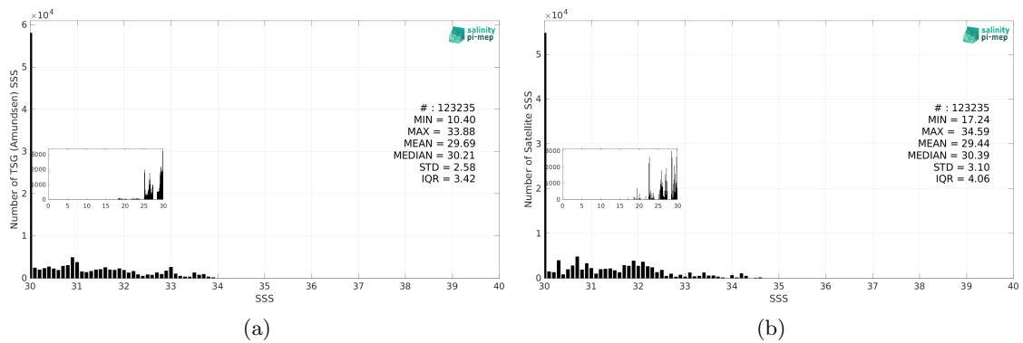
Figure 3: Histograms of SSS from TSG (Amundsen) (a) and SMAP SSS L3 v6 - Monthly (RSS) (b) considering all match-up pairs per bins of 0.1 over the Arctic Ocean Pi-MEP region and for the full satellite product period.
