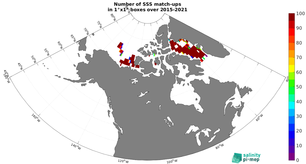
Figure 5: Number of SSS match-ups between TSG (Amundsen) SSS and the SMAP SSS L3 v6 - Monthly (RSS) SSS product for the Arctic Ocean Pi-MEP region over 1^\circ \times 1^\circ boxes and for the full satellite product period.
