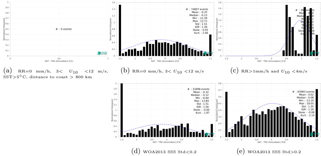
Figure 15: Normalized histogram of \Delta SSS (SMAP SSS L3 v6 - Monthly (RSS) - TSG (Amundsen)) for 5 different subdatasets corresponding to: RR=0 mm/h, 3 < U_{10} < 12 m/s, SST > 5°C, distance to coast > 800 km (a), RR=0 mm/h, 3 < U_{10} < 12 m/s (b), RR > 1mm/h and U_{10} < 4 m/s (c), WOA2013 SSS Std < 0.2 (d), WOA2013 SSS Std > 0.2 (e).
