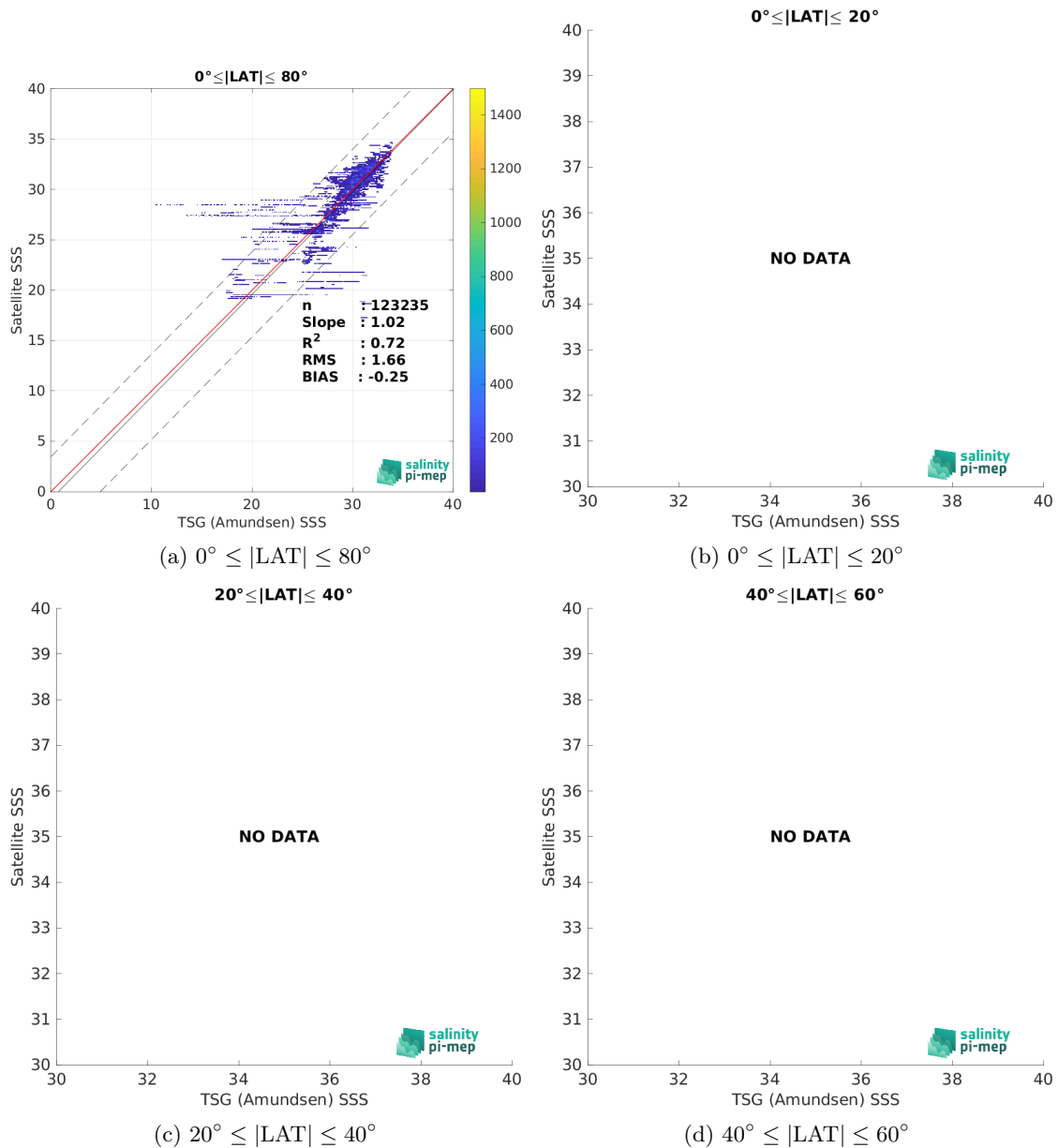
Figure 10: Contour maps of the concentration of SMAP SSS L3 v6 - Monthly (RSS) SSS (y-axis) versus TSG (Amundsen) SSS (x-axis) at match-up pairs for different latitude bands. For each plot, the red line shows x=y . The black thin and dashed lines indicate a linear fit through the data cloud and the \pm 95\% confidence levels, respectively. The number match-up pairs n , the slope and R^2 coefficient of the linear fit, the root mean square (RMS) and the mean bias between satellite and in situ data are indicated for each latitude band in each plots.
