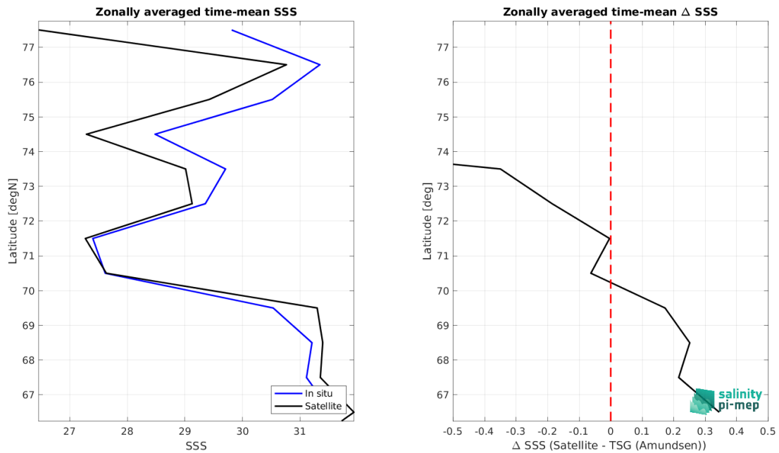
Figure 9: Left panel: Zonal mean SSS from SMAP SSS L3 v6 - Monthly (RSS) satellite product (black) and from TSG (Amundsen) (blue). Right panel: Zonal mean of \Delta SSS (Satellite - TSG (Amundsen)) for all the collected Pi-MEP match-up pairs estimated over the full satellite product period.
