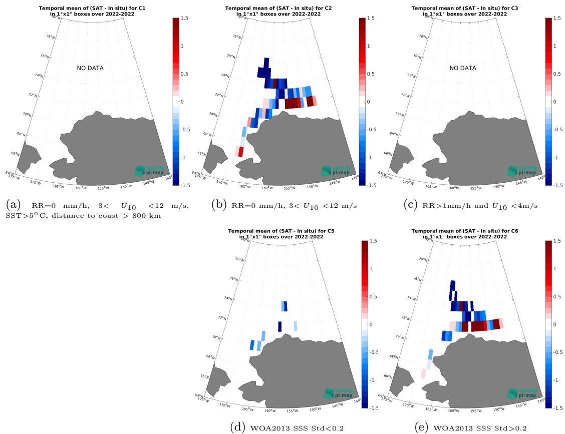
Figure 14: Temporal mean gridded over spatial boxes of size 1^\circ \times 1^\circ of \Delta SSS (SMAP SSS L3 v6 - Monthly (RSS) - SASSIE) for 5 different subdatasets corresponding to:RR=0 mm/h, 3 < U_{10} < 12 m/s, SST >5^\circ\text{C} , distance to coast > 800 km (a), RR=0 mm/h, 3 < U_{10} < 12 m/s (b), RR >1 mm/h and U_{10} < 4 m/s (c), WOA2013 SSS Std <0.2 (d), WOA2013 SSS Std >0.2 (e).
